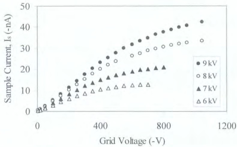
Figure 3.9: A typical set of calibration curves for CCCT varying the needle current, I_s ; 9 kV (4.23 \mu\text{A} ), 8 kV (3.77 \mu\text{A} ), 7 kV (3.15 \mu\text{A} ) and 6 kV (2.61 \mu\text{A} )
