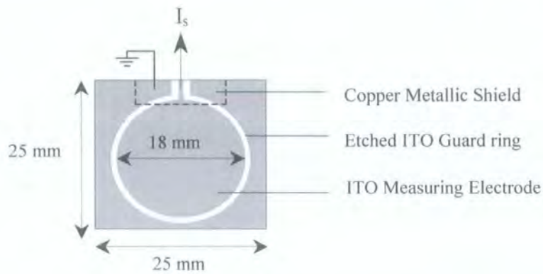
Figure 3.6: Substrate design
