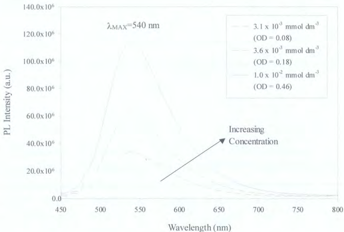
Figure 4.16: Photoluminescence spectra of MORPIP in acetonitrile solution as a function of concentration, \lambda_{ex} = 410 \text{ nm} (absorption peak)
