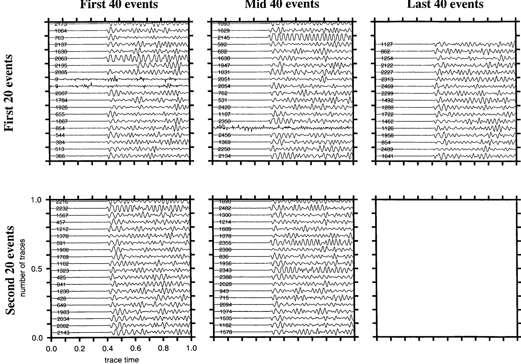
Waveform for events in multiplet sr001_01_95, for station ACR.
