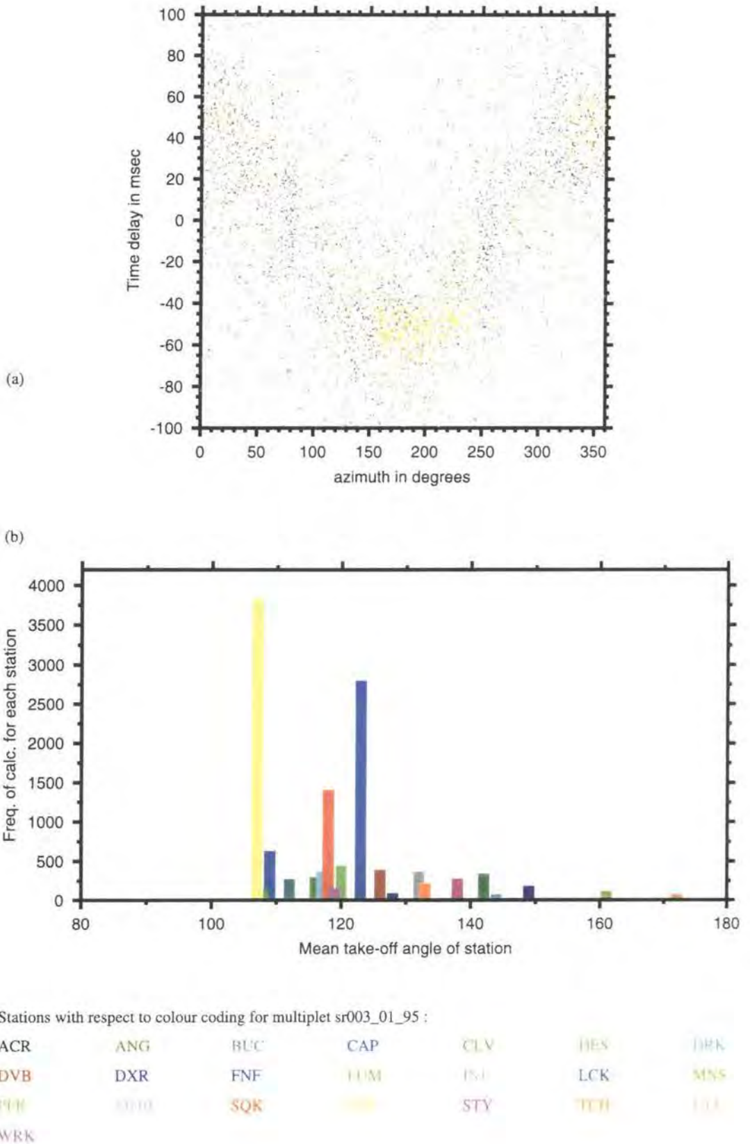
Figure 4.42: As for Figure 4.14 except for multilet sr003_01_95.
