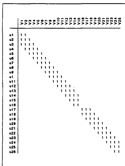
Fig. 7: Matrix of the nearly perfect seriation consisting of two entirely separate sub-sets.
