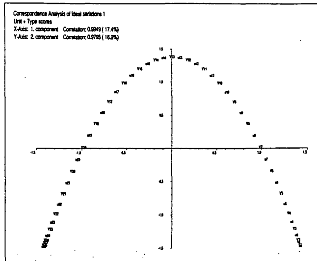
Fig. 6: Scattergram of Correspondence Analysis of the matrix in Fig. 5.
