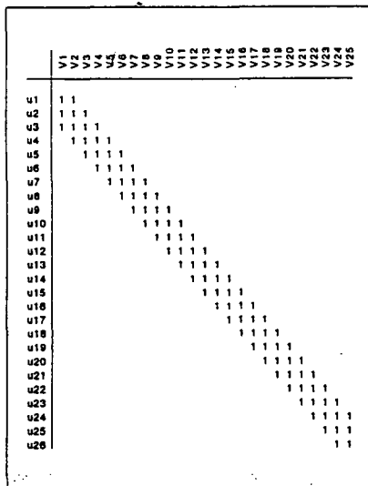
Fig. 5: Matrix of nearly perfect seriation.
