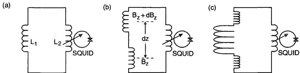
Figure 4.12 – Schematic diagram of three different flux transformers.
