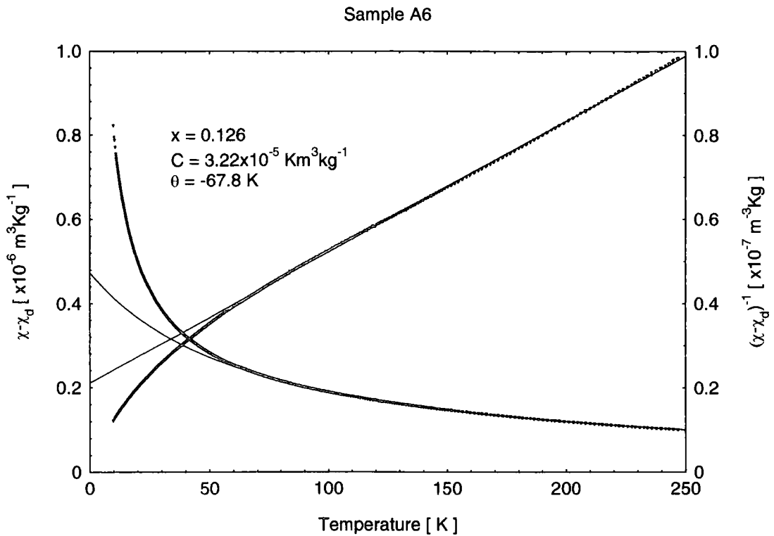
Figure A.3 – Magnetic susceptibility and inverse susceptibility as a function of temperature. For sample A6, x = 0.126 , measuring field B = 50 mT. Plot shows experimental data and fits to Curie-Weiss law used to obtain values for C and \theta .
