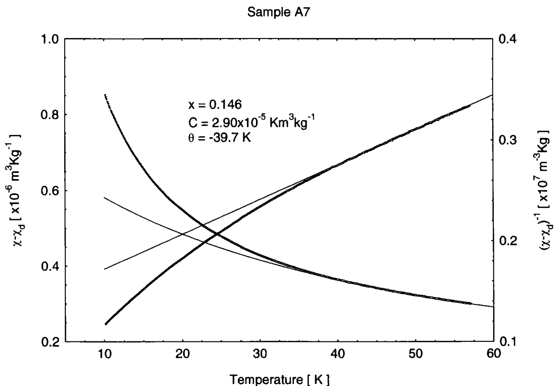
Figure A.4 – Magnetic susceptibility and inverse susceptibility as a function of temperature. For sample A7, x = 0.146 , measuring field B = 50 mT. Plot shows experimental data and fits to Curie-Weiss law used to obtain values for C and \theta .
