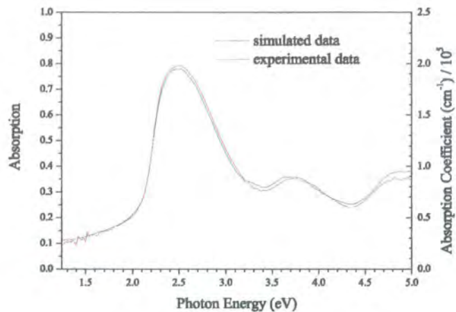
Fig. 4.3: Comparison between simulated absorption data calculated from the ordinary extinction coefficient and the experimental absorption data of MEH-PPV. The simulated data is also shown in units of the absorption coefficient \alpha = 4\pi k/\lambda .
