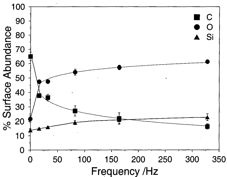
Figure 2.7a Surface elemental abundances of PPSQ oxidized with DBD treatments of varying frequencies.
