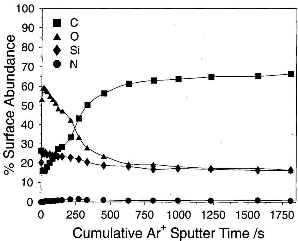
Figure 2.12 Depth profile of DBD oxidized PPSQ.
