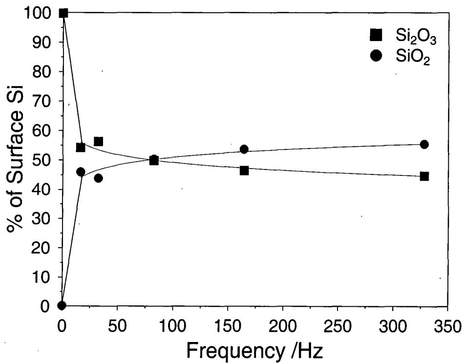
Figure 2.9b Silicon oxidation state distribution of PMSQ oxidized with DBD treatments of varying frequencies.
