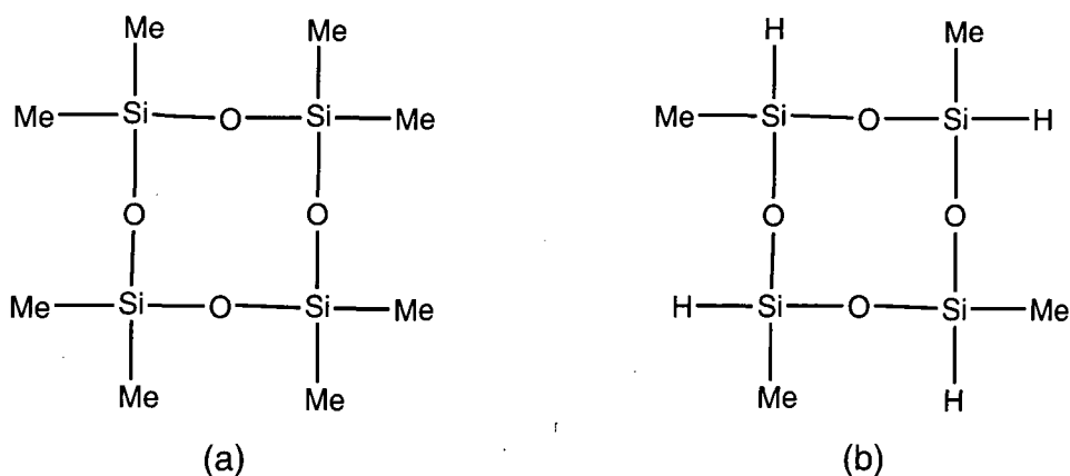
Figure 5.1 The structures of (a) octamethylcyclotetrasiloxane and (b) tetramethylcyclotetrasiloxane.
