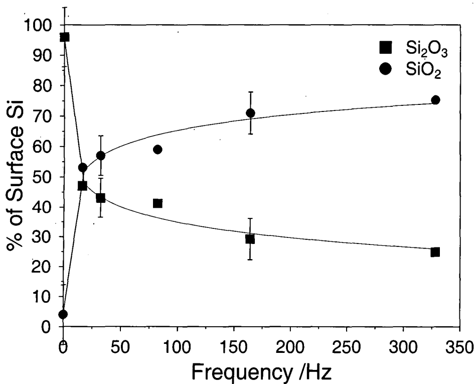
Figure 2.7b Silicon oxidation state distribution of PPSQ oxidized with DBD treatments of varying frequencies.
