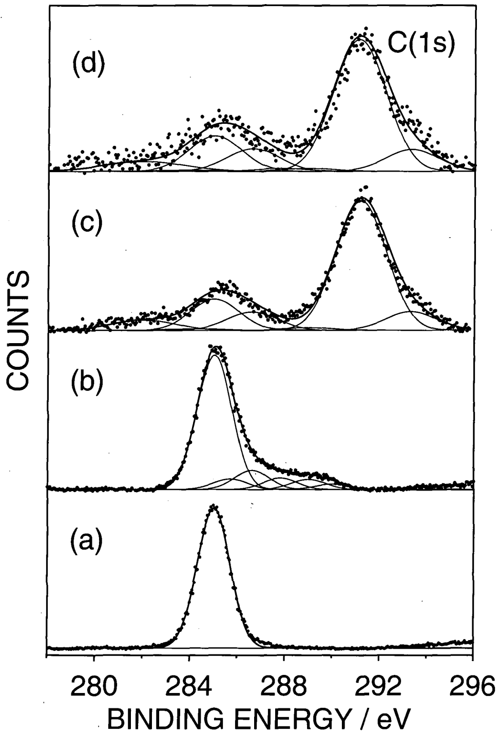
Figure 3.1 C(1s) XPS spectra of (a) clean PE; (b) 10 s silent discharge oxidized polyethylene; (c) 10 s silent discharge oxidized polyethylene exposed to PFDTCS; (d) solvent washed (c).
