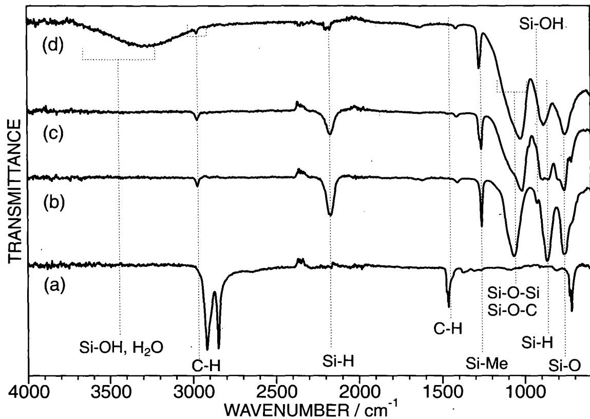
Figure 5.6 ATR-FTIR spectra of (a) polyethylene substrate; (b) TMCTS liquid; (c) helium APGD deposited TMCTS; and (d) helium/oxygen APGD deposited TMCTS.
