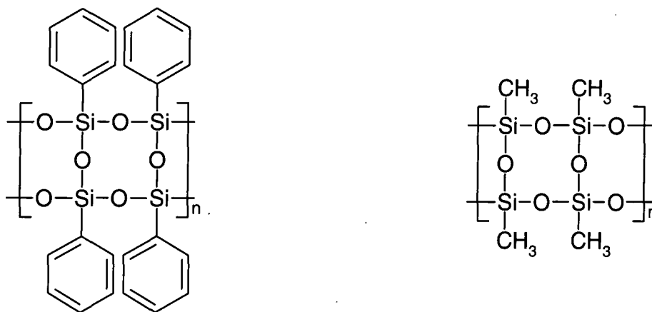
Figure 2.2 Polyphenylsilsesquioxane. Figure 2.3 Polymethylsilsesquioxane.
