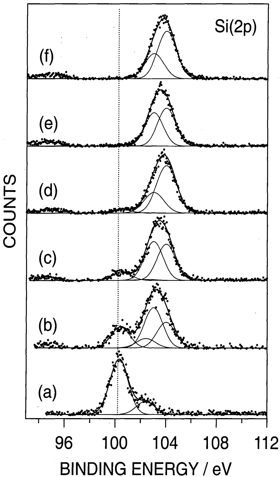
Figure 2.6 Si(2p) XPS spectra of DBD oxidized PCHMS (a) untreated, (b) 16 Hz, (c) 32Hz, (d) 82 Hz, (e) 164 Hz, (f) 328 Hz.
