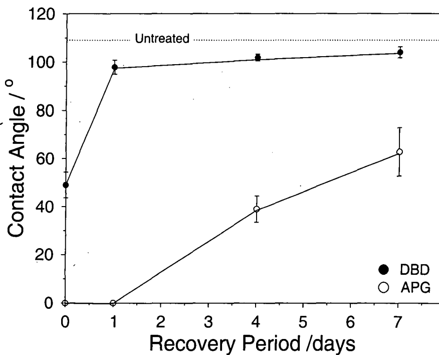
Figure 4.1d Hydrophobic recovery of oxidized ABA/PE blend.
