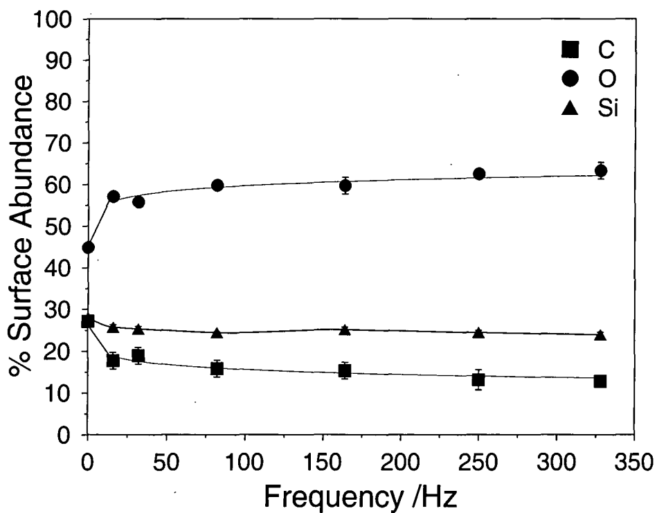
Figure 2.9a Surface elemental abundances of PMSQ oxidized with DBD treatments of varying frequencies.
