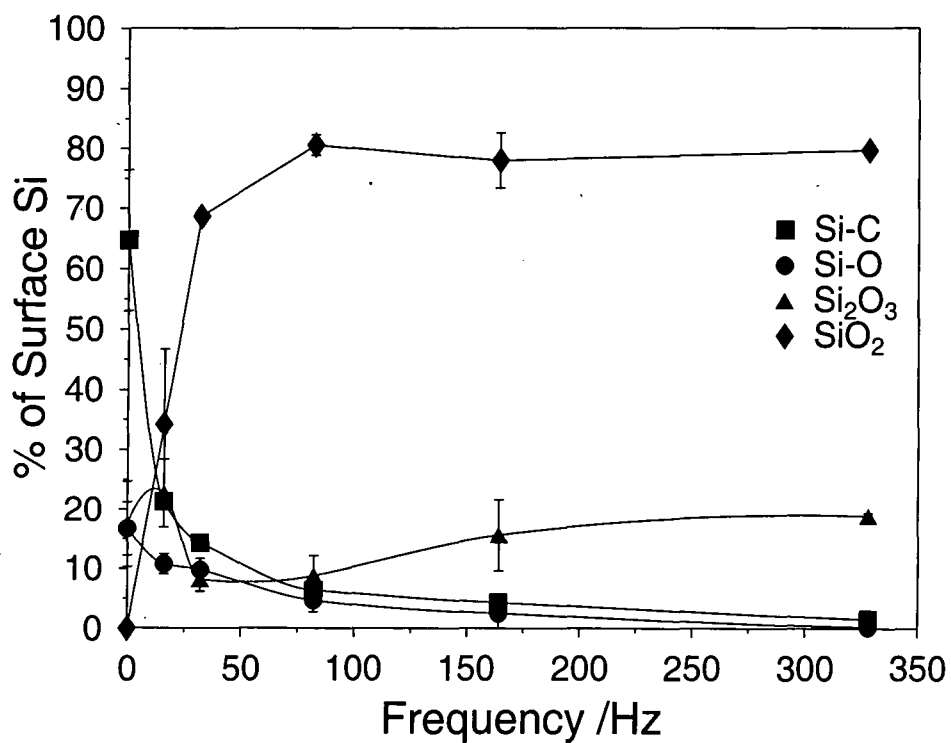
Figure 2.5b Silicon oxidation state distribution of PCHMS oxidized with DBD treatments of varying frequencies.
