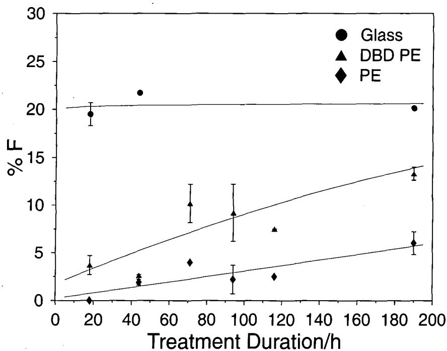
Figure 3.3b PFDMCS labelling onto polyethylene, silent discharge treated polyethylene and glass as a function of exposure time: %F.
