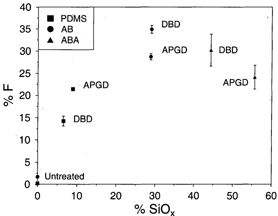
Figure 4.5 The correlation between %SiO x and the degree of PFDMCS attachment (%F) for the plasma oxidized surfaces.
