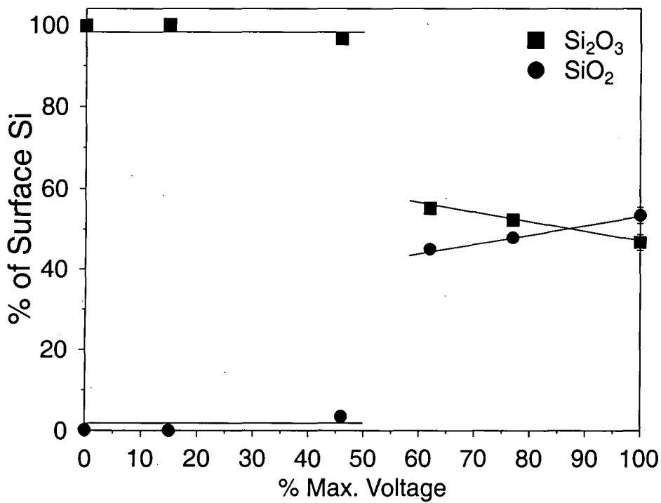
Figure 2.20b The effect of applied voltage upon the silicon oxidation state of DBD treated PMSQ.
