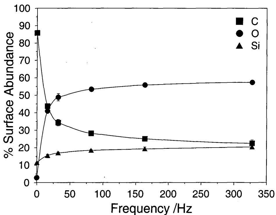
Figure 2.5a Surface elemental abundances of PCHMS oxidized with DBD treatments of varying frequencies.
