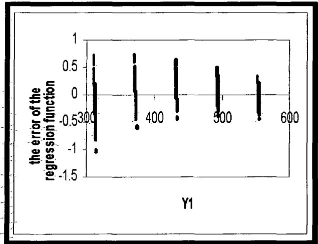
Figure 7-3 The relationship between Y_1 and lm
