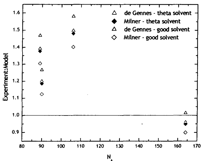
Figure 4.25 - Ratio of experimental brush height to theoretical brush height for cross-linked micelles in both a theta and a good solvent. The horizontal line represents a perfect match between theory and experiment, i.e. Experiment:theory=1.
