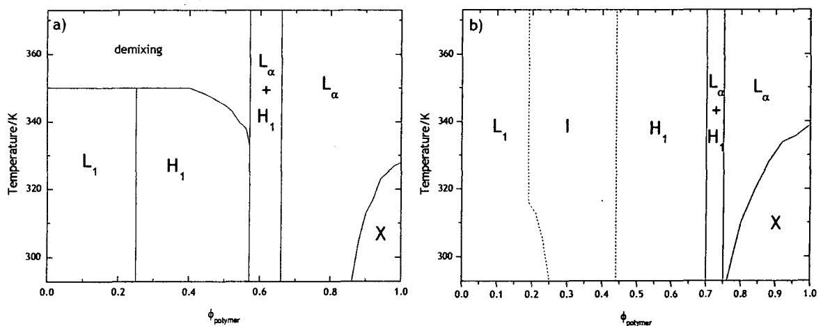
Figure 1.16 - Phase diagrams from Hentze et al. 34 for PB-PEO block copolymers as a function of copolymer concentration and temperature. a) M_n = 13900\text{g mol}^{-1} , w_{PEO} = 0.55 PEO, b) M_n = 28400\text{g mol}^{-1} , w_{PEO} = 0.64 . L_1 -isotropic micellar solution, H_1 -hexagonal phase, L_\alpha - lamellar phase, X-semi-crystalline phase, I-cubic phase
