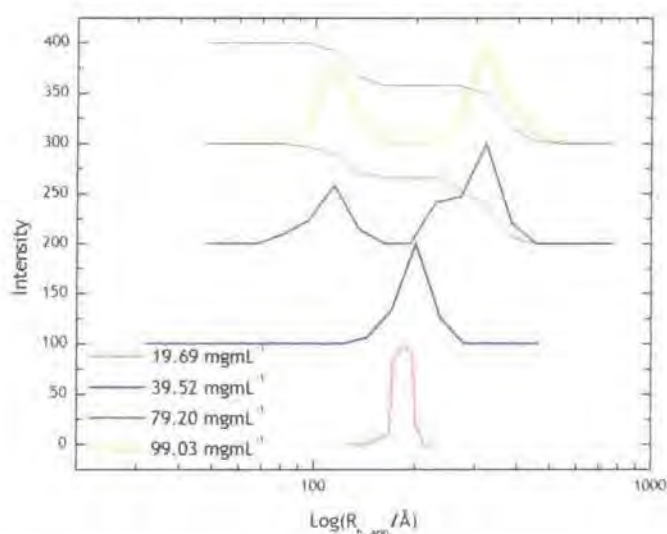
Figure 3.10 - Size distribution for 10k hPB-hPEO at higher concentrations showing the development of dual populations at c > 40 \text{ mg mL}^{-1} . The black lines on the cumulative distributions represent the relative amounts of each present. The distributions are shifted successively by 100 for clarity.
