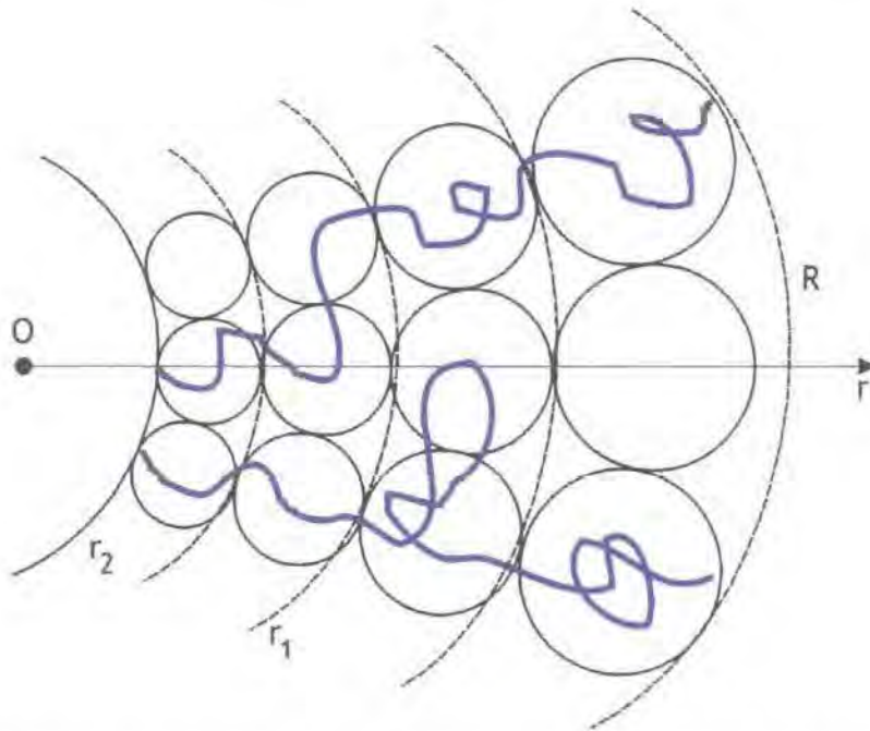
Figure 1.7 - Representation of the blob analogy utilised by Daoud and Cotton
