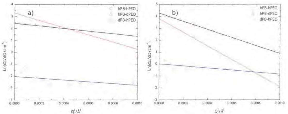
Figure 3.39 - Guinier plots for 1% dispersions of a) 5k and b) 10k generated using equation 3.24. Lines are linear fits to the data
