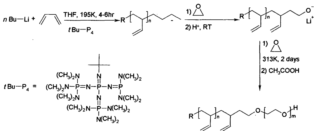
Scheme 2.3- Reaction scheme of Förster and Krämer 11 showing the structure of phosphazene base
