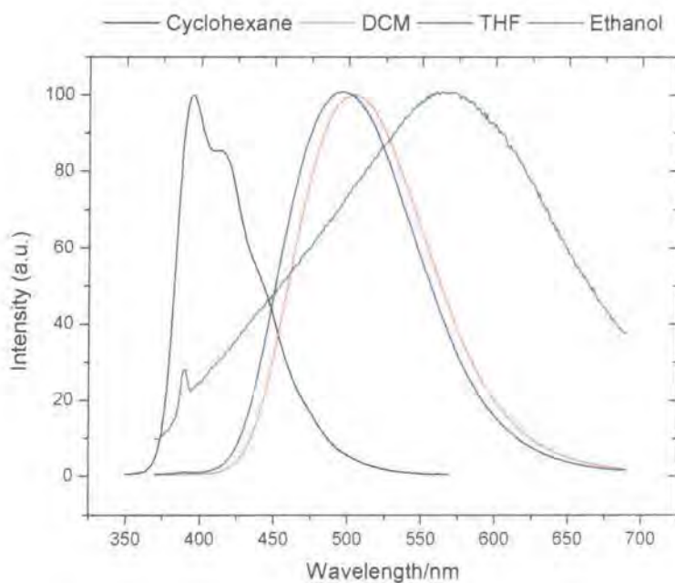
Figure 3.4 – Normalised emission spectrum of L^6 in cyclohexane, THF, DCM and ethanol, \lambda_{\text{exc}}=350\text{nm} . (Corresponding quantum yields are given in table 3.3; note that the compound is much less emissive in ethanol than in the other solvents).
