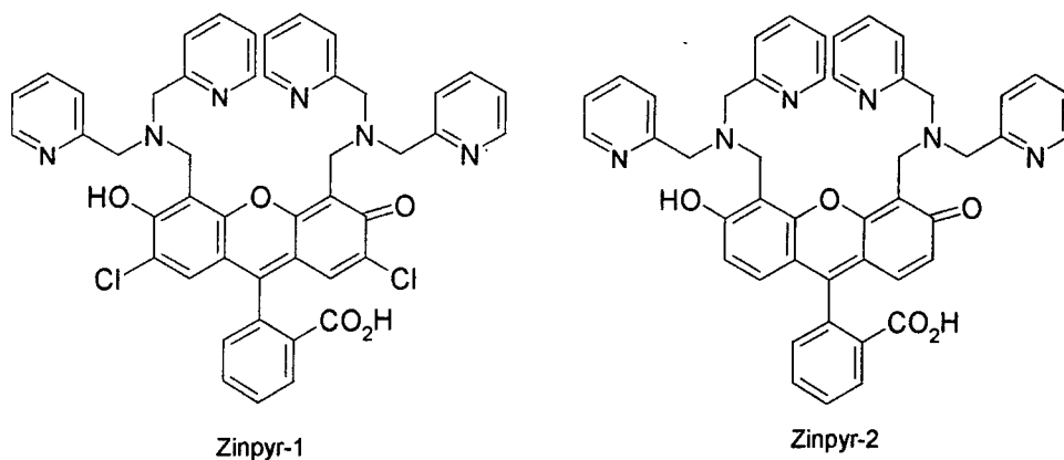
Figure 3.18 - Fluorescein based Zn^{2+} sensors
