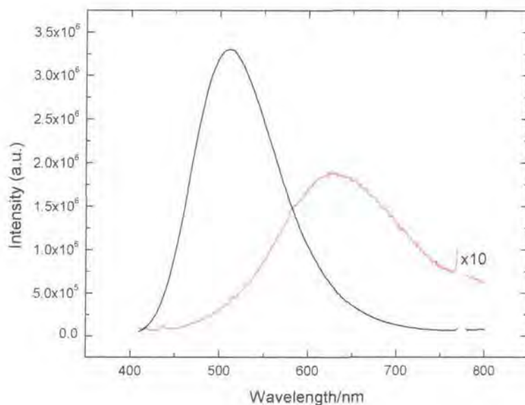
Figure 3.20 - Corrected fluorescence emission spectra of L^- in ethanol (black); and L^- in the presence of Zn^{2+} (red) ( \times 10 ) when excited at the isosbestic point (387 nm)
