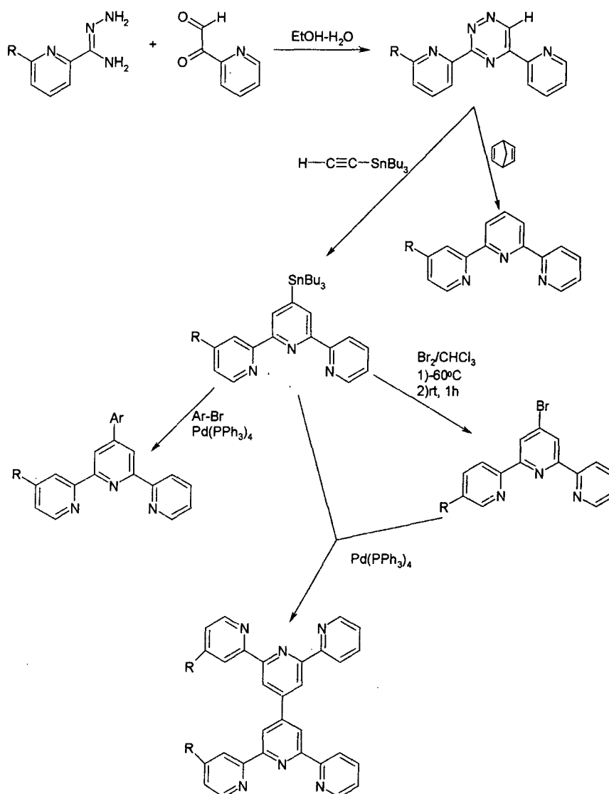
Figure 1.26 - Synthesis of terpyridines using the Sauer methodology 76
