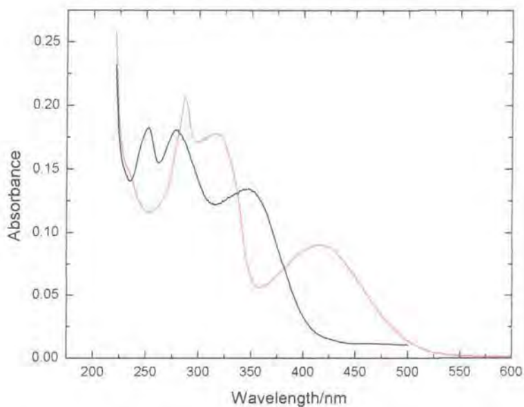
Figure 3.25 - Absorption spectrum of L^{12} in ethanol (black); and L^{12} in the presence of Zn^{2+} (5 equivalents of zinc triflate) (red)
