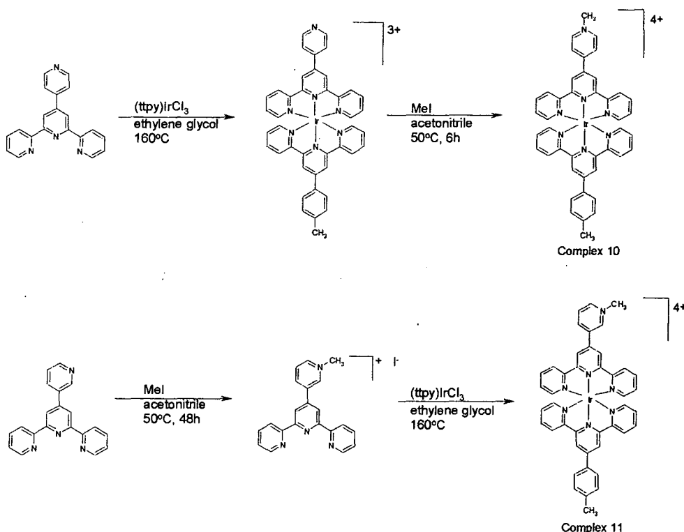
Figure 1.36 - Ir (III) bis(terpyridine) complexes that display Cl - sensitive emission 30
