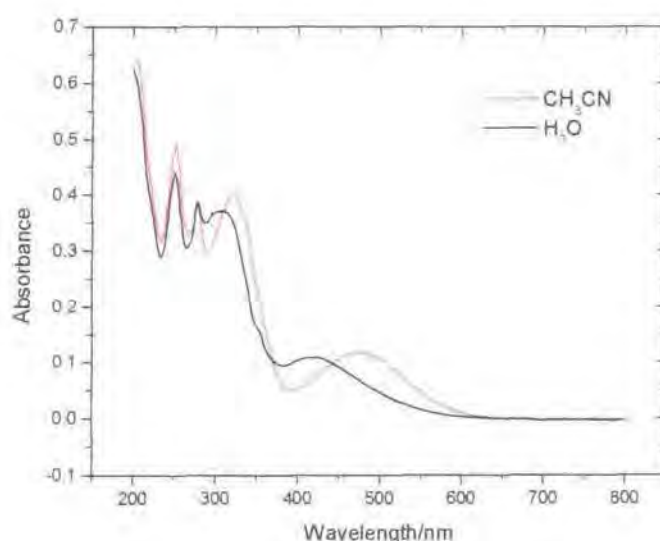
Figure 5.4 – Red-shift observed in the ILCT band of complex 11 on changing solvent from \text{H}_2\text{O} (black) to \text{CH}_3\text{CN} (red).
