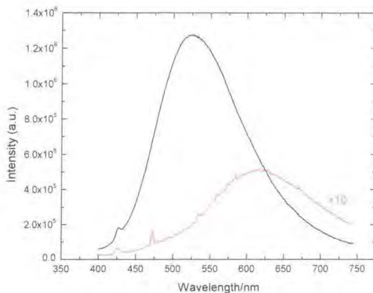
Figure 3.23 - Corrected fluorescence emission spectra of L^6 in ethanol (black); and L^6 in the presence of Zn^{2+} (red) ( \times 10 ) when excited at the isosbestic point (378 nm)
