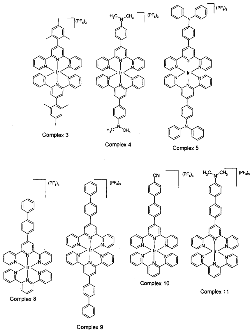
Figure 7.1 – Ir (III) bis(terpyridine) complexes prepared during this work
