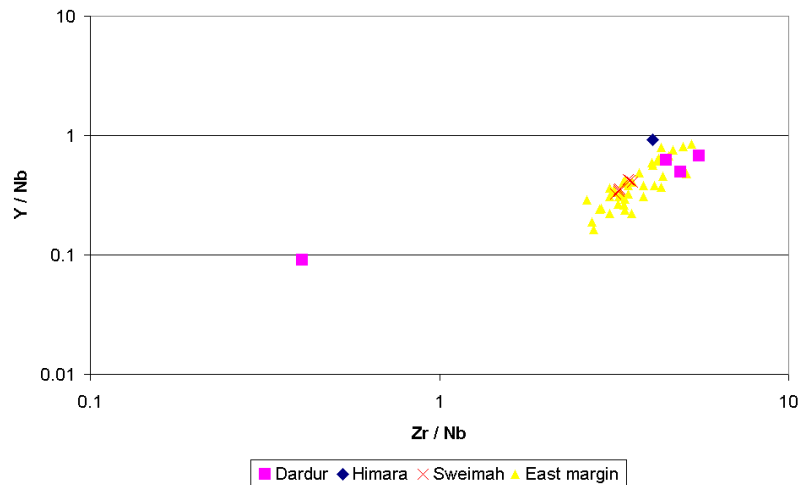
Fig 7.12: Zr/Nb-Y/Nb plot for the Dead Sea outcrops
