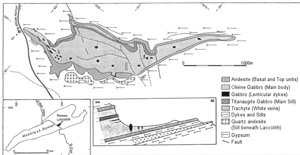
Fig 4.4: The Ramon Laccolith
