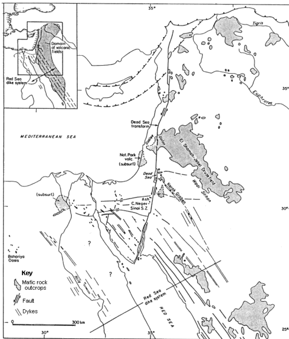
Fig 4.1: Neogene to Quaternary regional magmatic activity
