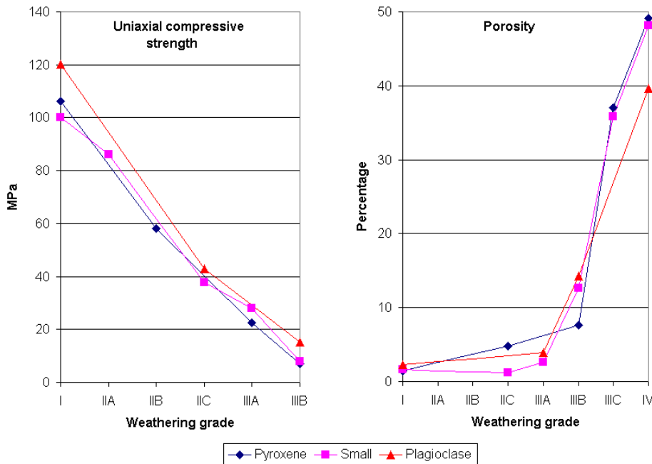
Fig 3.6: Properties of basalt rocks containing different phenocrysts
