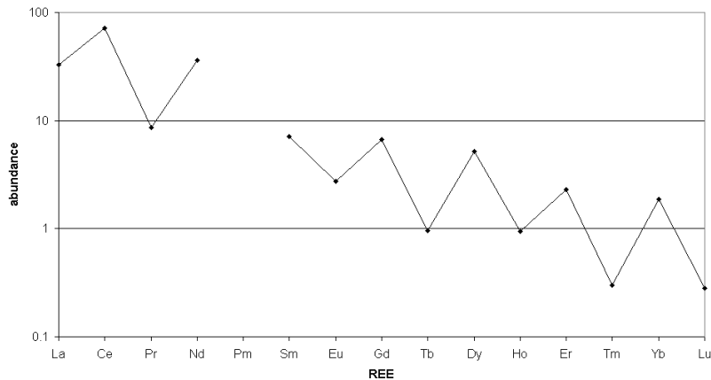
Fig 3.4: REE abundance plot of sample G165
