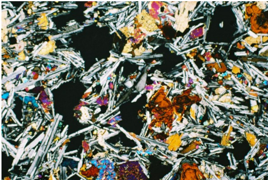
Plate 11: A075 (Hazor), basalt in XPL
