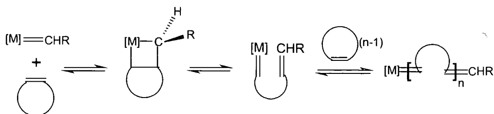
Figure 1.17 Mechanistic pathway for ring opening metathesis polymerisation
