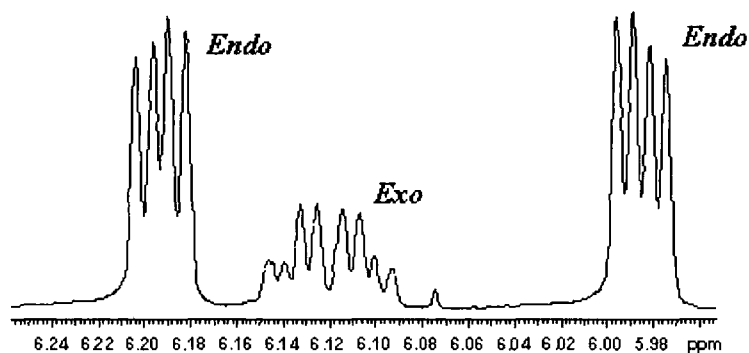
Figure 2.4 Region of the 1 H NMR spectrum of exo/endo 5-norbornene-2-carboxylic acid showing the vinylic hydrogen signals for the endo and exo isomers
