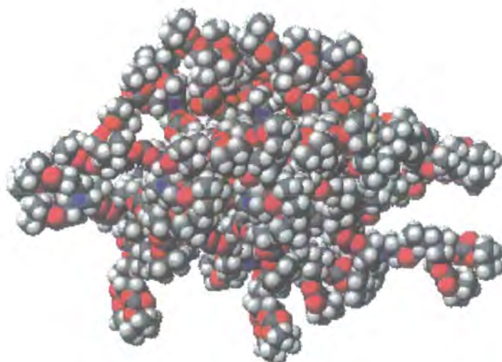
Figure 4.10 Structure corresponding to 8DP of conformer 4 (carbon = grey, oxygen = red, nitrogen = blue)
