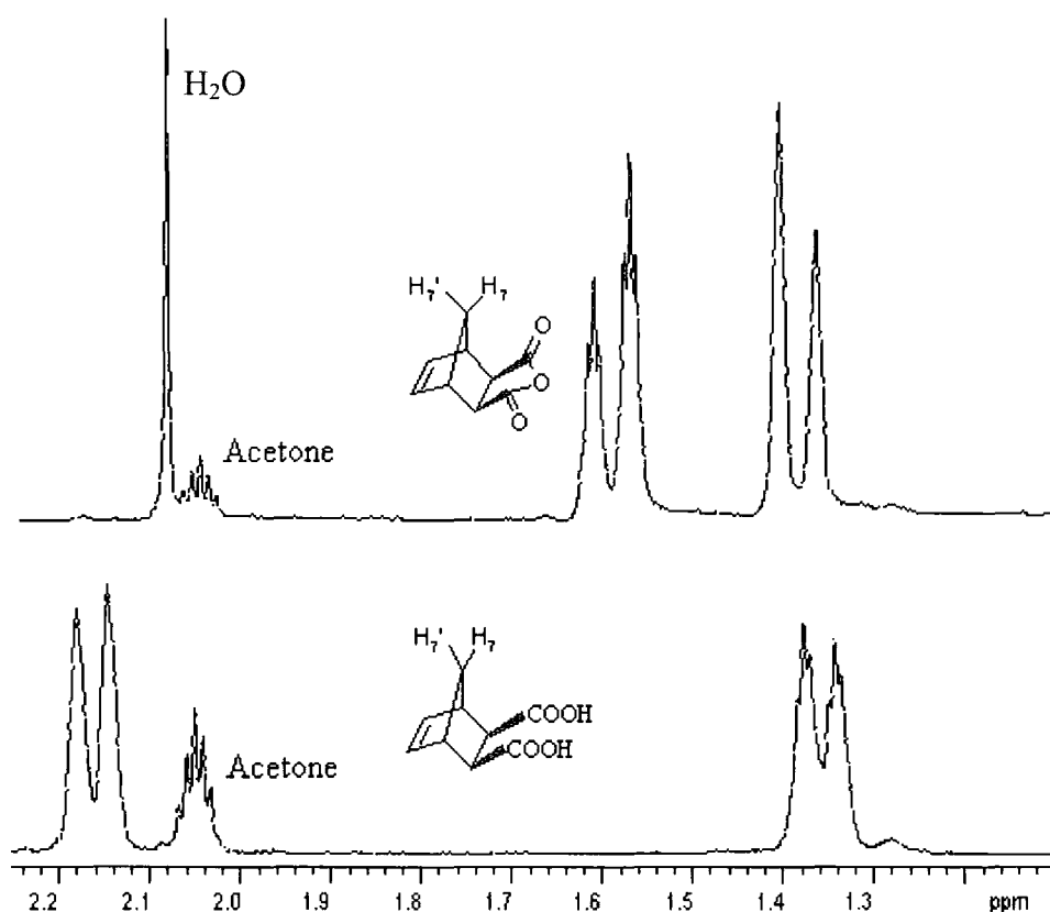
Figure 2.9 1 H NMR spectra for norbornene- exo -5, 6-dicarboxylic anhydride, top, and norbornene-5- exo , 6- exo -dicarboxylic acid, bottom.
