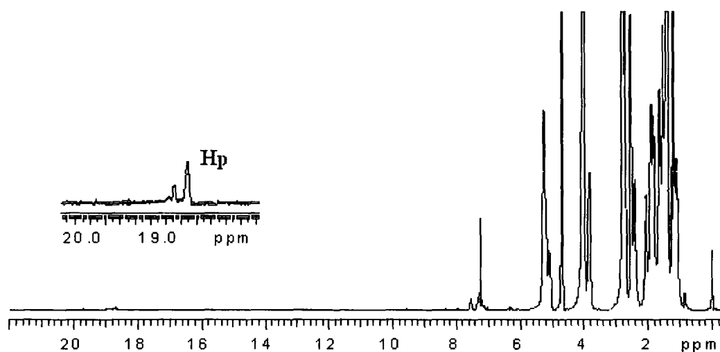
Figure 3.4 The ^1\text{H} NMR spectrum of the polymerisation of 50 molar equivalents of DMPCB1M in chloroform- d after one day
