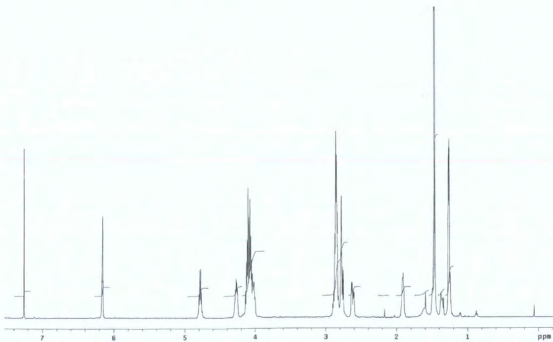
Appendix 4 1 H NMR spectrum of DMPCB1D
