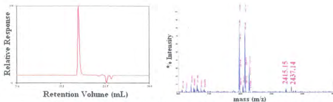
Figure 2.44 a) GPC trace of DMPUH2D b) Maldi-TOF spectrum of DMPUH2D
