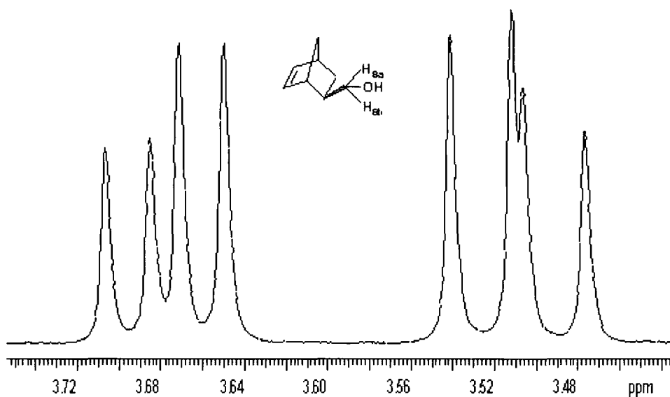
Figure 2.7 Region of the 1 H NMR spectrum of norbornene-5- exo -methanol showing diastereotopic protons H 8a and H 8b
