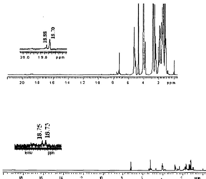
Figure 3.6 The ^1\text{H} NMR spectra of the polymerisation of 50 molar equivalents of DMPCB1M (top spectrum) and the subsequent addition of 50 molar equivalents of norbornene (bottom spectrum) (both in chloroform-d)
