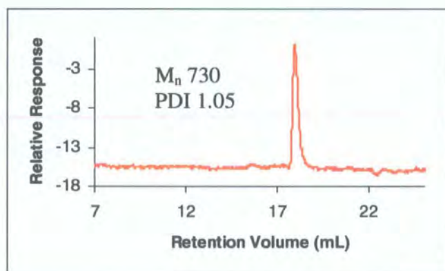
Figure 2.32 GPC trace of [7]- \text{NH}_2
