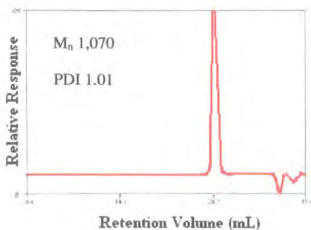
Figure 2.38 GPC trace of DMPCB1D
