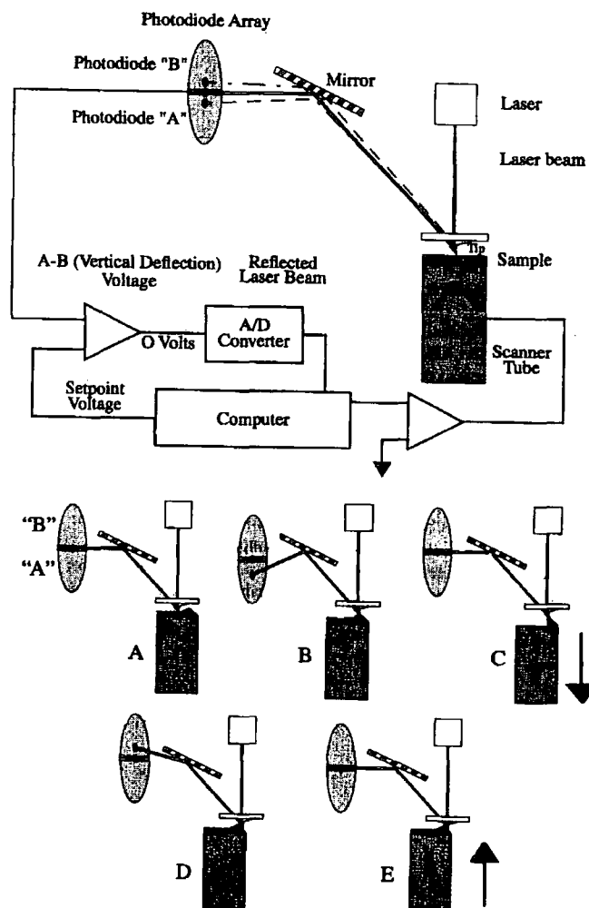
Figure 4.13 Use of a feedback loop to adjust the laser spot to its original position
