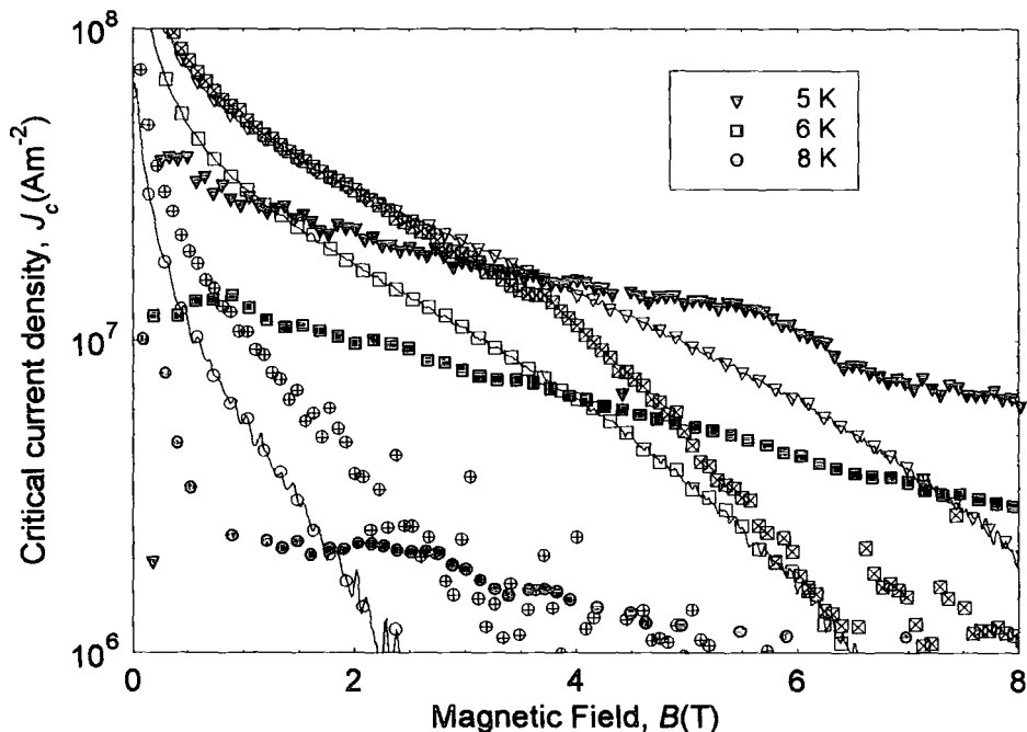
Figure 6.14. Critical current density of Pb 0.75 Eu 0.25 Mo 6 S 8 as a function of magnetic field and temperature. The closed shapes are the 150 \mu\text{m} \varnothing torque data, the open shapes are the 4 mm samples' VSM data, and the shapes with crosses inside are the 300 \mu\text{m} \varnothing samples' VSM data. The 300 \mu\text{m} \varnothing sample was not measured at 5 K.
