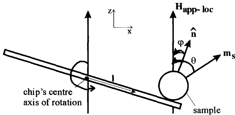
Figure 3.7. Schematic diagram of the experimental set-up of the QD torque chip, in an applied local magnetic field, \mathbf{H}_{app-loc} . In the figure \hat{\mathbf{n}} is normal to the chip, l is the distance between the sample and the centre of rotation of the chip and \mathbf{m}_s is the sample moment. The angle \theta is between the sample moment and the magnetic field and the angle \phi is between the normal to the chip and the magnetic field.
