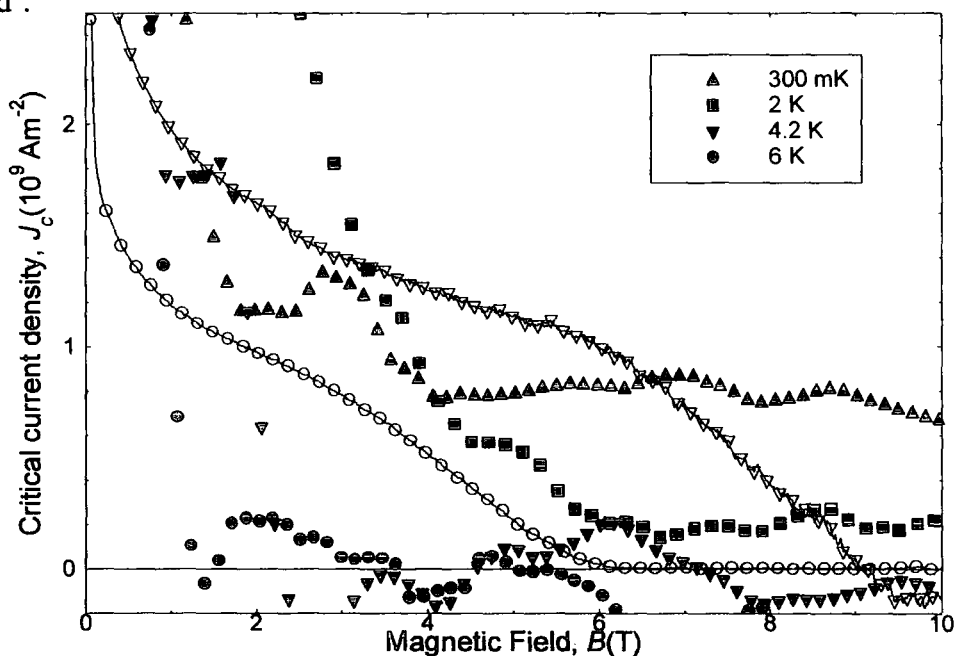
Figure 5.38. The critical current density of NbTi wire as a function of magnetic field and temperature. For these data, at each field gradient, the voltage vs. field sweep loops were measured for every temperature, before the Heliox was lifted to the next height from the magnet centre. The closed shapes are the torque data, and the open shapes are the VSM data. The sample was on chip 4.
