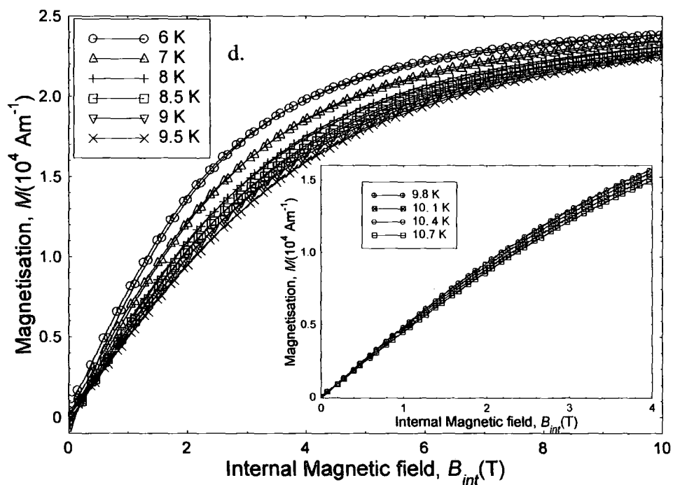
Figure 4.7c & d. Magnetisation of (\text{Pb}_{0.75}\text{Eu}_{0.25})\text{Mo}_6\text{S}_8 as a function of internal magnetic field and temperature, for (c) bulk and (d) powder samples. Insets (c) & (d): The high temperature magnetisation for x = 0.25 (a), as a function of magnetic field and temperature.
