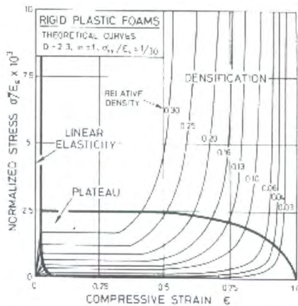
Figure 6.30 Stress-strain map for a rigid plastic foam material, constructed from the equations in 1.2.3 (6) .
