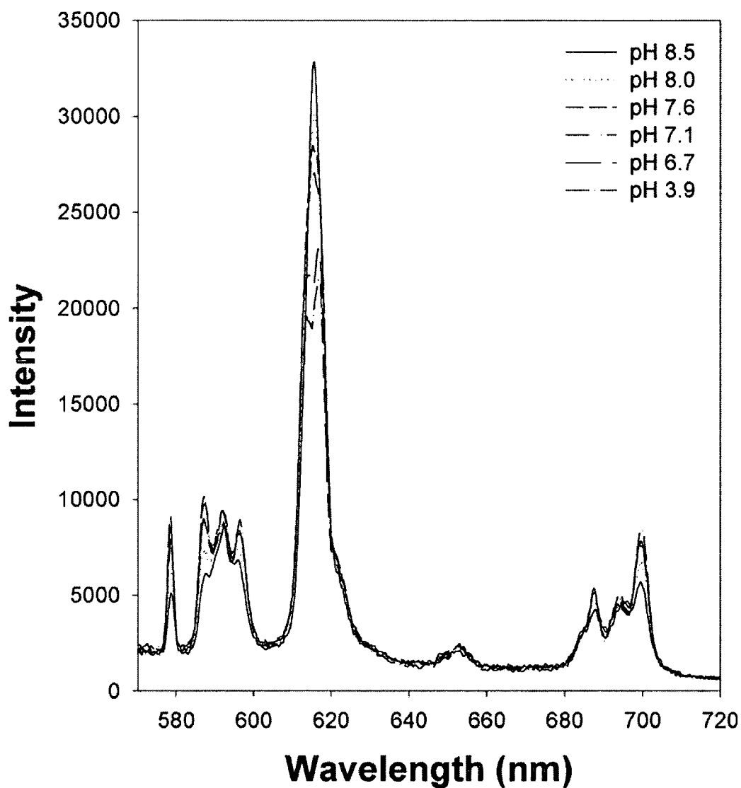
Figure 4.17 Effect of pH on sensitised emission ( \lambda_{\text{ex}} 271 nm) of [EuL 9 ] in an extracellular anion background.
