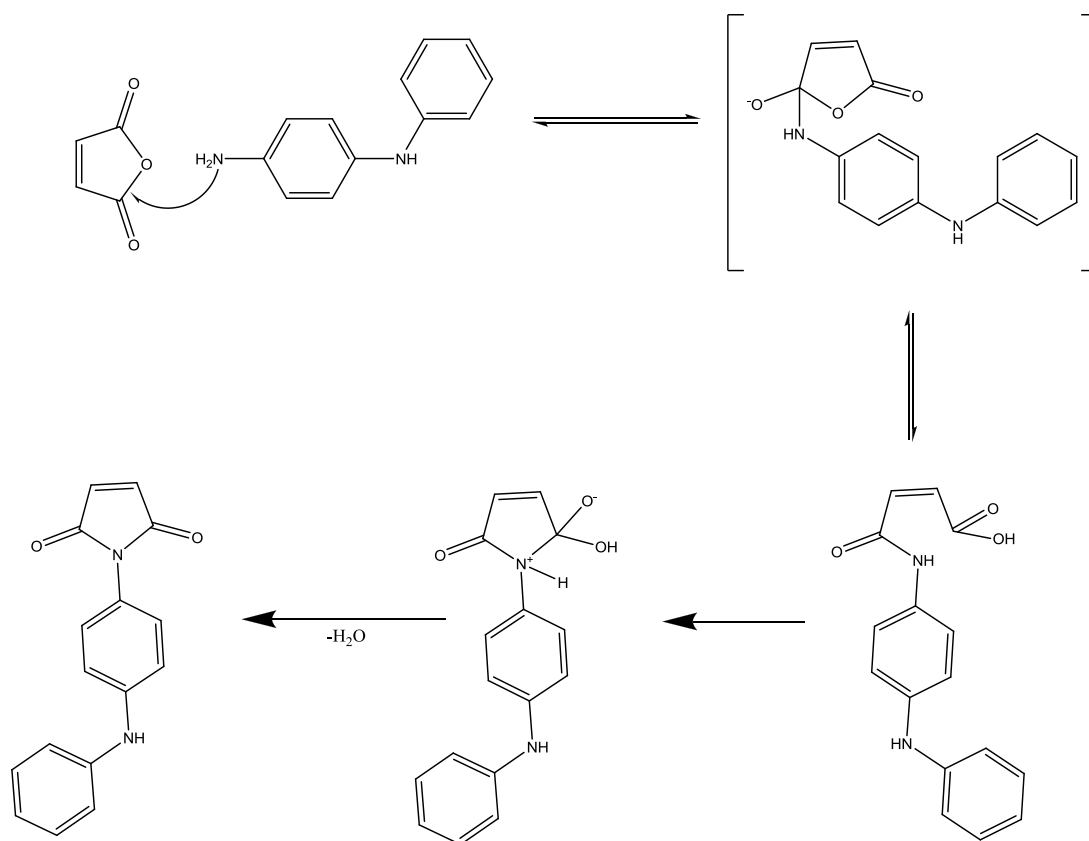
Figure 72: Proposed mechanism of N-maleimide formation
