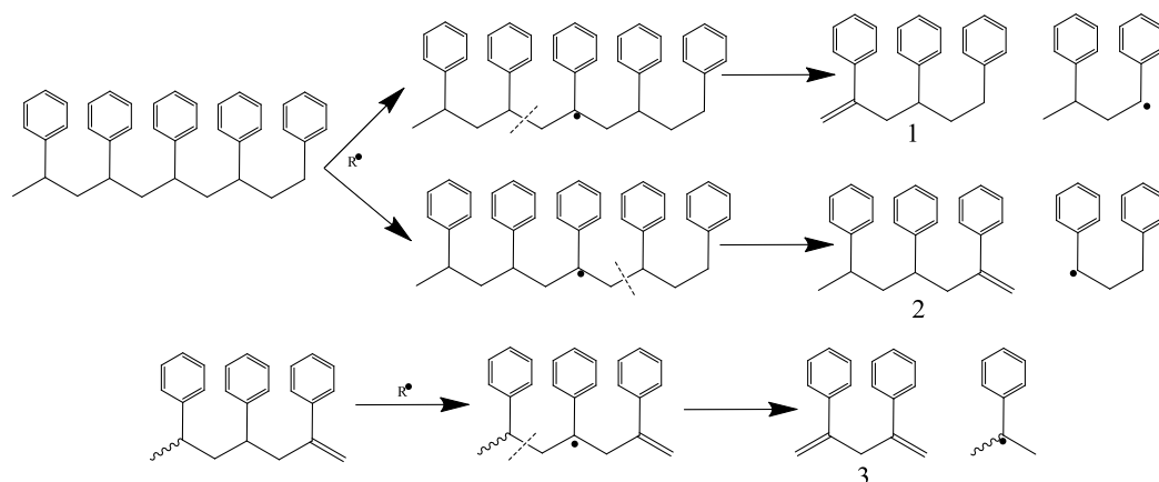
Figure 33: Polystyrene degradation reactions leading to terminal olefin formation
