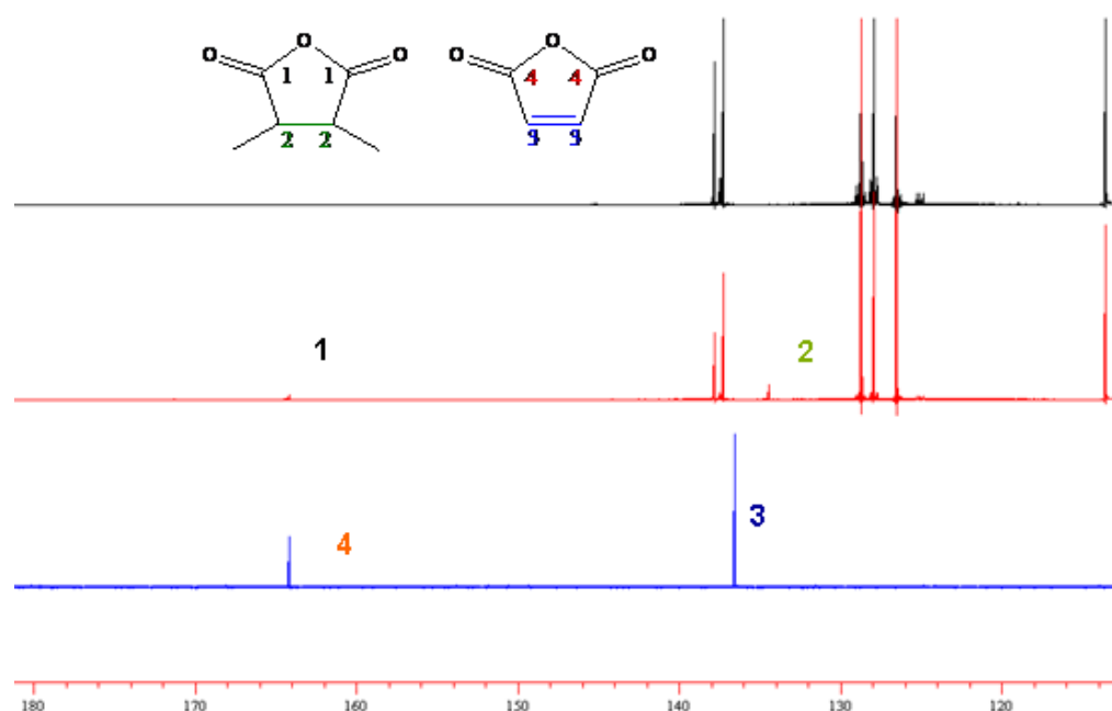
Figure 55: Comparison of the 125MHz ^{13}\text{C} NMR spectra showing 180-110ppm; top spectrum: RAFT polymerisation of styrene. Middle spectrum: RAFT polymerisation of styrene with maleic anhydride addition after 48h. Bottom spectrum: maleic anhydride monomer.
