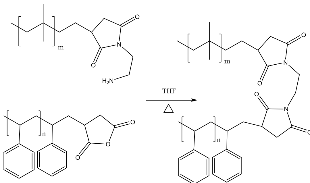
Figure 71: Coupling of maleic anhydride functionalised waste polystyrene with PIB-amine
