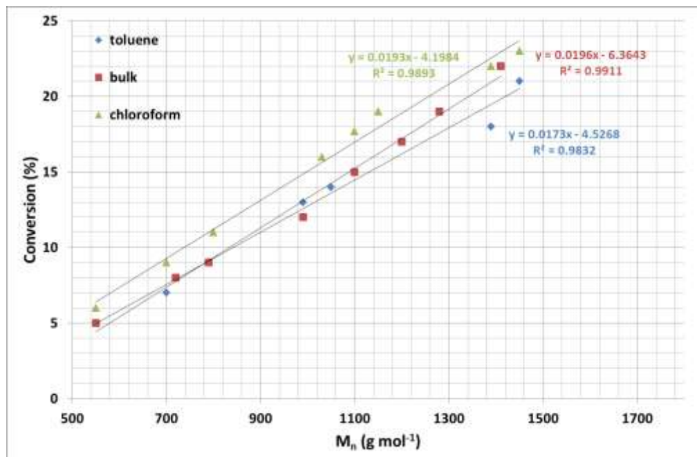
Figure 52: Molecular weight vs conversion for the RAFT polymerisation of styrene in toluene, bulk and chloroform at 70°C.
