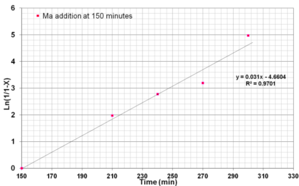
Figure 49: Kinetic plots for the addition of maleic anhydride at t=150 min. Conversion was determined by offline ^1\text{H} NMR spectroscopy.
