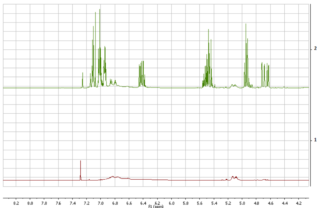
Figure 32: ^1\text{H} NMR spectra for 1) The waste polystyrene mixture prior to degradation 2) the residual waste product at 160minutes
