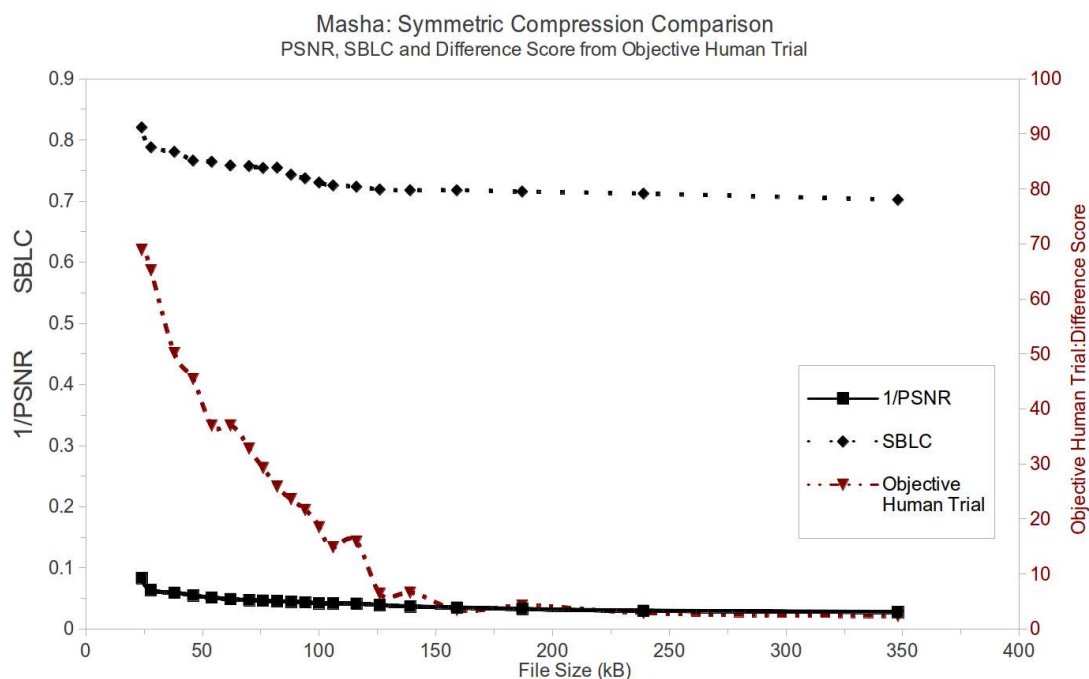
Figure 7.2: Masha : PSNR, SBLC and Difference Score from the Human Trial
