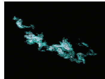
Figure 6.5: Perseus .
