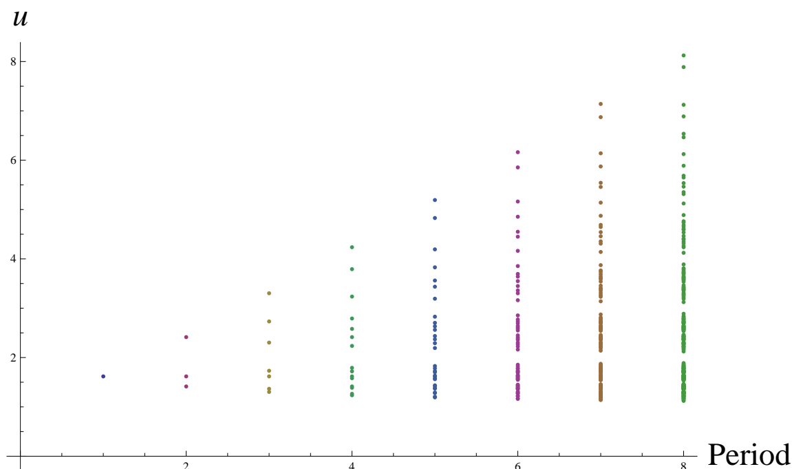
Figure 6.1: A plot of the periodic values of u plotted by period
