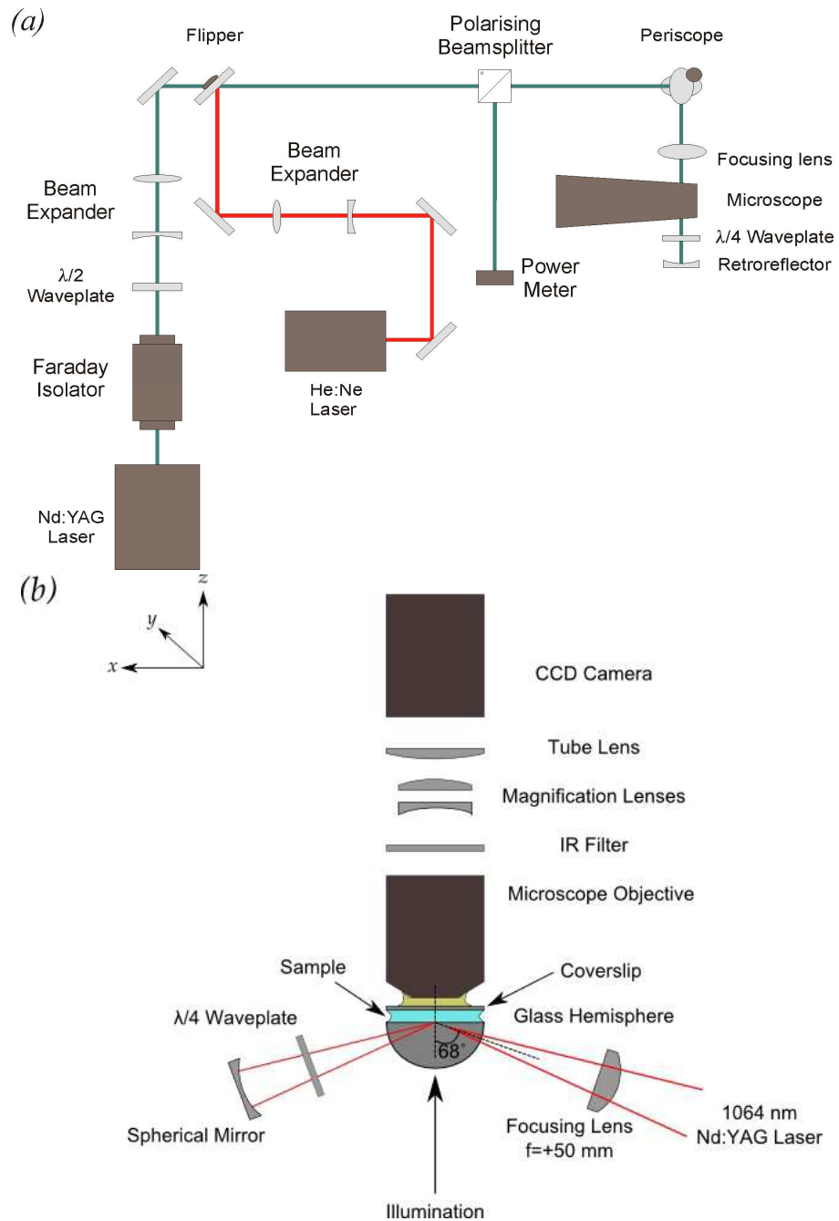
Figure 2.3: Schematic showing (a) the optical bench layout, and (b) the experimental setup around the microscope for optical trapping in evanescent waves generated by TIR with a Nd:YAG \lambda=1064 nm laser.
