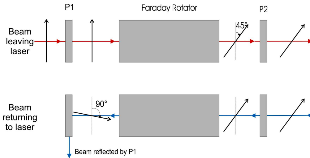
Figure 2.4: Schematic showing a Faraday Isolator. Black arrows indicate the polarisation of light.
