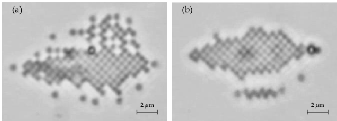
Figure 3.5: Arrays comprised of large numbers of 460 nm PS are square (a) in p -pol, but with many edge defects; (b) in s -pol. ( \theta_i = 56^\circ ; D = 380\text{nm} ; n_{\text{SF10}} = 1.702 ; \lambda = 1064 nm).
