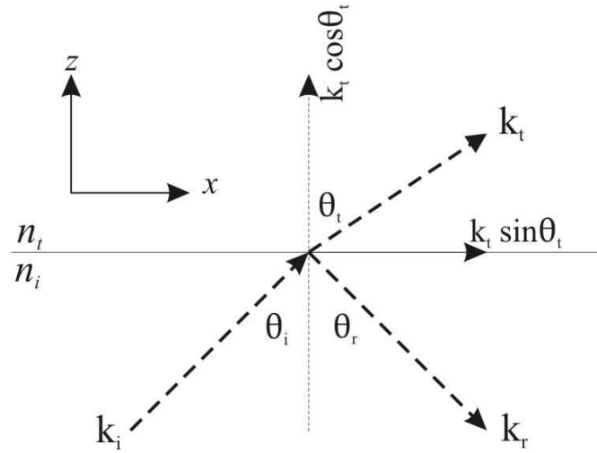
Figure 2.1: Propagation vectors for internal reflection. The x - y plane is the interface, and the x - z plane is the plane of incidence.
