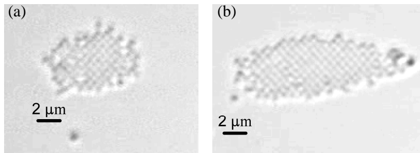
Figure 3.10: Arrays of 520nm silica particles are square and commensurate in (a) p -pol, and (b) s -pol. ( n_{SF10}=1.507 ; \theta_i=68^\circ ; \lambda=1064 nm)
