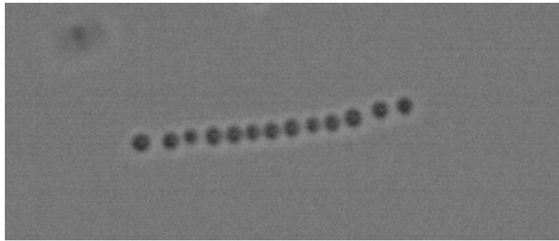
Figure 5.5: Incoherently trapped line array of 620 nm PS at \lambda = 865 nm, in p -pol. Particles spacings were seen to decrease towards the centre of the line. ( n_{BK7} = 1.507 ; \theta_c = 62.2^\circ ; \theta_i = 64.5 )
