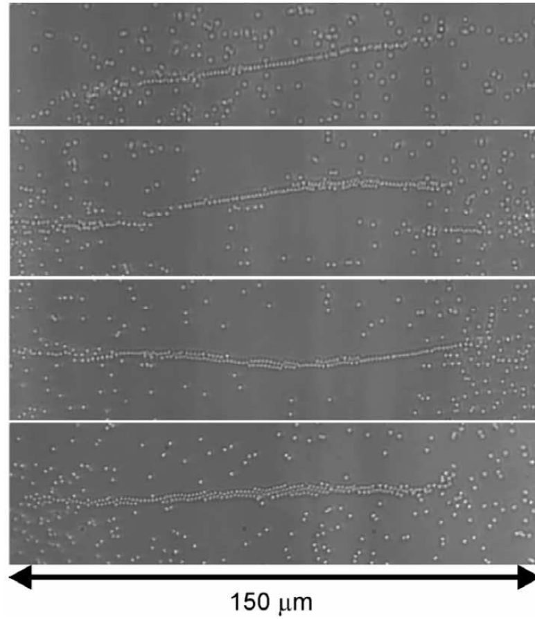
Figure 1.11: Chain-like structures of 1 \mu\text{m} silica formed for different input powers (corresponding peak intensity on the surface is given in brackets): (i) 100 mW (0.34 \text{mW } \mu\text{m}^{-2} ); (ii) 175 mW (0.68 \text{mW } \mu\text{m}^{-2} ); (iii) 219 mW (0.94 \text{mW } \mu\text{m}^{-2} ); (iv) 266 mW (1.02 \text{mW } \mu\text{m}^{-2} ). 49
