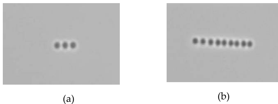
Figure 3.17: Build-up of a line of uncoated 881 nm silica particles showing (a) uniform separations of 3D ; and (b) modulated ‘pairs’.
