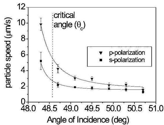
Figure 1.6: Velocity of 5 \mu\text{m} polymer colloids at a BK7 glass-water interface, resulting from optical interactions with evanescent waves generated by p - (solid triangles) and s -polarized (solid squares) light incident at different incident angles around the critical angle. Solid lines are an aid to the eye. The dotted line represents the experimentally determined critical angle. 37
