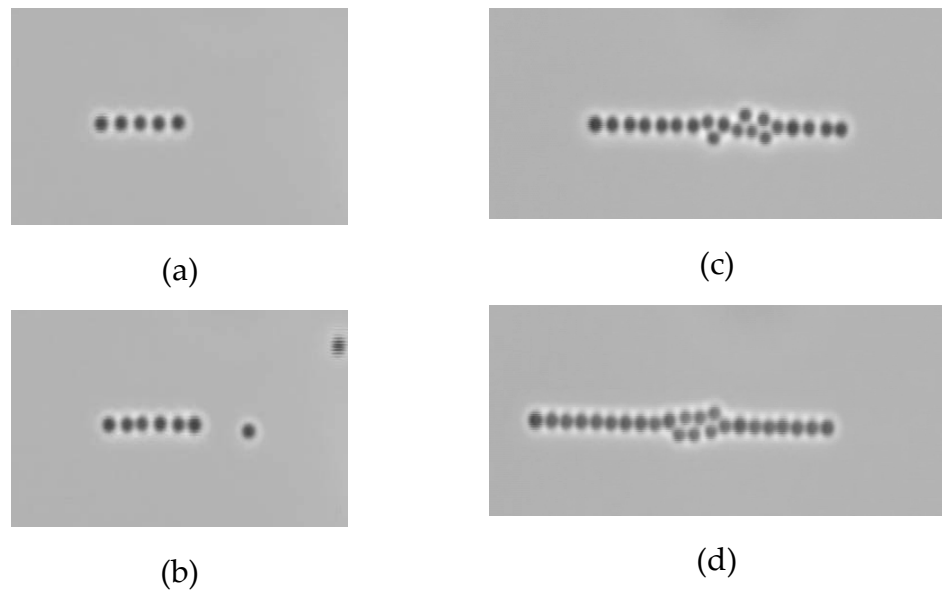
Figure 3.16: Build-up of a line of half-Au coated 881 nm silica microspheres showing (a) uniform separations of 3D ; (b) modulated ‘pairs’; (c) modulated separations persisting as particles sit in a 2 nd row; and (d) particles in close contact as even more particles are trapped. ( n_{\text{BK7}}=1.507 ; \theta_i=64^\circ ; s -pol; \lambda=1064 nm)
