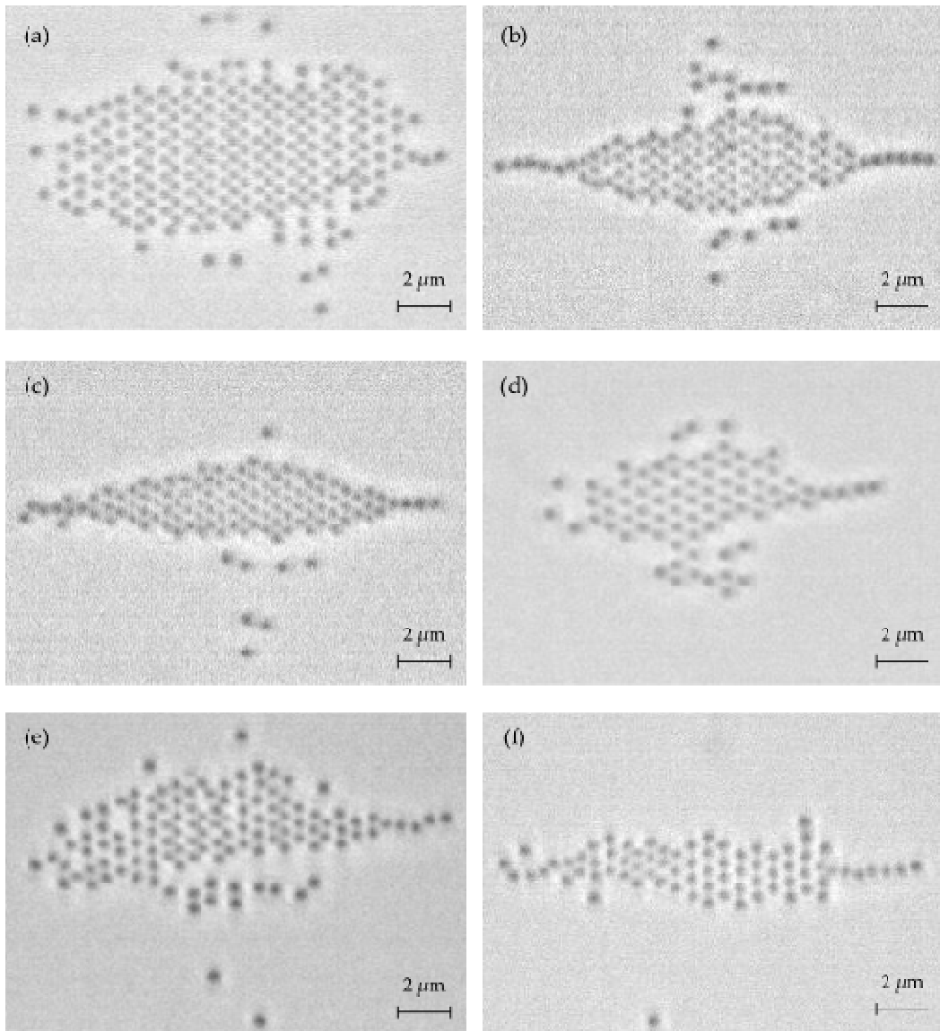
Figure 4.2: Arrays of 420 nm PS in p -pol at: (a) \lambda=890 nm showing broken hex2; (b) \lambda=880 nm showing broken hex2; (c) \lambda=870 nm showing an incommensurate hex2; (d) \lambda=860 nm showing an incommensurate hex2; (e) \lambda=850 nm showing hex2 with transient broken hex2 structure; and (f) \lambda=840 nm showing hex2.
