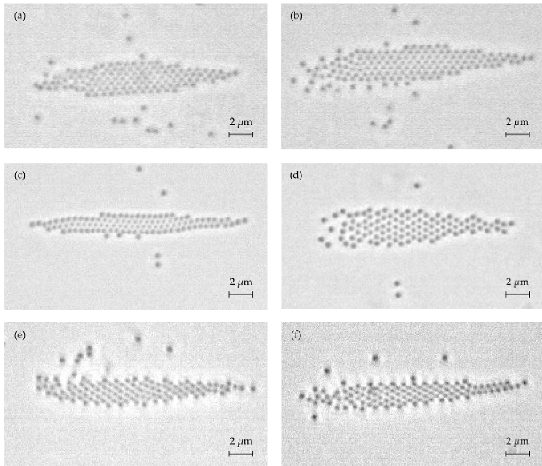
Figure 4.3: Arrays of 420 nm PS in s -pol at: (a) \lambda = 890 nm showing square-hex1 intermediate; (b) \lambda = 880 nm showing square-hex1 intermediate; (c) \lambda = 870 nm showing an incommensurate hex1; (d) \lambda = 860 nm showing an incommensurate hex2; (e) \lambda = 850 nm showing hex2; and (f) \lambda = 840 nm showing hex2. ( n_{BK7} = 1.507 ; \theta_c = 62.2^\circ ; \theta_i = 64.5^\circ ).
