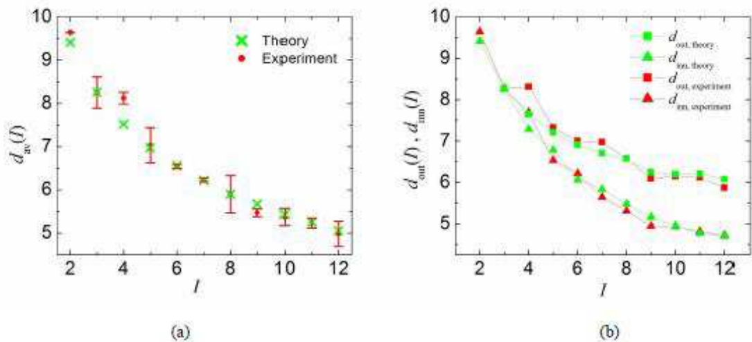
Figure 1.2: Inhomogeneous properties of inter-particle spacing. (a) Averaged inter-particle spacing d_{av} as a function of the number of particles I . (b) The inner most inter-particle spacing d_{in} and the outer most interparticle spacing d_{out} , as a function of I . 28
