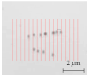
Figure 3.14: Reptating lines of 250 nm Au particles in incident s -pol. Stacked particles are seen as darker spots. Calculated interference fringes are superimposed in red. ( n_{BK7} = 1.507 ; \theta_i = 68^\circ ; D = 380 nm)
