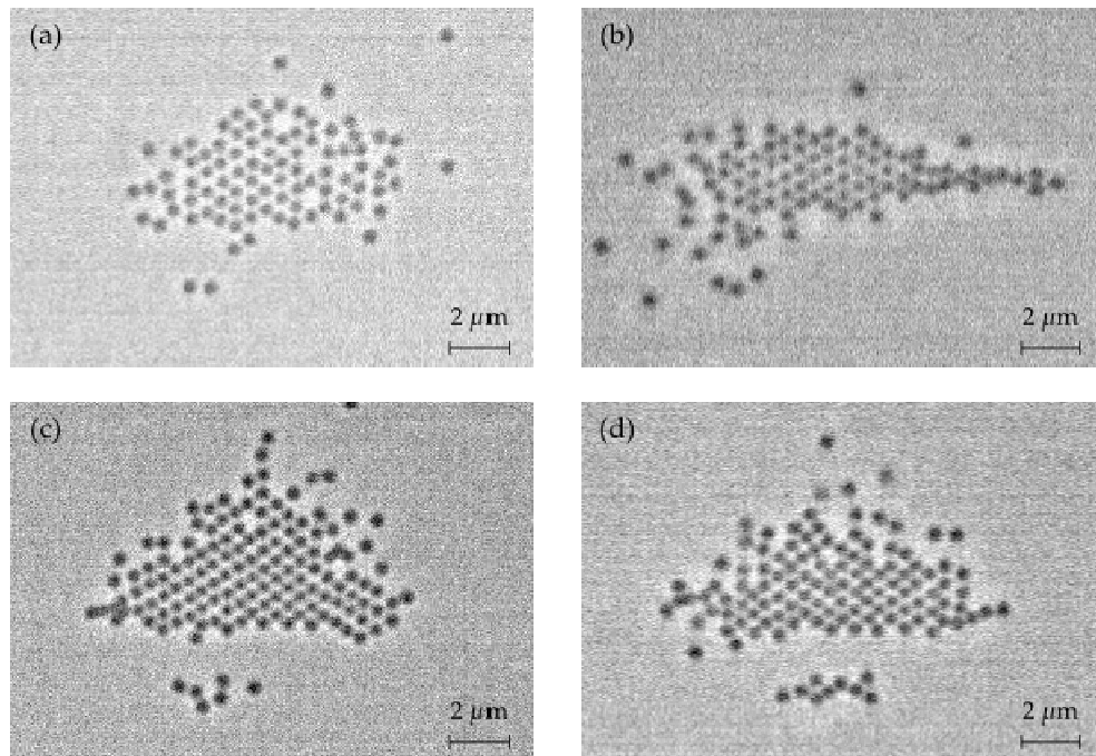
Figure 5.3: Incoherently trapped arrays of 520 nm PS in p -pol at: (a) \lambda = 840 nm, showing hex2; (b) \lambda = 865 nm, showing hex-2; (c) \lambda = 865 nm, showing square-hex-2 intermediate; and (d) \lambda = 890 nm, showing square-hex-2 intermediate. ( n_{BK7} = 1.507 ; \theta_c = 62.2^\circ ; \theta_i = 64.5^\circ )
