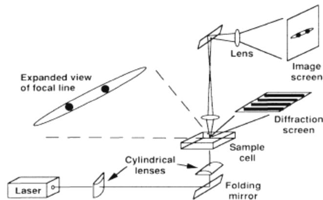
Figure 1.1: Experimental setup for transverse optical binding as performed by Burns, Fournier and Golovchenko in 1989. 15, 16
