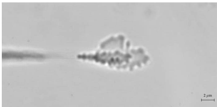
Figure 6.1: Large numbers of 520 nm PS particles being ejected at high speed from the array. ( \theta_i = 53^\circ ; \theta_c = 51.6^\circ ; n_{SF10} = 1.702 ; \lambda = 1064 \text{ nm} )
