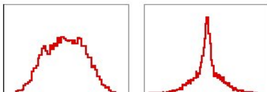
Figure 3.7: The Negative and The Positive Kurtosis
