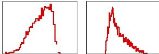
Figure 3.6: The Negative and The Positive Skew
