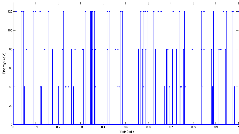
Fig 4-4 Simulation of the random arrival of events at a detector over 1 ms. Here the expected count rate for each of the three energies is 33,000 counts per second.
