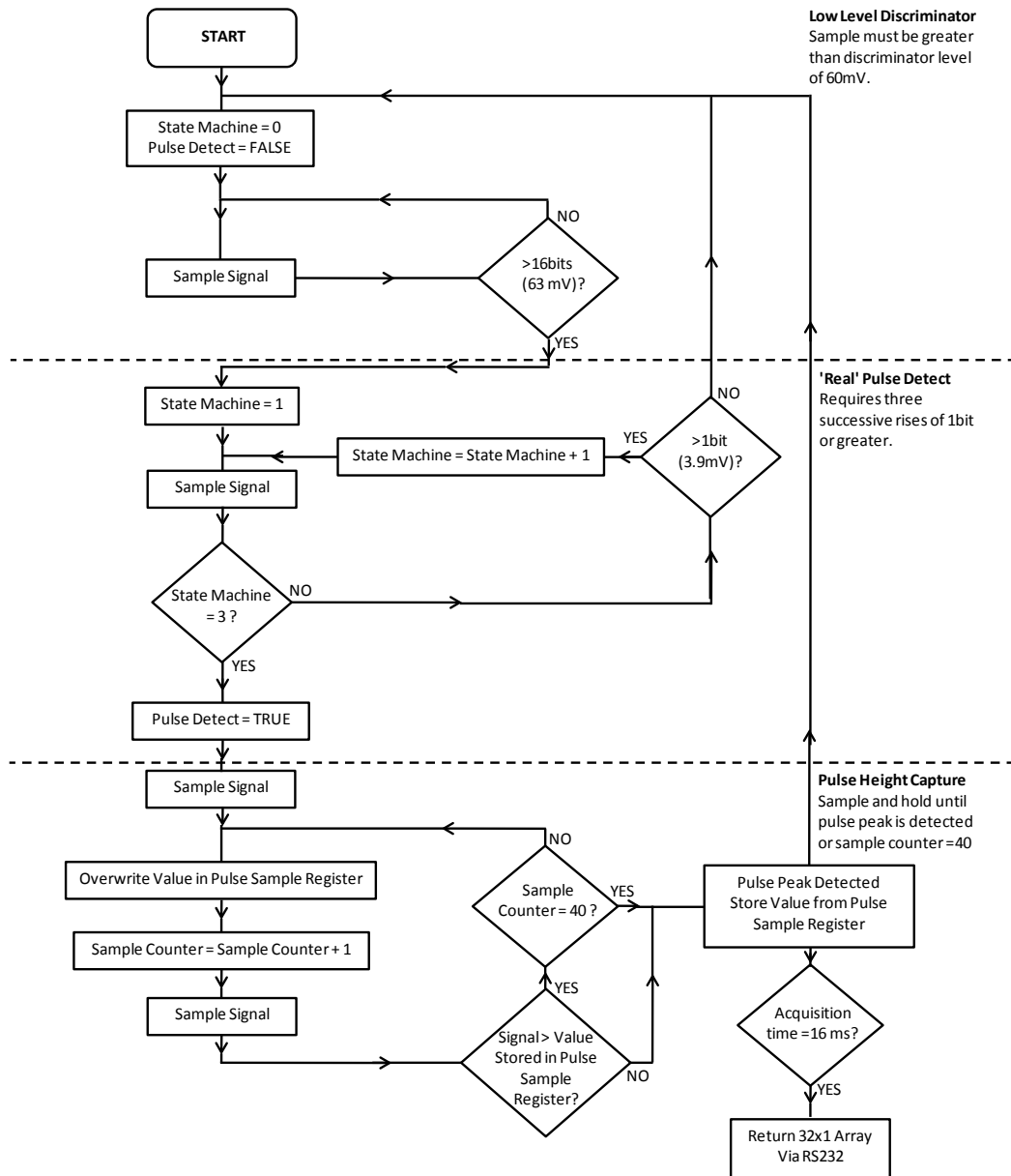
Fig 4-8 Flow chart describing the operation of pulse height detection Algorithm 1.
