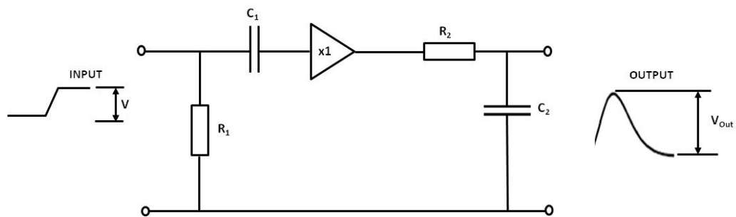
Fig 2-6 Schematic diagram of a simple CR-RC network. The unity gain buffer amplifier separates the filter stages for impedance isolation.
