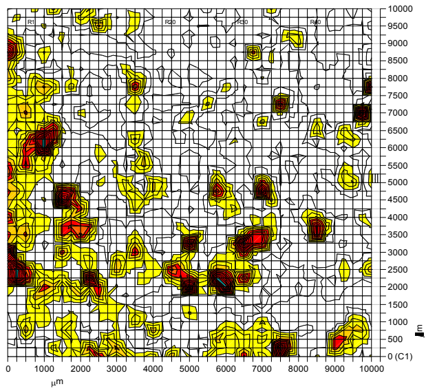
Fig 3.8.10 Map of natural luminescence intensity, measured across the surface of sample 316-2. Areas shaded red represent the highest levels of luminescence emission, whilst areas shaded yellow represent luminescence emission at levels that are substantially (2X or more) above sample background levels.
