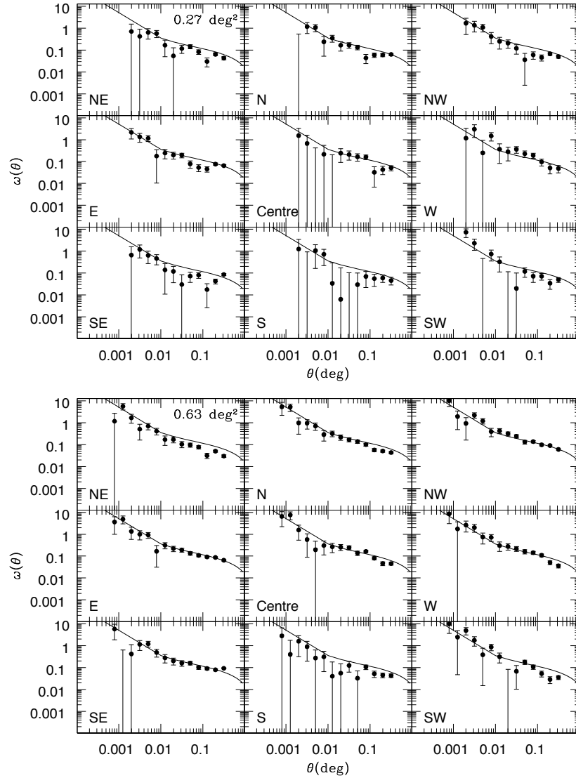
Figure 3.18: The angular correlation functions corrected for the integral constraint of EROs for 0.27 \text{ deg}^2 (top) and 0.63 \text{ deg}^2 (bottom) fields at each position. The solid lines indicate the best fit of K < 18.8 and i - K > 4.5 EROs in the whole field.
