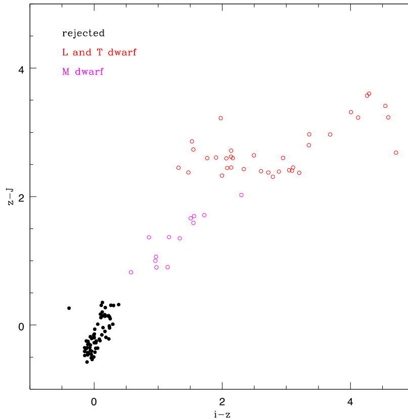
Figure 2.11: The z-J versus i-z diagram for brown dwarves. Filled circles indicate rejected objects from T dwarf candidates. Magenta and red open circles show known M dwarf and L, T dwarves, respectively, from Hewett et al. (2006).
