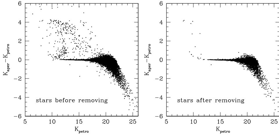
Figure 2.3: The difference of aperture and Petrosian magnitude of stars versus Petrosian magnitude. The left panel shows plot for all stars. The right panel presents the plot after removing objects having a close neighbour. The scatter is decreased after removing objects having a neighbour.
