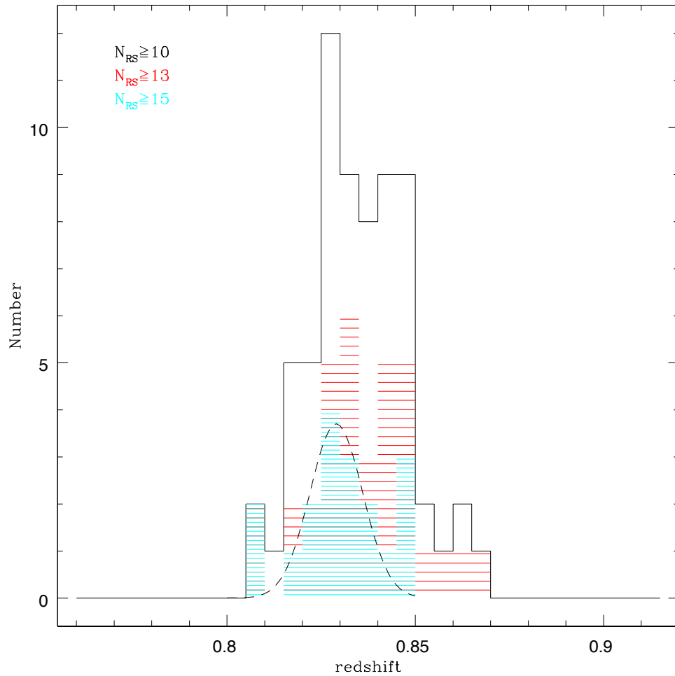
Figure 6.13: The Photometric redshift distribution of massive cluster candidates displayed in Figure 6.12 with the same colour coding. The dashed line shows the Gaussian fit for candidates at 0.815 < z_{phot} < 0.845 .
