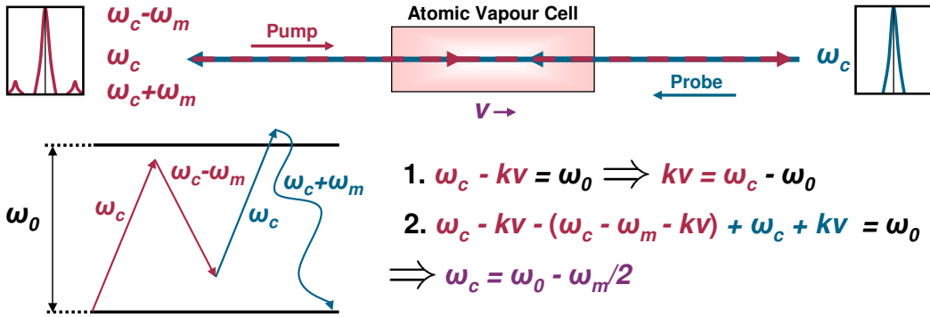
Figure 3.4: A simple setup for modulation transfer. A phase-modulated pump beam and a counter-propagating, unmodulated probe beam are aligned collinearly through a vapour cell. Four-wave mixing results in modulation transfer and generates a sideband on the probe beam. The four-wave mixing process is described in the text.
