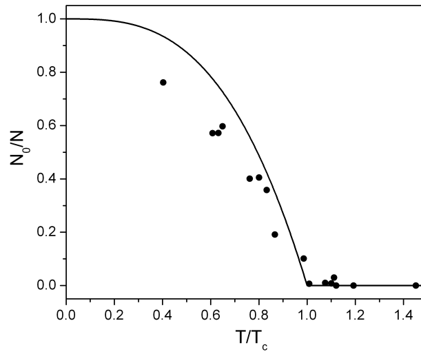
Figure 5.5: ^{87}\text{Rb} condensate fraction vs the scaled temperature T/T_c . The experimental data were determined from double Gaussian fits applied to density profiles recorded via absorption imaging. The solid line is the theoretical curve from equation 2.26. At the transition the cloud consists of 1.2(1) \times 10^6 atoms at 0.37(3) \mu\text{K} .
