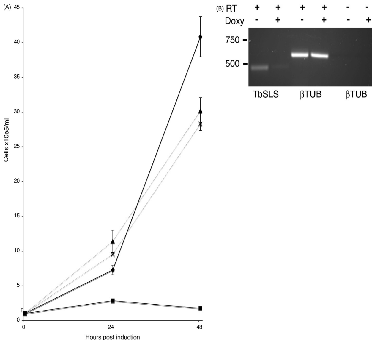
Fig. 6. TbSLS is an essential enzyme in bloodstream form T. brucei . (A) Inhibition RNA of TbSLS. Cell counts over a 48 h period: (x) mock transfected cells induced by 1 µg/ml doxycycline; (♦) TbSLS RNAi cells non-induced; (■) TbSLS RNAi cells induced by 1 µg/ml doxycycline. Error bars for standard deviation over three replicates are shown. (B) RT-PCR using total RNA isolated from TbSLS RNAi parasites with or without doxycycline induction (Doxy). RT, reverse transcriptase. βTUB, β tubulin control.
