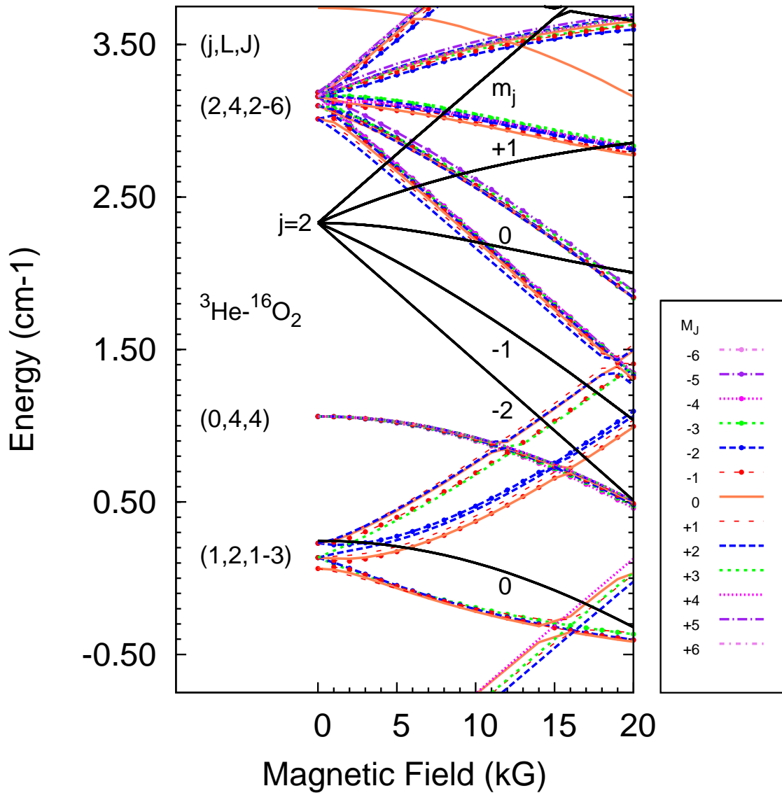
Figure 5.9: The Zeeman structure of the quasi-bound states of {}^3\text{He}-{}^{16}\text{O}_2 . For the energy range depicted, the highest projection quantum number is M_J = +6 . The solid black lines show the levels of {}^{16}\text{O}_2 which are the collision threshold levels of the complex. Only quasi-bound states with the same symmetry as the {}^{16}\text{O}_2 level can result in zero-energy S-wave resonances.
