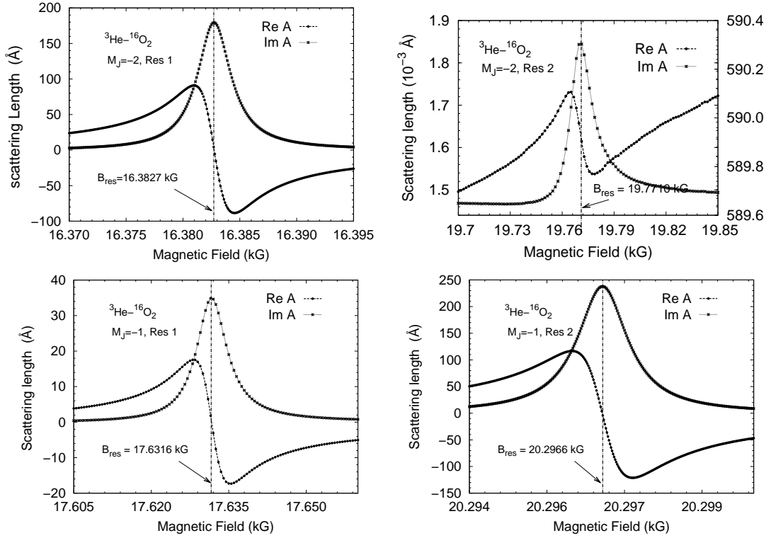
Figure 5.19: The real and imaginary parts of the scattering length across resonances of ^3\text{He-}^{16}\text{O}_2 , for M_J = -2 and -1 symmetry. For Res 2 of M_J = -2 symmetry, the y-axis of the real and imaginary parts have been separated, with the y-axis of the real part to the right. This is because of the difference in magnitude between them. Also note the 10^{-3} scaling factor, which applies to both real and imaginary parts.
