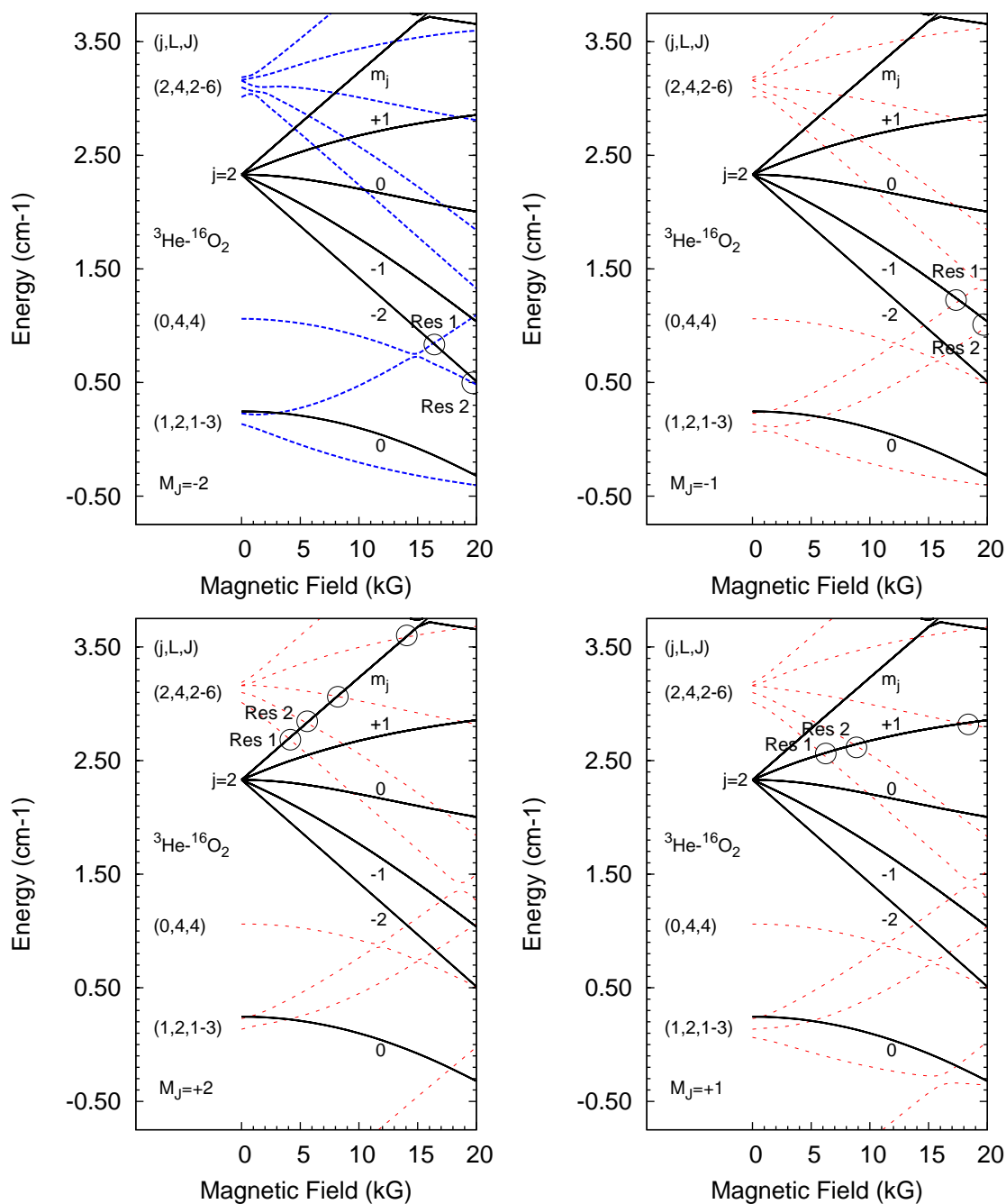
Figure 5.8: Quasi-bound levels of ^3\text{He-}^{16}\text{O}_2 of M_J = \pm 1, \pm 2 symmetry. Each graph shows levels of unique total angular momentum projection M_J (in dotted colored lines) and the threshold levels (in a solid black line). The circles indicate positions of zero-energy resonances.
