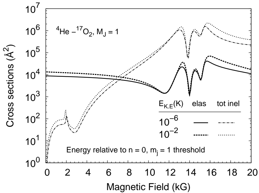
Figure 5.2: Elastic and inelastic cross sections of collisions of {}^4\text{He} with {}^{17}\text{O}_2 for collision energies 10 mK and 1 \mu\text{K} . The incoming channel belongs to the trappable (n, j, m_j) = (0, 1, 1) threshold of {}^{17}\text{O}_2 . The overall symmetry of the scattering state is M_J = 1 .
