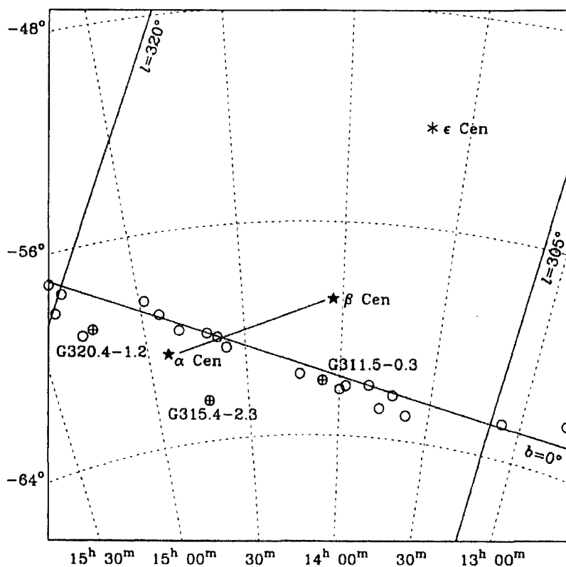
Figure 4.1 – Remnants in the Nanmen Area 22
