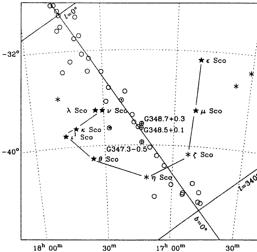
Figure 4.3 – Remnants in the Scorpius Region 28
