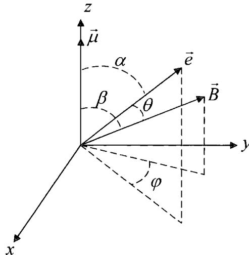
Figure 5-4. Orientation axis and angle notation for a particle in colloidal state
