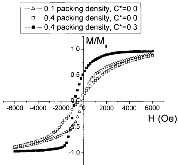
Figure 3-10. Interaction effects for systems with average particle diameter of 6nm, anisotropy constant of 4.0 \times 10^6 erg/cc and temperature of 300K
