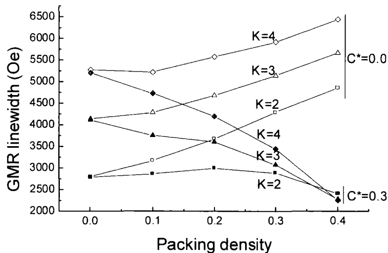
Figure 3-37. GMR linewidth as a function of anisotropy and packing density
