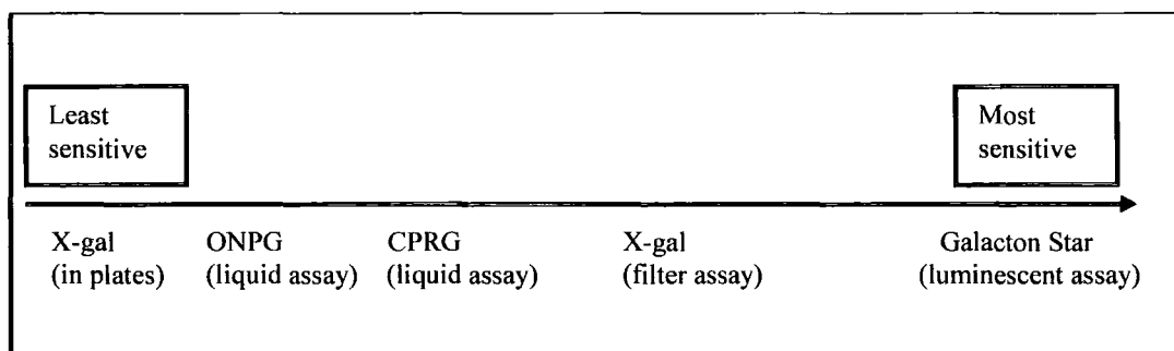
Figure 3.1. Relative sensitivity of the five types of \beta -galactosidase assays. The X-gal filter assays have been reported to be approximately 10^6 fold more sensitive than ONPG liquid assays and were subsequently used for this work. CPRG (chlorophenol red- \beta -D-galactopyranoside; ONPG, o -nitrophenyl \beta -D-galactopyranoside (Breedon and Nasmyth, 1985; Clontech, UK).
