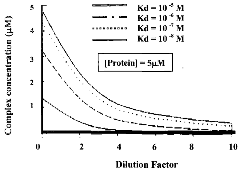
Figure 1.6. Computer-generated curves for the dissociation of a bienzyme ( E_1 and E_2 ) complex. Whereby, E_1E_2 \leftrightarrow E_1 + E_2 (Srere and Mathews, 1990).
