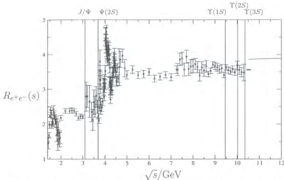
Figure 5.2: Data used to compare with model, statistical errors shown only.
