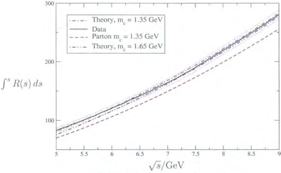
Figure 5.9: Area under R_{e^+e^-}(s)
