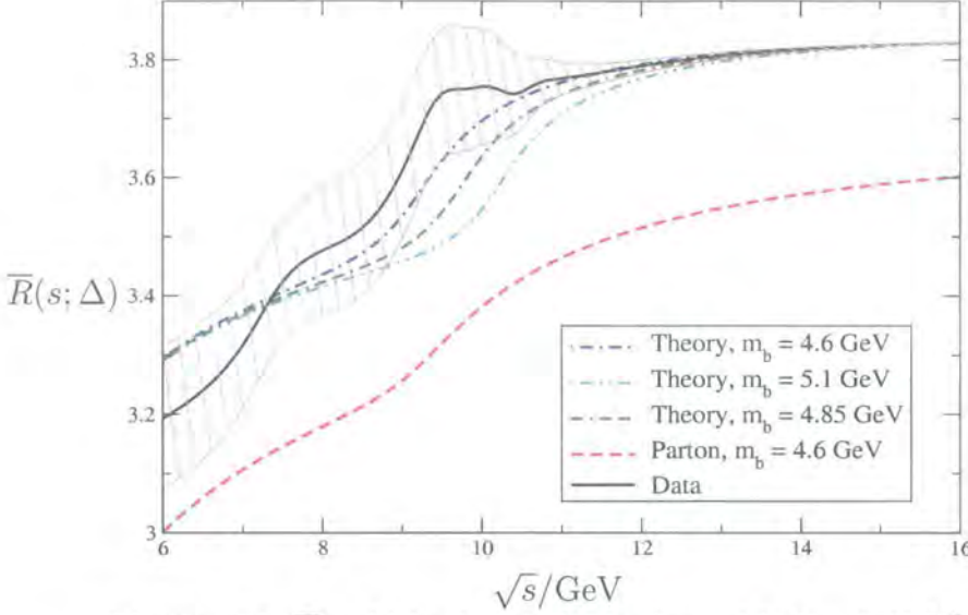
Figure 5.8: \bar{R}(s; \Delta) in the upsilon region, with \Delta = 10\text{GeV}^2 .
