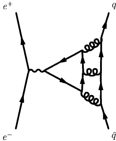
Figure 4.1: Light-by-light diagram contributing to R_{e^+e^-}
