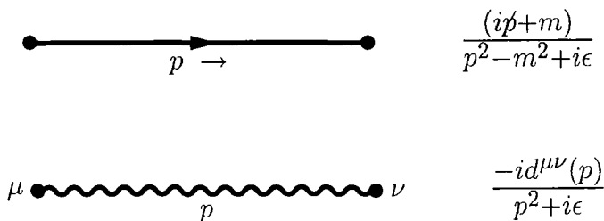
Figure 1.5: QED propagators
