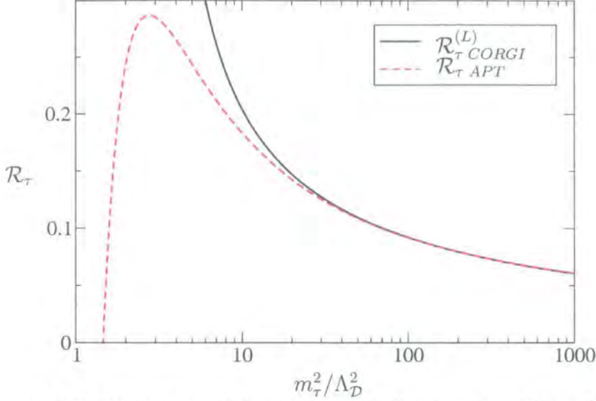
Figure 6.8: Comparison of fixed-order and all-orders calculations for \mathcal{R}_\tau .
