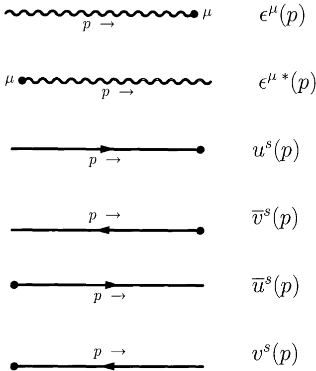
Figure 1.6: QED external particles
