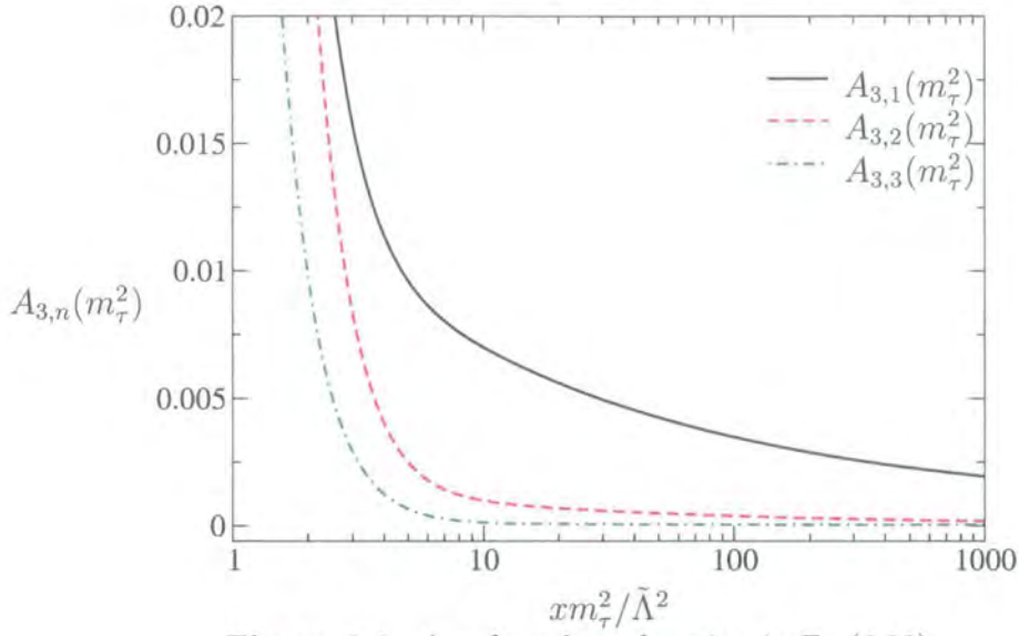
Figure 6.6: A_{3,n} from beta function in Eq.(6.28)
