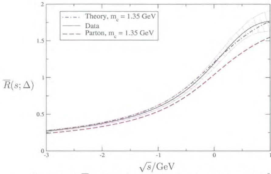
Figure 5.6: \bar{R}(s; \Delta) in the spacelike region, with \Delta = 1\text{GeV}^2 .
