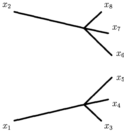
Figure 1.3: Diagram that contributes to \langle 0|T\phi(x_1)\cdots\phi(x_8)|0\rangle but not to 2 \rightarrow 6 scattering.
