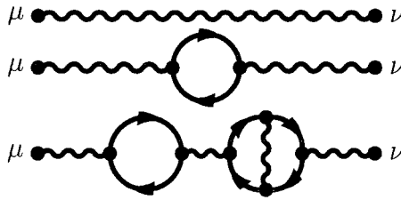
Figure 2.3: Feynman diagrams contributing to Eq.(2.8)
