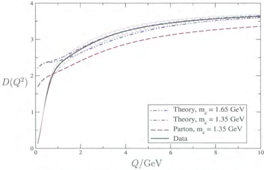
Figure 5.10: D(Q^2) calculated using APT.
