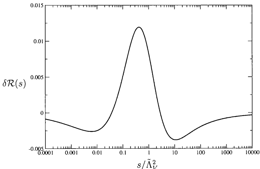
Figure 4.5: \delta\mathcal{R}(s) = \text{all orders}\mathcal{R}(s) - \text{fixed order}\mathcal{R}(s) at the one-loop level for 2 flavours of quark.
