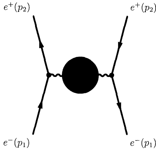
Figure 1.11: Hadronic correction to electron positron scattering
