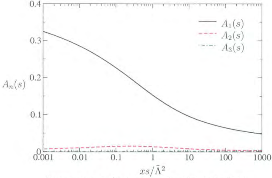
Figure 6.4: A_n(s) from beta function in Eq.(6.28)
