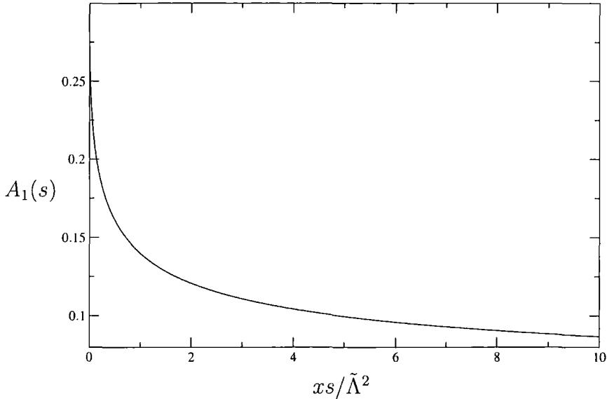
Figure 4.2: A_1(s)
