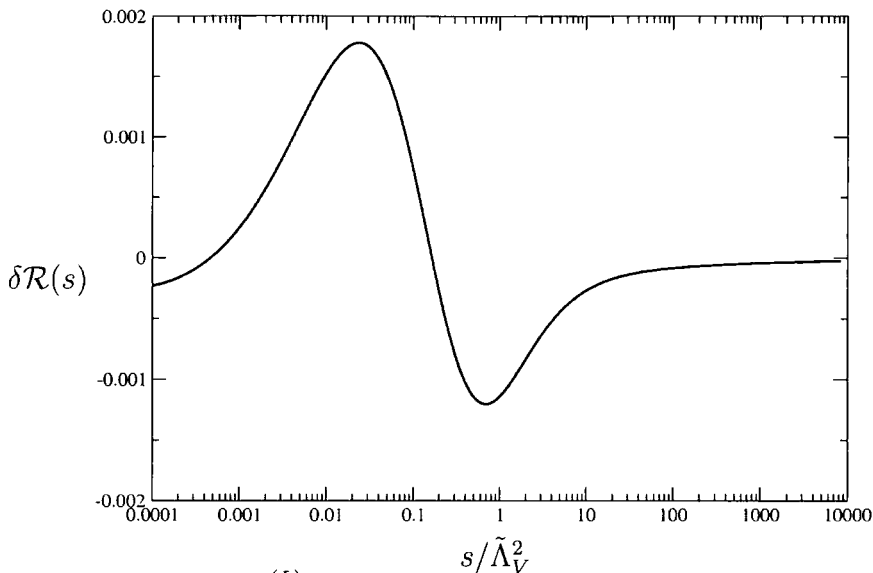
Figure 4.6: \delta\mathcal{R}(s) = \mathcal{R}_{CORGI}^{(L)}(s) - \mathcal{R}_{APT}(s) at the two-loop level for 2 flavours of quark.
