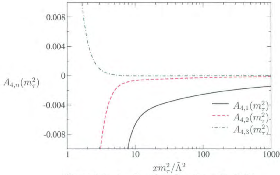
Figure 6.7: A_{4,n} from beta function in Eq.(6.28)
