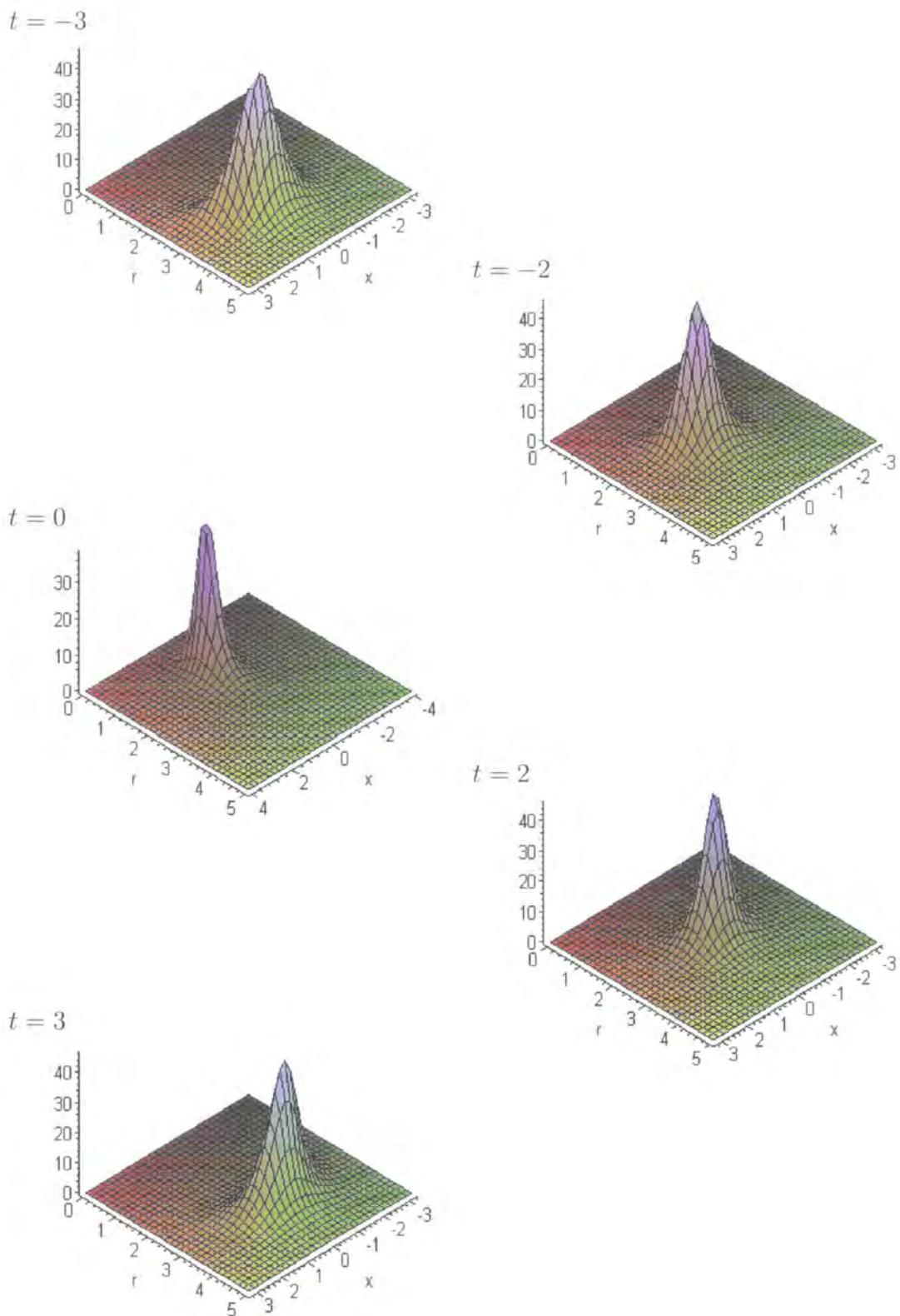
Figure 4.1: Example 4.4 — \|\Phi\|^2 for various values of t .
