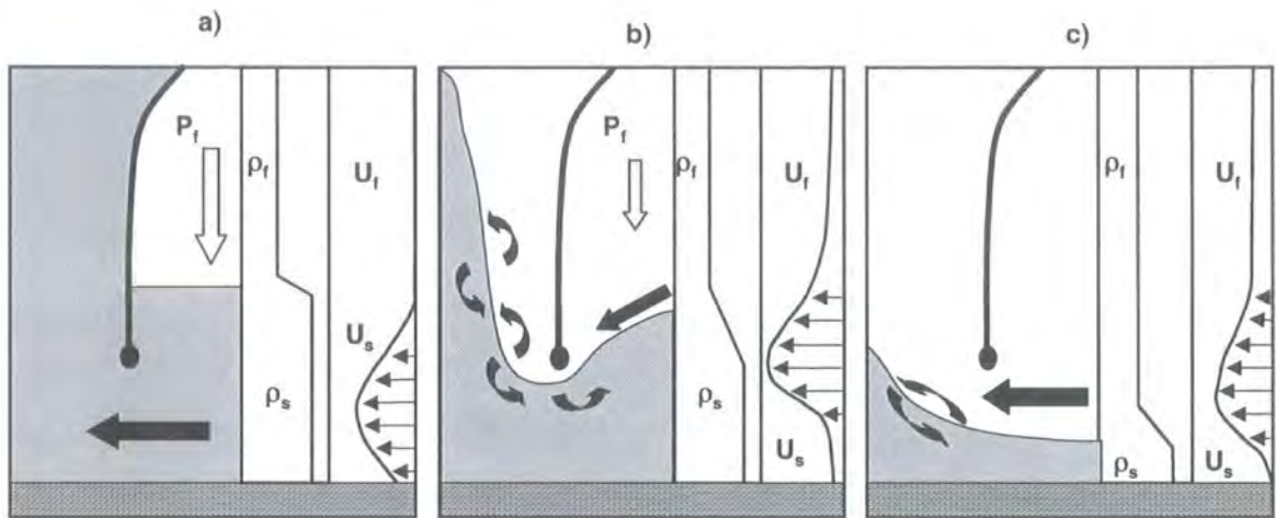
Figure 3-17 Interface at the baffle opening
