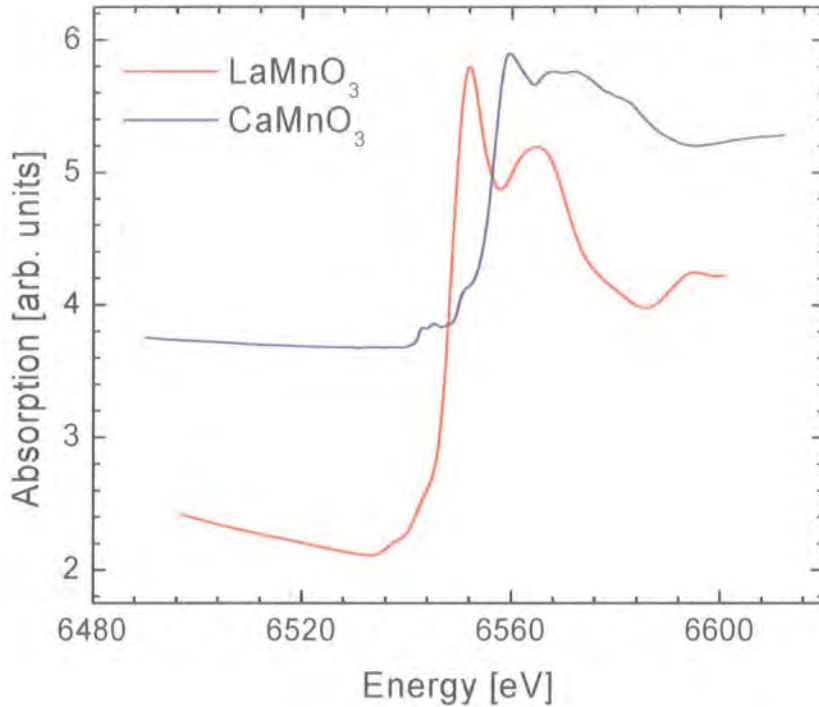
Figure 2.19: XAFS data for LaMnO 3 and CaMnO 3
