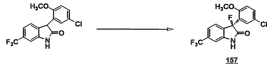
SCHEME 3.10
