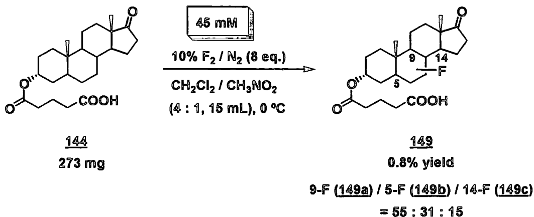
SCHEME 2.78
