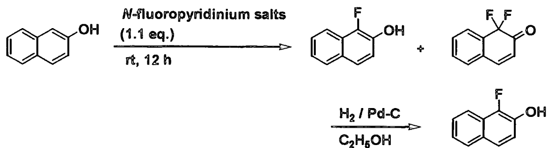
SCHEME 1.39
