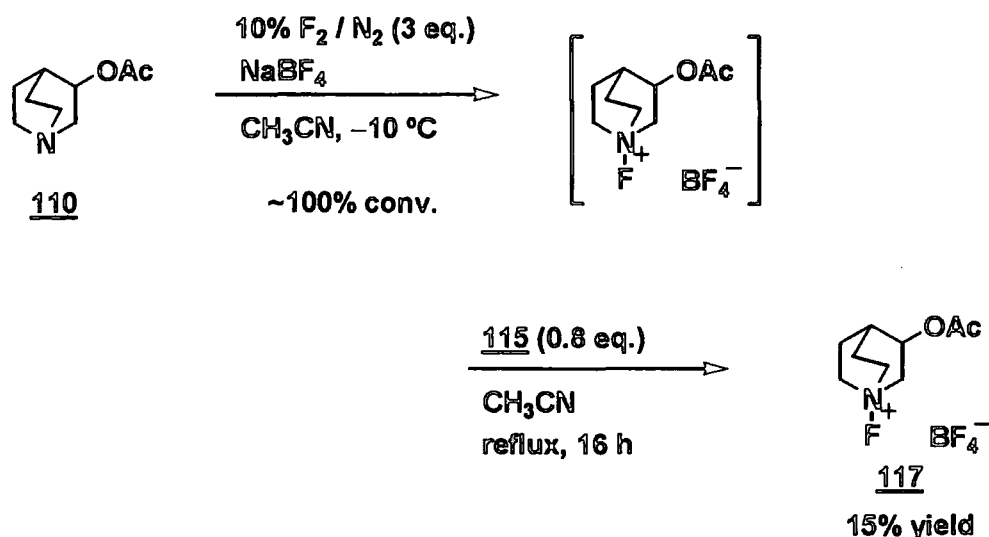
SCHEME 2.38
