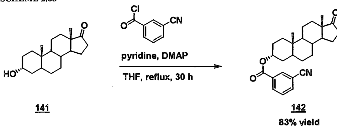
SCHEME 2.68
