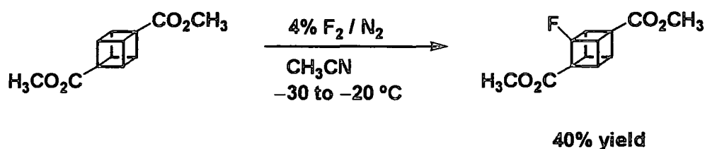
SCHEME 1.7
