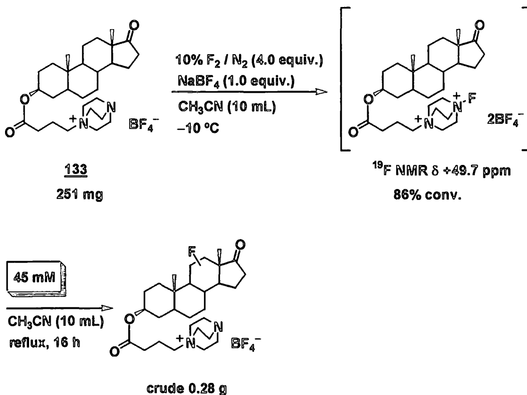
SCHEME 2.55
