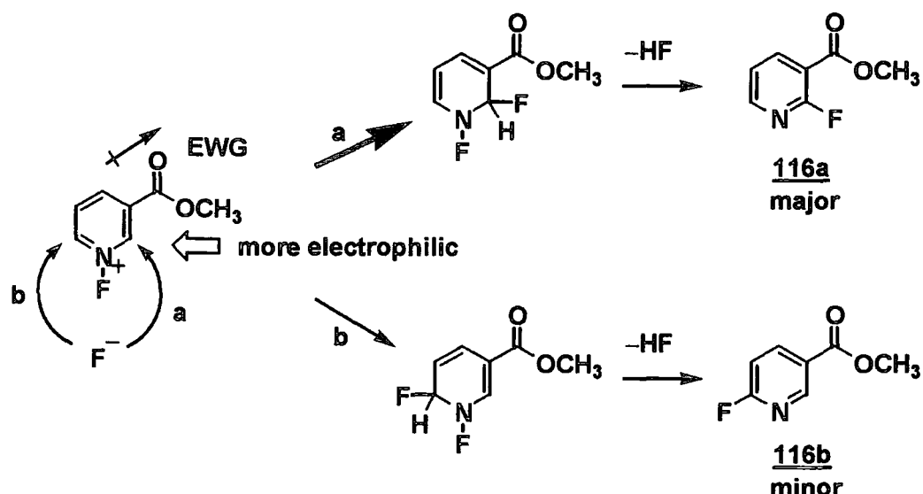
SCHEME 2.33
