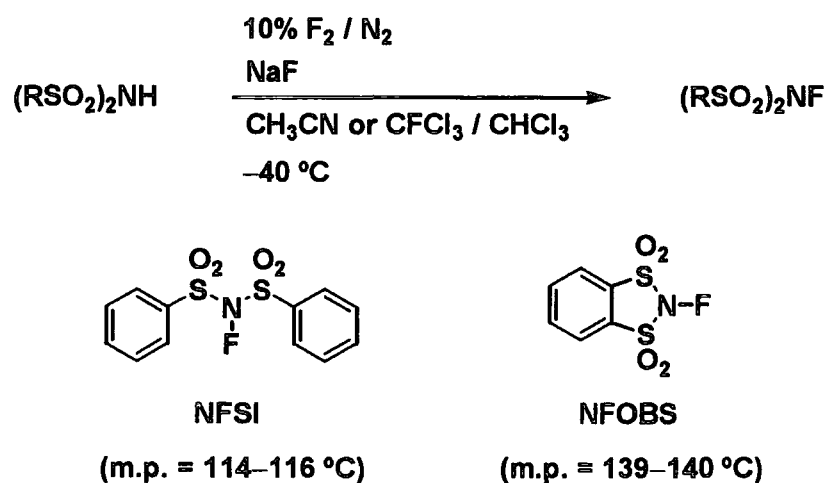
SCHEME 1.27
