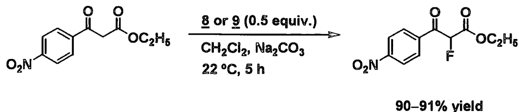
SCHEME 1.26
