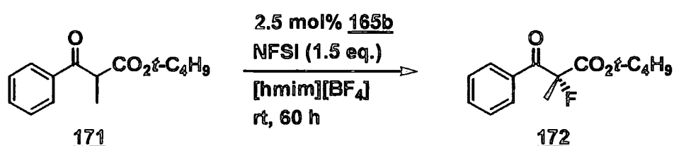
SCHEME 3.17
