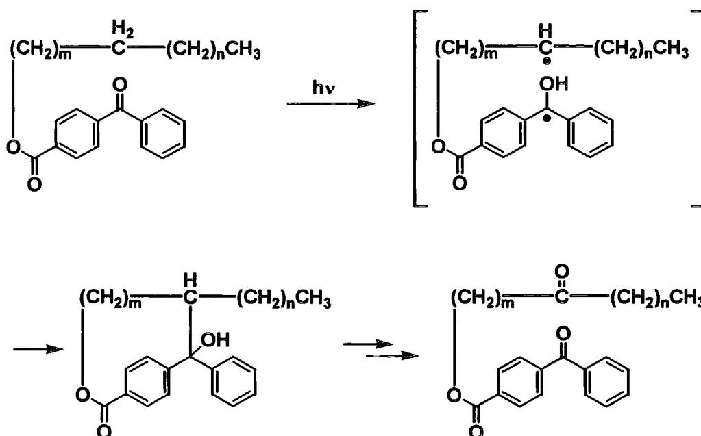
SCHEME 2.15
