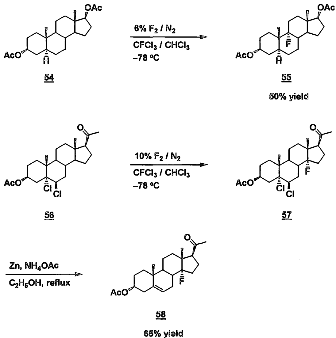
SCHEME 2.1
