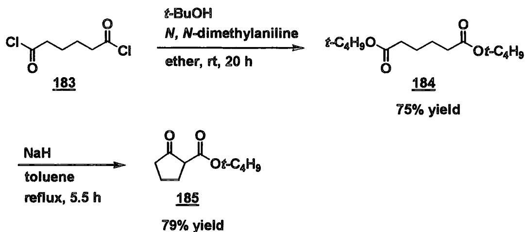
SCHEME 3.26
