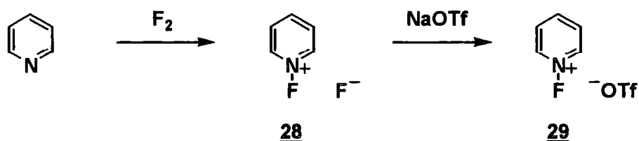
SCHEME 1.33
