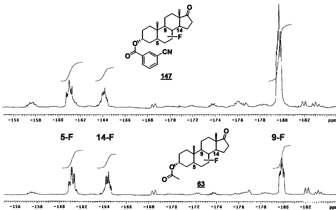
FIGURE 2.15 19 F NMR spectra of the crude products of the fluorination of compound 142 and 62
