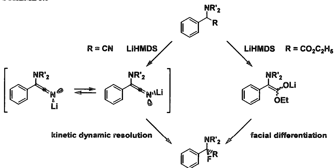
SCHEME 3.8
