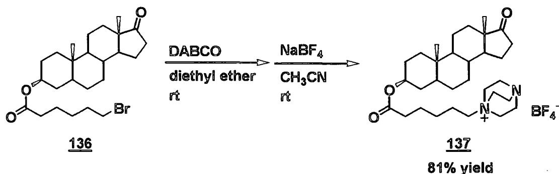
SCHEME 2.50
