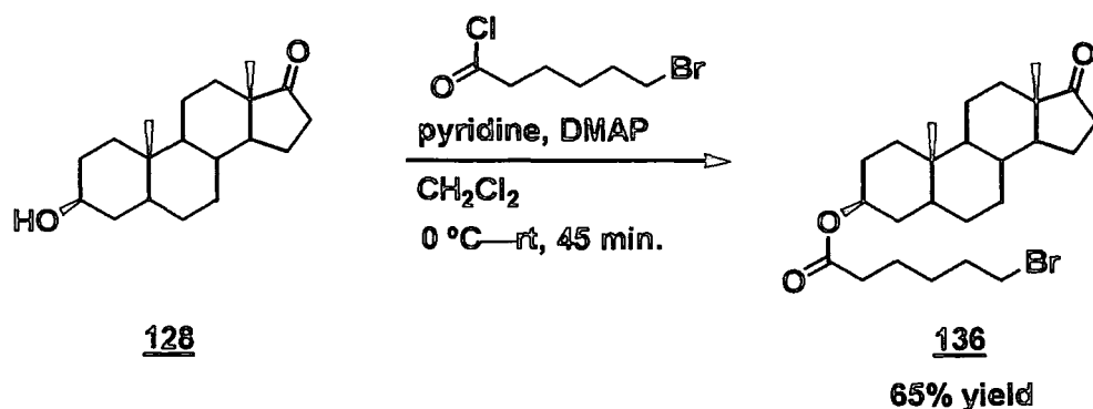
SCHEME 2.49
