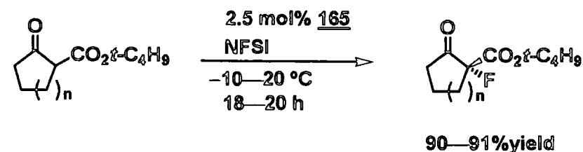
SCHEME 3.14
