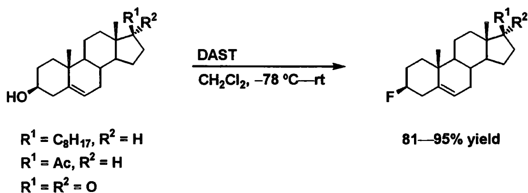
SCHEME 2.12
