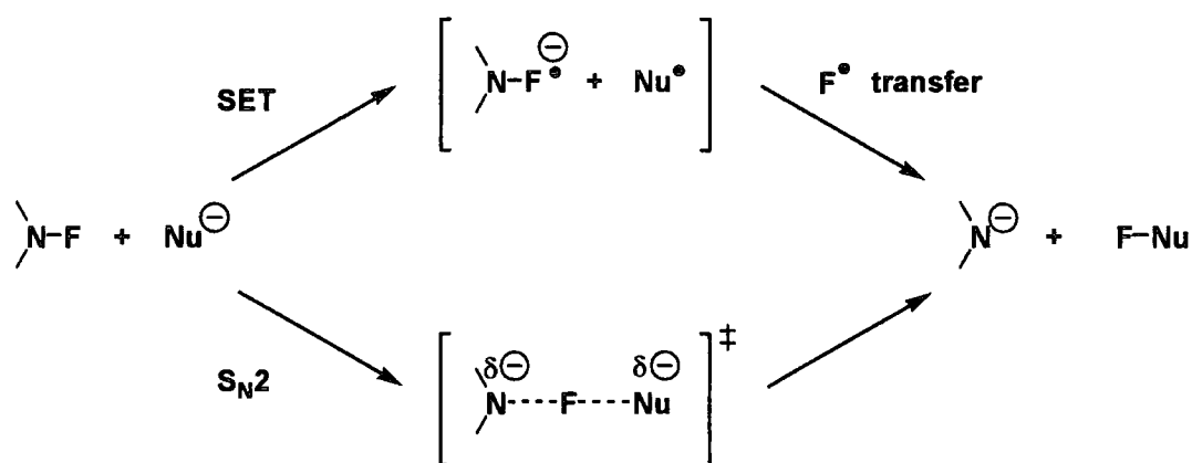
SCHEME 1.48
