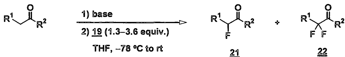
SCHEME 1.32
