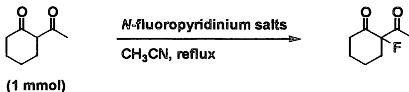
SCHEME 1.35
