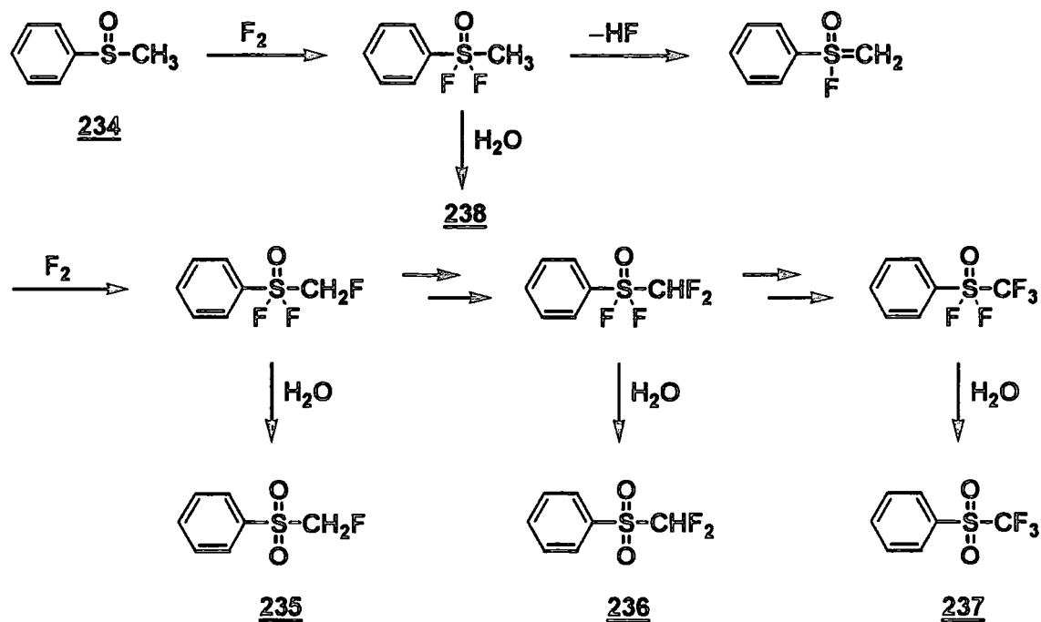
SCHEME 5.10
