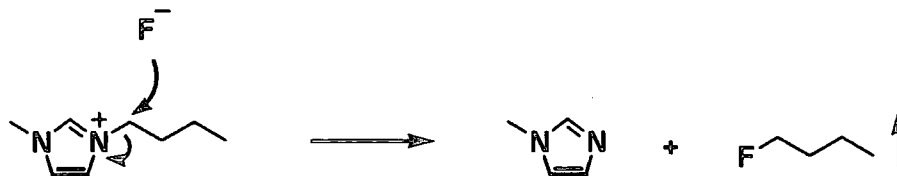
SCHEME 5.7
