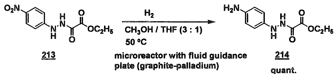
SCHEME 4.8
