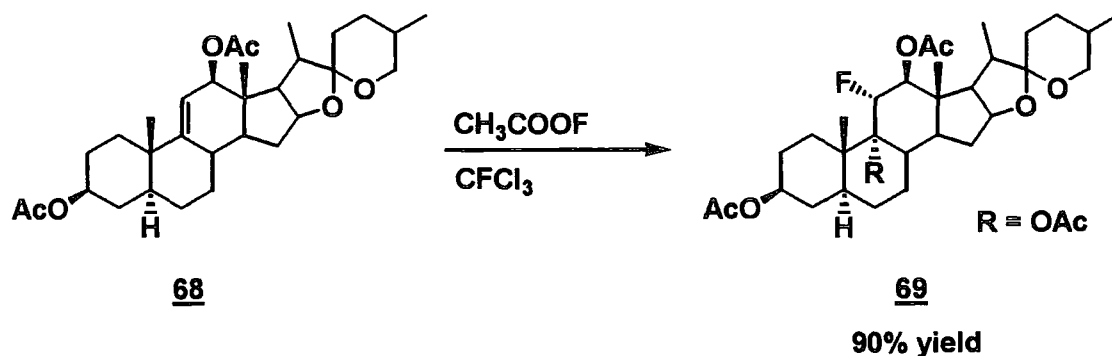
SCHEME 2.7
