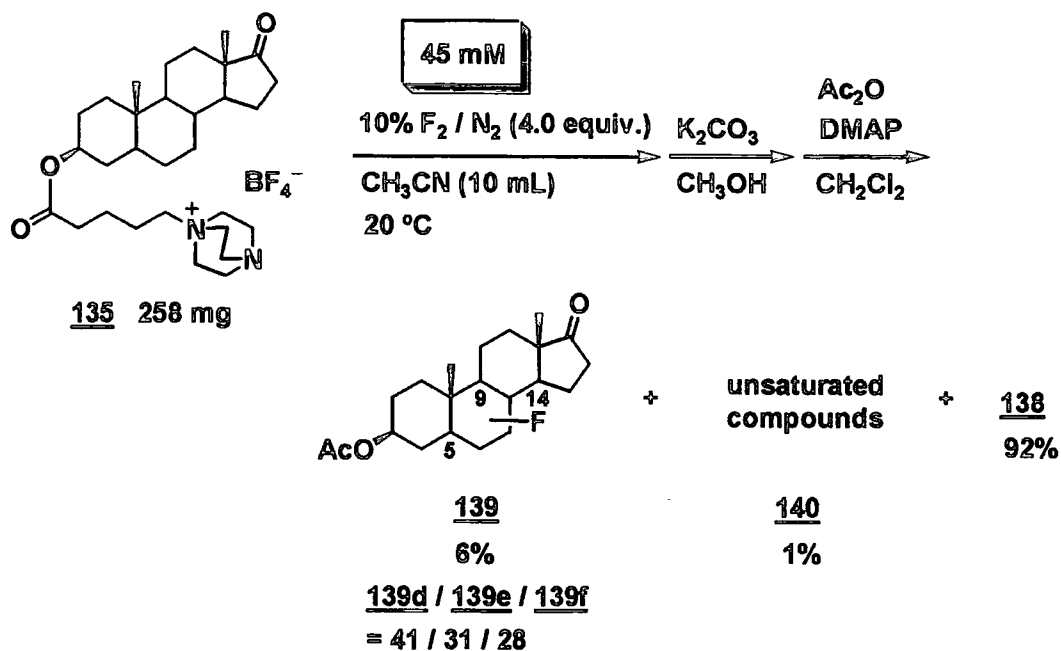
SCHEME 2.75
