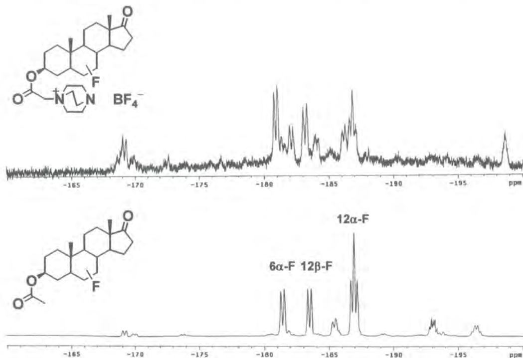
FIGURE 2.9 ^{19}\text{F} NMR spectra of crude products of fluorination of 138 and 131 .
