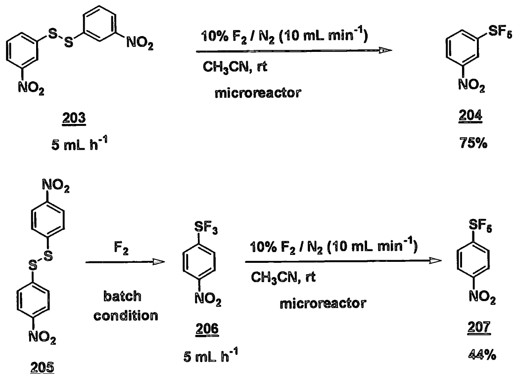
SCHEME 4.2
