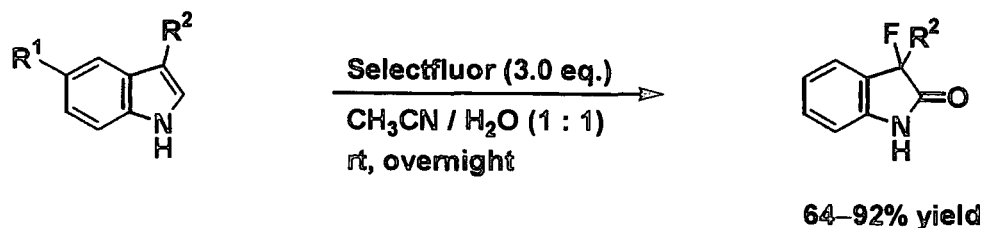
SCHEME 1.42
