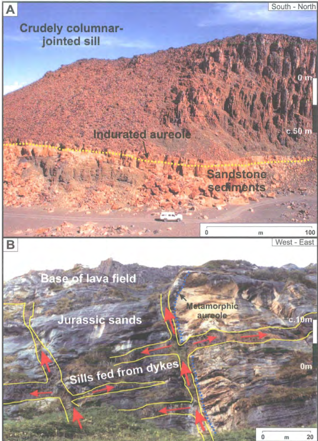
Figure 4-6 Sills and feeder dykes. A: A thick sill in the Etendeka flood basalts, Namibia. These picritic sills lie at the base of the Etendeka CFB stratigraphy and severely bake the aeolian and fluvial sandstones beneath; B: Feeder dykes in the cliffs of Carsaig Bay, Isle of Mull in the British Tertiary Igneous Province (BTIP). Metamorphic aureoles are evident where the Jurassic sands have been baked by the regular use of the conduits. Also note that the intruding sheets also intrude concordantly into the Jurassic sands as thin (<5m thick) sills.
