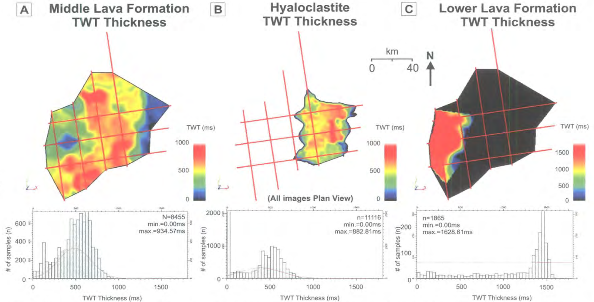
Figure 5-12 Two-way-time (TWT) thicknesses of major parts of the Faeroes succession in the GFA-99 data. A: The Middle Lava Formation (MLF) volcanics are absent in the north of the area, and thicken towards the East Faeroe High. To the East of the East Faeroe High, the MLF thins and the ULF forms a hyaloclastite volcanoclastic delta sequence on top of the MLF; B: The best defined hyaloclastite volume lies in the east of the study area in the Upper and Middle Formations where volcanoclastics have prograded into the area of the Corona Basin; C: The Lower Lava Formation (LLF) thickness in this figure, are estimated from the seismic data alone.
