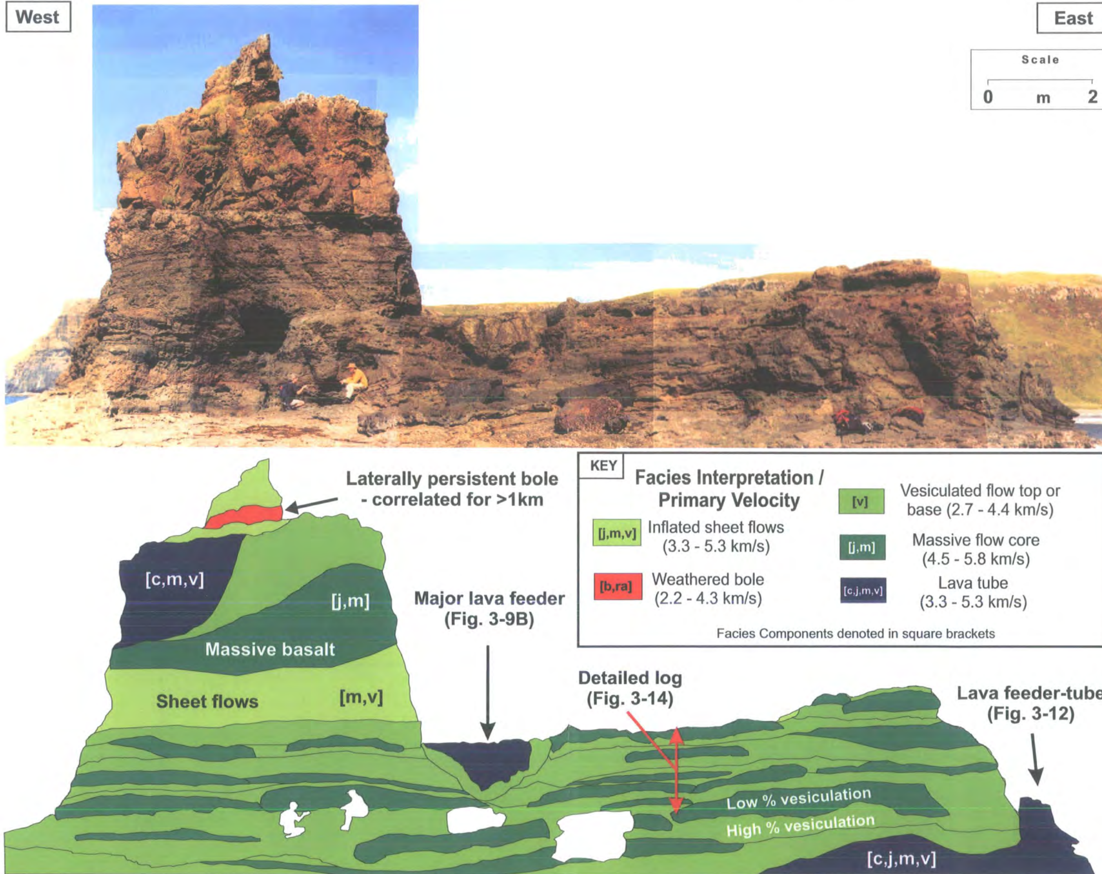
Figure 3-16 An Stac small sea stack section [NG 13117 82997] (Fig. 3-1B&C) showing lava feeders resident within the olivine-basalt succession. Lower in the outcrop it is possible to distinguish the individual massive and vesiculated zones which constitute the inflated pahoehoe. Higher up the section where the alternating zones are less obvious, they have been grouped under the inflated pahoehoe facies interpretation. Elastic velocity range estimates for geological intrafacies types are inferred from rock property data collated from the SIMBA rock property database and from Planke (1994) & Planke et al. (1999 & 2000). These inferred velocity ranges are tabulated in Table 3-2.
