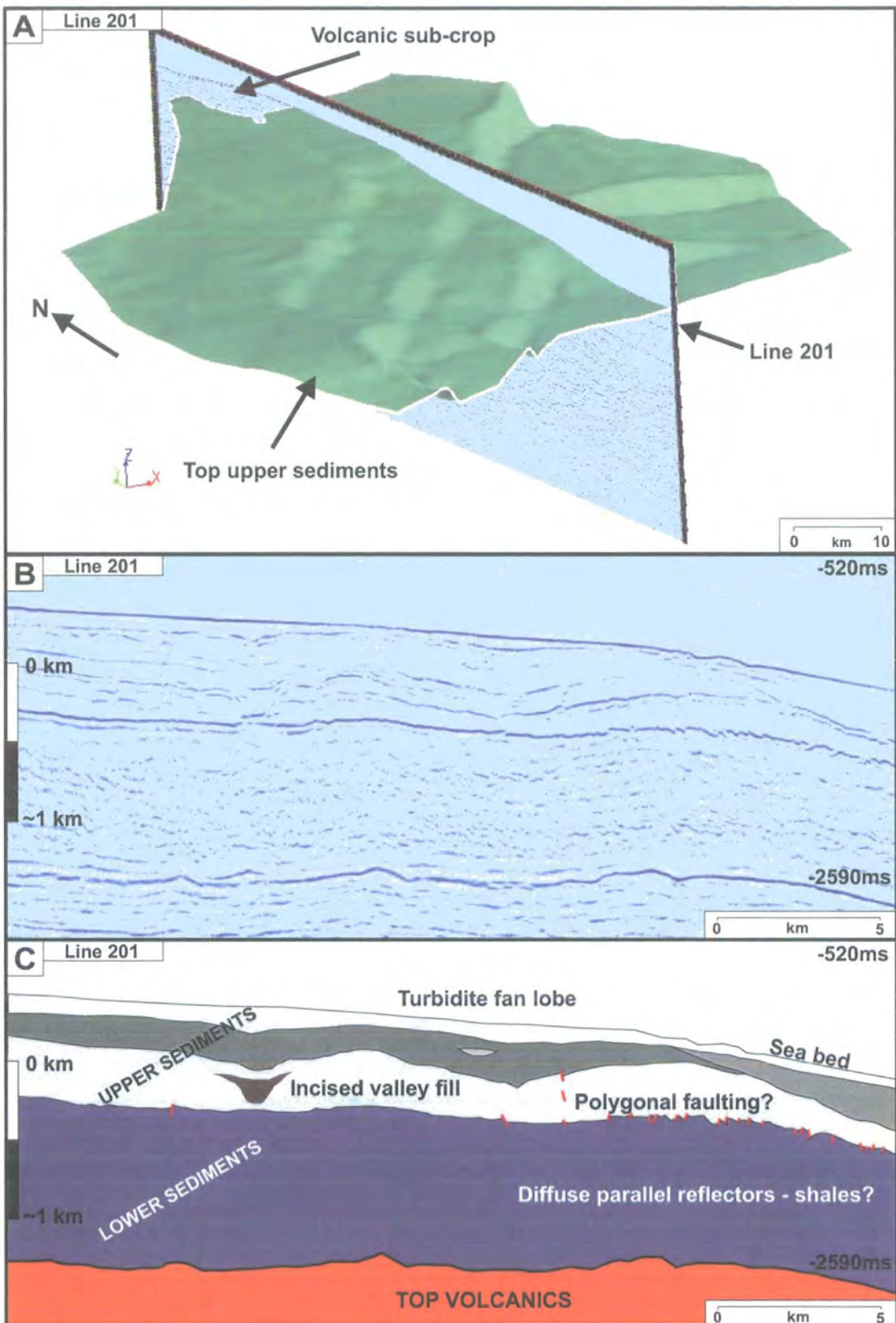
Figure 5-7 Post-volcanic sedimentary succession in the GFA-99 seismic dataset; A : The areal extent of the upper Sediments interpolated through the 2D data (green). Note the sub-crop is not sediments in the north of the image. Depth of Line 201 TWT section is 8 seconds; B : Close-up section of line 201; C : Interpretation of the upper and lower sediments in the same portion of line 201. Faults in the sedimentary sequence are marked in red. Vertical scale is in ms of TWT. Approximate scale in km is also stipulated.
