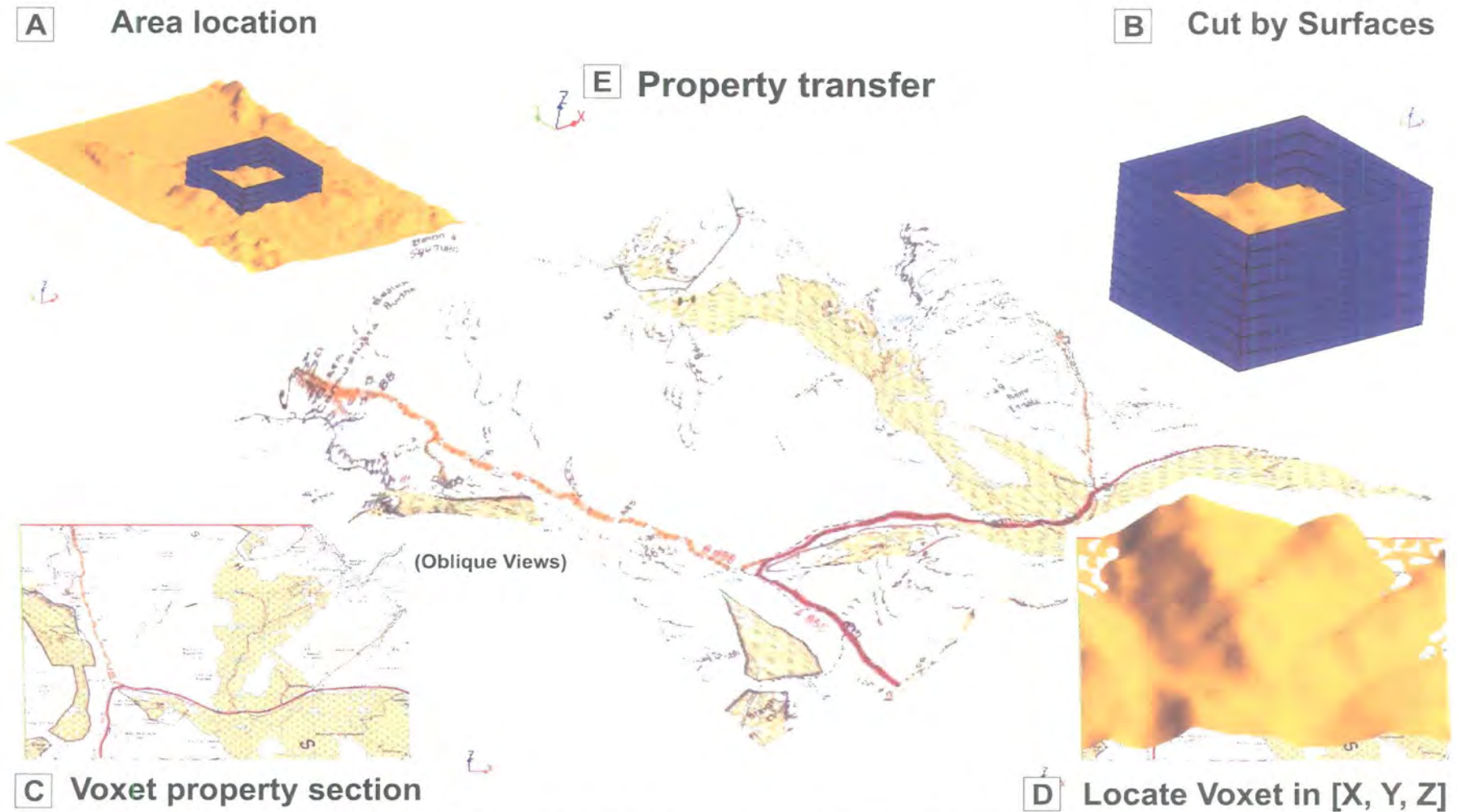
Figure 2-13 The creation of a property texture mapped Surface. A: The area on which the property texture is to be applied is selected from the DTM. A cutting Surface is built as a Tube through the topography; B: The DTM is reduced to the cut area; C: A Voxel property W-axis section is imported; D: The Voxel section is located precisely beneath the topographic Surface; E: The property section of the Voxel is transferred by vertical projection onto the DTM.
