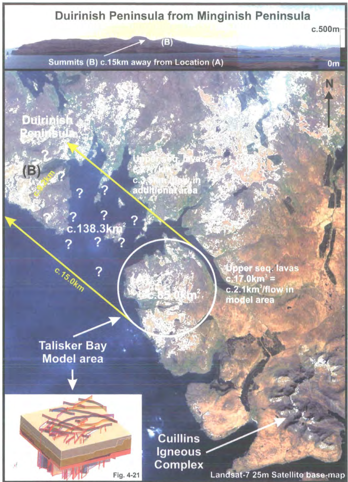
Figure 4-22 The peninsulas of Minginish and Durinish on the west coast of Skye showing the Skye Lava Field and estimates of potential lava volumes.
