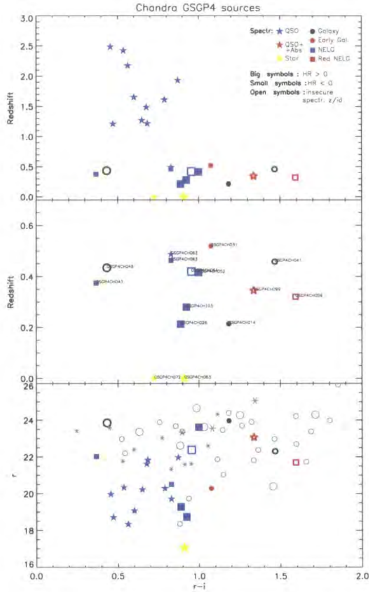
Figure 4.7: r-i colours against redshift and r band magnitude for sources in the GSGP4 field.
