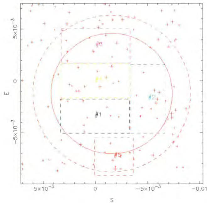
Figure 3.11: The WFC comprises four 4\text{ k} \times 2\text{ k} CCDs for the science array plus a thinned 2\text{ k} \times 2\text{ k} CCD for use as a dedicated frame transfer autoguider. The solid circle marks the unvignetted region while the dashed circle marks the 0.5 vignetting limit.
