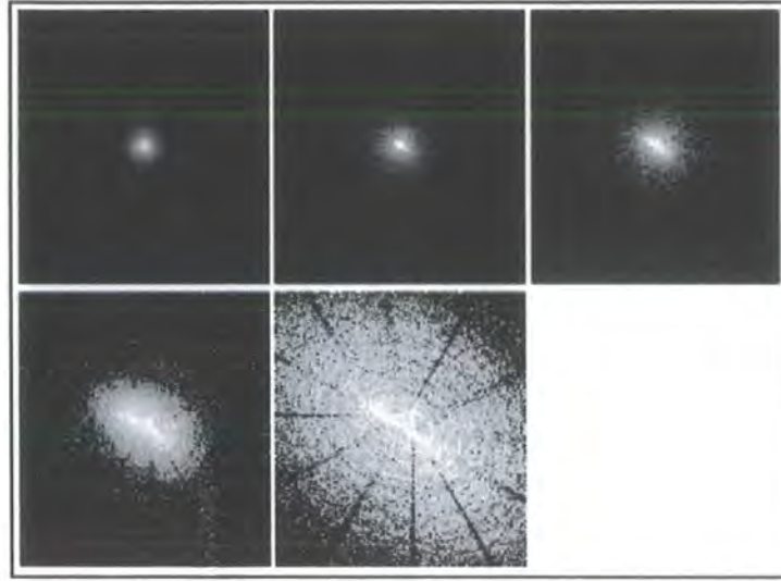
Figure 2.3: Simulated PSFs for the HRC-I instrument at 1.497 keV as a function of off-axis angles; clockwise from the top left, off-axis angles: 0, 1.5', 3', 12' and 6'. \text{FOV} \sim 0.5' . The point-spread function of the Chandra telescope depends on the spectral energy distribution of the source and location in the telescope field of view. Because of the Wolter type I design, the image quality is best in a small area centred about the optical axis. The on-axis PSF has a circular symmetry and the best resolution is achieved for photon energies around 0.277 keV, where the PSF can be approximated by a single Gaussian with 85% of the energy within less than 1". At lower or higher energies and at larger off-axis angles the resolution degrades. See also figure 2.4 which shows the 85% encircled energy diameter as a function of off-axis angle and energy. (From the CXO Detect Manual .)
