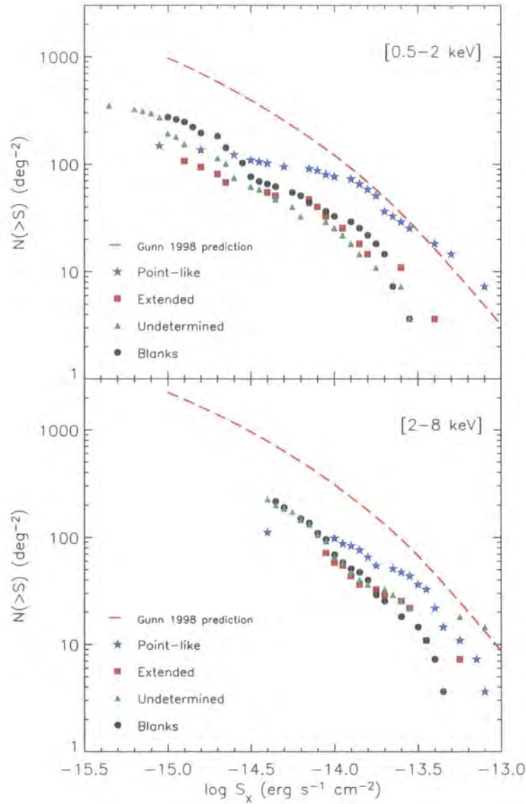
Figure 4.10: Soft (top panel) and hard (bottom panel) cumulative number counts for sources with stellar-like (blue stars) and extended (red squares) spatial distributions, for sources with unreliable stellarity index (“undetermined”; green triangles) and for undetected sources (“blanks”; black dots), according to their appearance in optical images of the WHDF, GSGP4 and F864 fields. The predictions from a XRB population synthesis model by Gunn (1999) have been included for reference.
