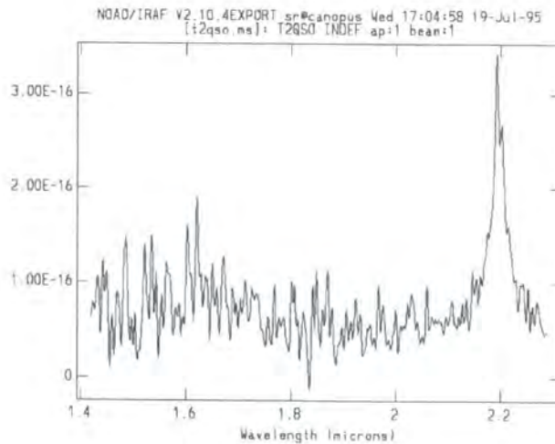
Figure 4.15: The UKIRT/CGS4 K -band spectrum of the type II QSO candidate RX J13433+0001, at z = 2.35 . The broad H \alpha indicates moderate obscuration. Obtained in March/May 1995.
