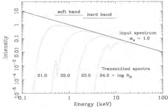
Figure 1.5: Absorption at x-ray energies for column densities of N_{\text{H}} = 10^{21} , 10^{22} , 10^{23} and 10^{24} \text{cm}^2 , derived using XSPEC. The incident spectrum is a power-law, I \propto \nu^{-\alpha_x} , with spectral index \alpha_x = 1 . From Gunn (1999).
