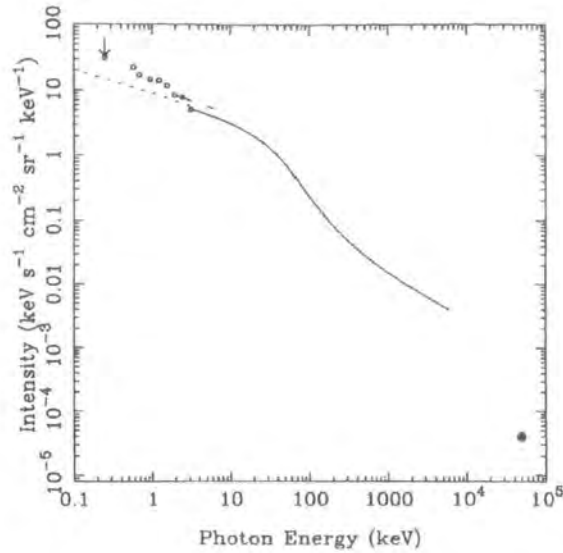
Figure 1.4: The XRB intensity spectrum I_{\epsilon} , from Fabian & Barcons (1992). In the 2–10 keV range, the XRB measurements can be fit by a power law of the form P(\epsilon) \equiv \frac{N}{\epsilon} = A\epsilon^{-\Gamma} , where P(\epsilon) is the photon intensity, \epsilon is the energy and the photon index has a value of \Gamma = 1.4 .
