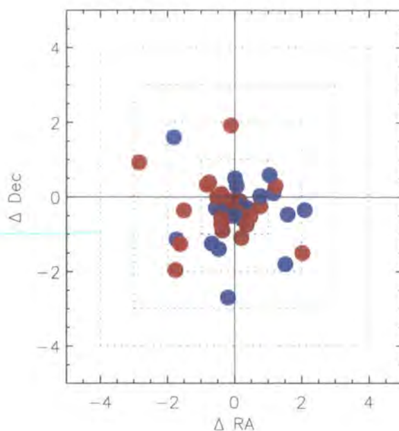
Figure 3.25: Offsets between SDSS and Chandra positions for the objects from table 3.13 in arcsec units. Fifty-one sources were found to match to better than three arcseconds.
