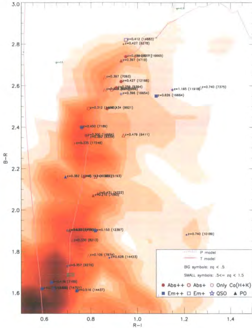
Figure 5.1: Colour-colour diagram of the red E/S0 galaxies studied. Early-type galaxies at redshifts below 0.5 are distributed in a narrow R - I gap with B - R colours redder than \sim 1.6 ; this region can be easily seen as the high surface density of galaxies in the background contour (constructed from all the R < 24 galaxies in the field). Bright sources on this colour-colour space were selected for our study; the plot shows them with a range of symbols: a) red circles indicate the presence of absorption lines in their spectra and the amount of fill denote the strengths of the lines; b) blue squares indicate narrow emission-lines in the spectra of the source and, again, filled for strong lines and shallow for weaker lines; c) blue stars denote the presence of broad lines; d) triangles are either absorption- or emission-line galaxies and, in that case, their colour serves as the discriminant. Each source is labelled with its redshift and its R -band catalogue number. In the plot there are as well two evolutionary tracks for early-type galaxies based on Bruzual & Charlot (2003) single stellar population synthesis models.
