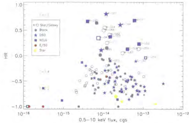
Figure 4.12: Hardness ratio with optical identification for sources in the WHDF and 10 \times 10 ks surveys. The legend is as for figure 4.1 with the addition of grey circles for x-ray sources without optical counterpart (“blanks”). Note the hardening of, not only the extended population, but of the QSOs as well towards fainter fluxes. Also, the presence of a distinct population of bright and hard QSOs. (The labels for the hard fraction of sources denote survey id numbers.)
