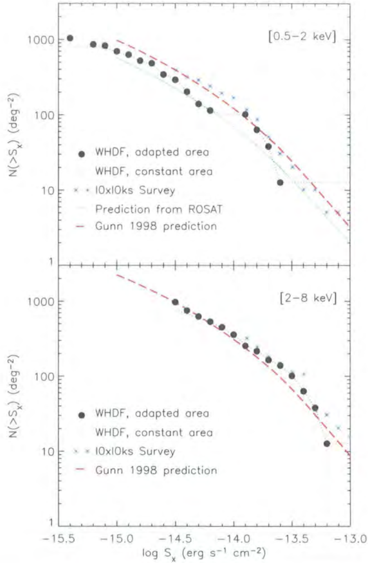
Figure 2.14: Cumulative source number counts per square degree for sources detected in the soft (top) and hard (bottom) band images, in the WHDF and 10 \times 10 ks surveys. The dotted line following the same distribution as the WHDF black dots are the number counts if the area of the survey is taken as constant as opposed to being a function of flux; we note that diverging effects are only observed at the faintest limits. Plotted as a thin green line in the soft band, an early prediction from ROSAT data is seen to underpredict the counts. On the other hand, the predictions from Gunn (1999) fit the data in both bands very well (red thick dashed line).
