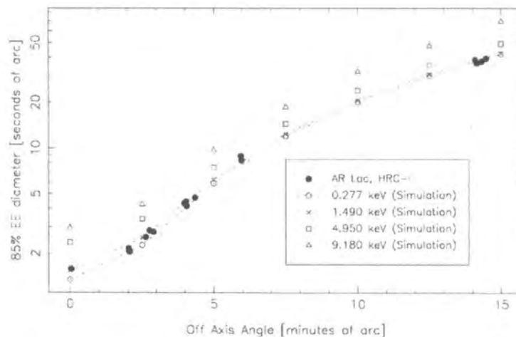
Figure 2.4: Observed and simulated 85% encircled energy diameters from Jerius et al. (2000).
