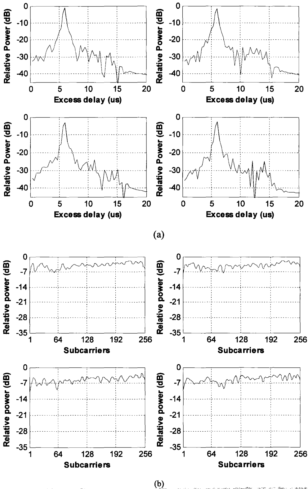
Figure 6.10 (a) Examples of channel impulse responses, (b) their corresponding channel transfer functions.
