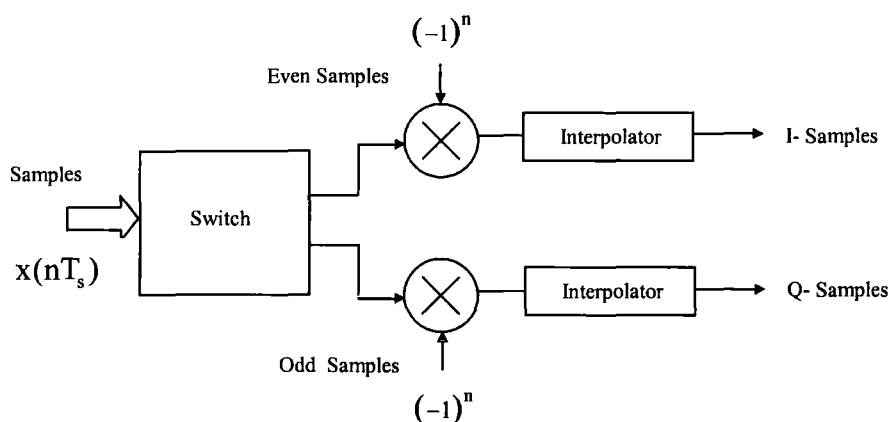
Figure 3.20 Block diagram of double Nyquist digital product detector.
