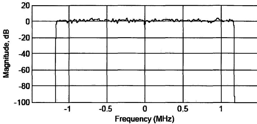
Figure 5.17 Measured spectrum for one OFDM symbol of IEEE 802.16-2004 system implemented in SIMULINK.
