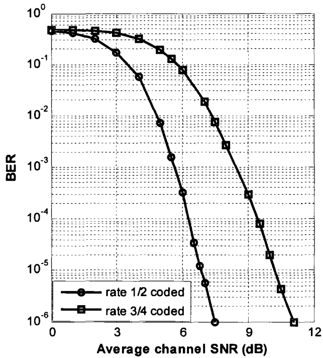
Figure 6.3 BER performance of rate 1/2 and 3/4 coded 256 OFDM IEEE 802.16-2004 WirelessMAN in AWGN channel employing QPSK.
