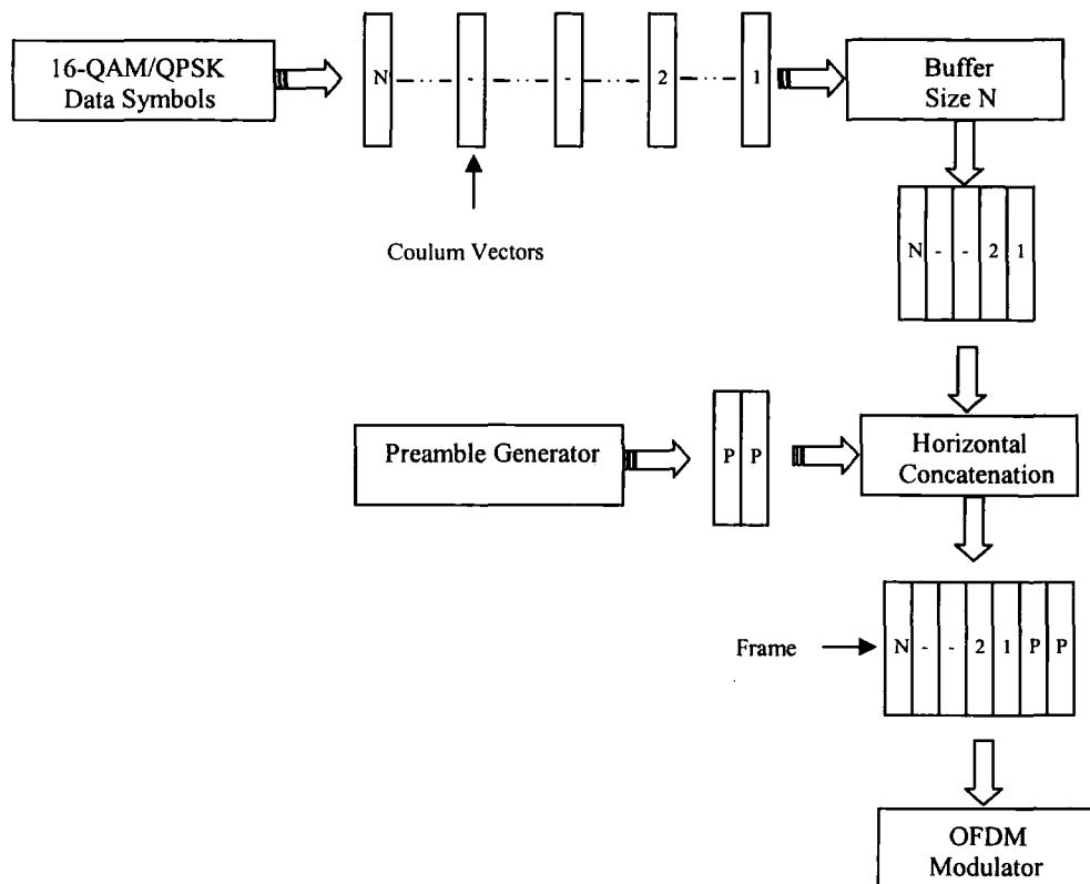
Figure 5.22 Process of frame formulation and preamble attachment
