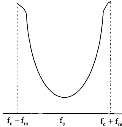
Figure 2.7 Doppler spectrum for Parson's model
