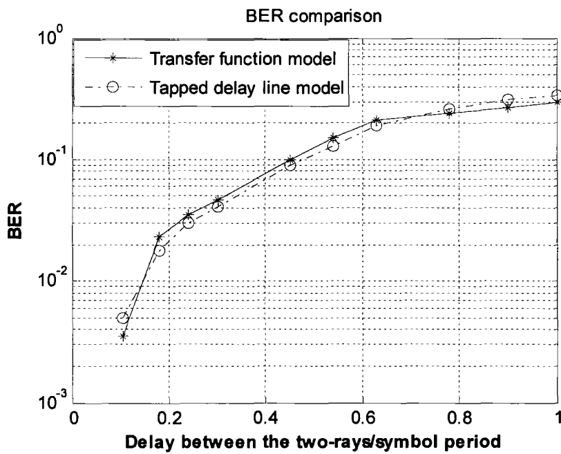
Figure 4.19 BER comparison for transfer function model and tapped delay line model. The delay between the two rays is 3 \mu\text{s} .
