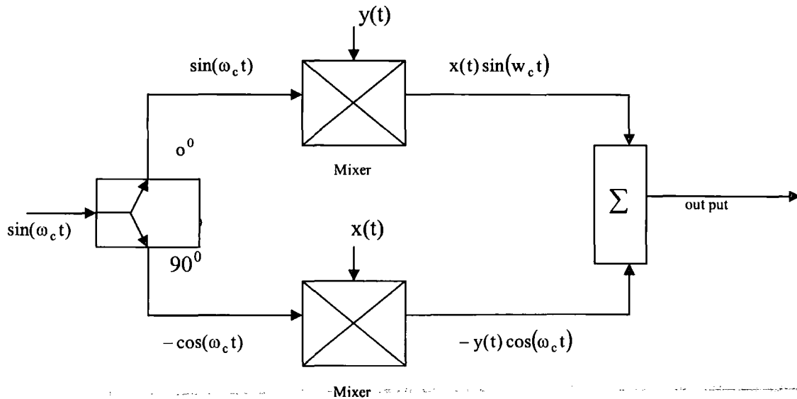
Figure 3.11 Rayleigh fading generator
