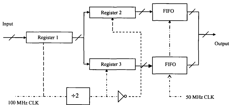
Figure 3.22 Application of demultiplexing in digital delays
