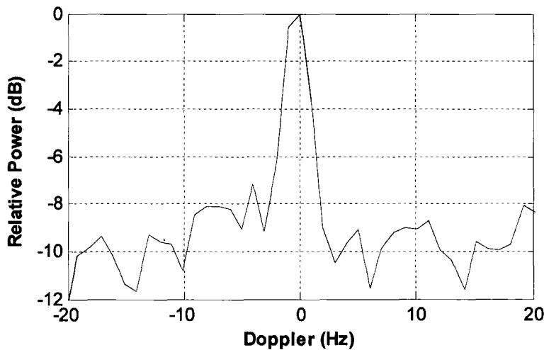
Figure 6.32 Average Doppler power spectrum of profile 4 for 2.5 GHz
