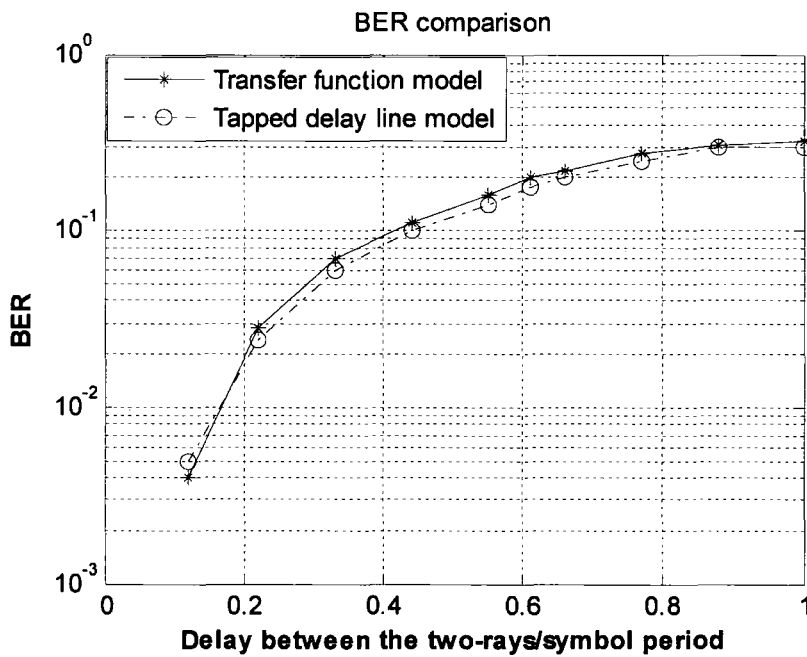
Figure 4.18 BER comparison for transfer function model and tapped delay line model. The delay between the two rays is 2.2 \mu\text{s} .
