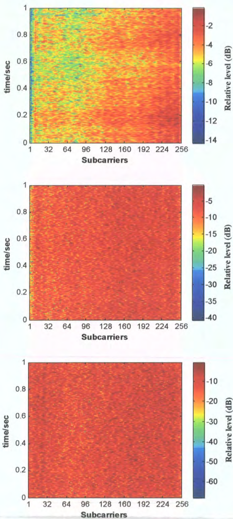
Figure 6.14 Time variant channel transfer functions of profile 1, 2 and 3 (top to bottom) for 3.5 GHz
