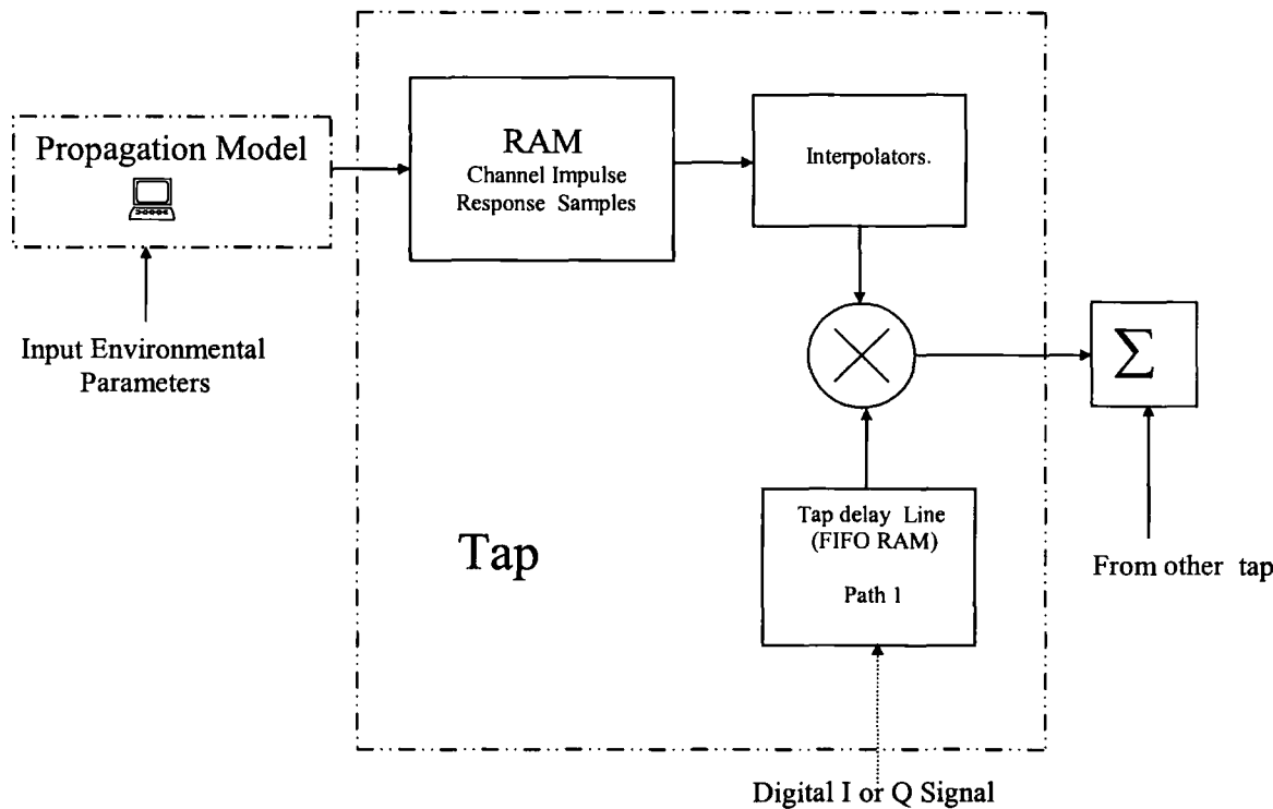
Figure 3.21 Functional diagram of each tap.
