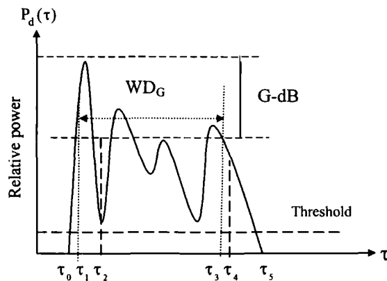
Figure 2.12 Profile width and delay window
