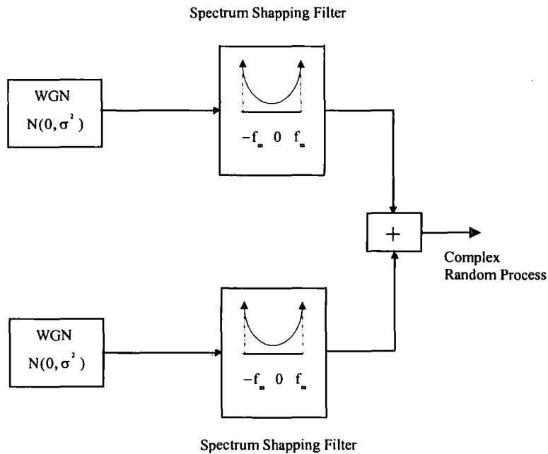
Figure 3.3 Filtered noise method of random process generation.
