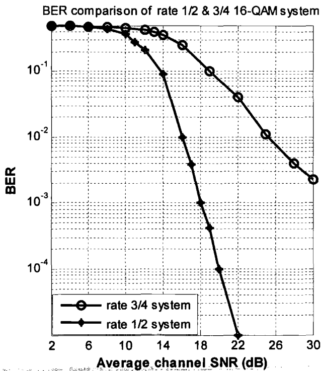
Figure 6.34 BER comparisons between rate 1/2 and 3/4 coded system employing 16-QAM in a measured channel profile 4 for 2.5 GHz band depicted in Figure 6.30.
