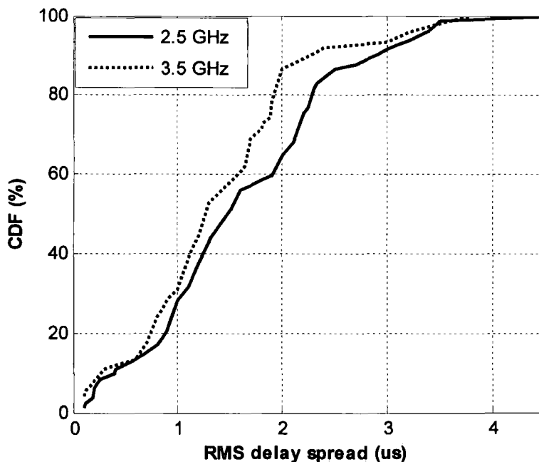
Figure 6.5 CDFs for the distributions of RMS delay spread for the 2.5 GHz and 3.5 GHz bands
