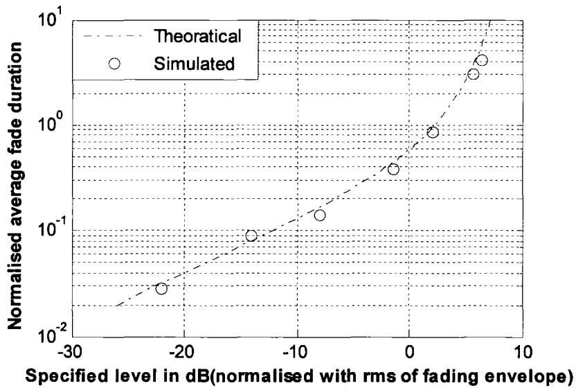
Figure 4.12 Comparison between the measured and theoretical average fade duration (afd) of the envelope of the simulated complex process with 40 Hz Doppler.
