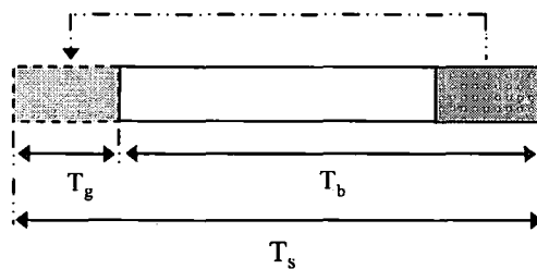
Figure 5.3 Description of cyclic prefix for OFDM symbol
