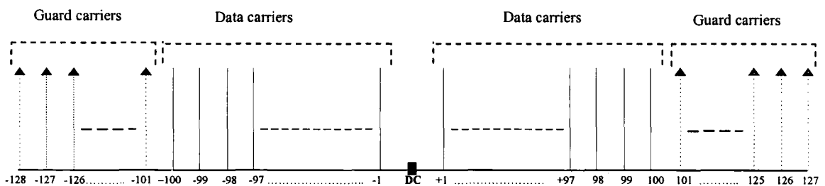
Figure 5.14 Frequency domain description of OFDM symbol.
