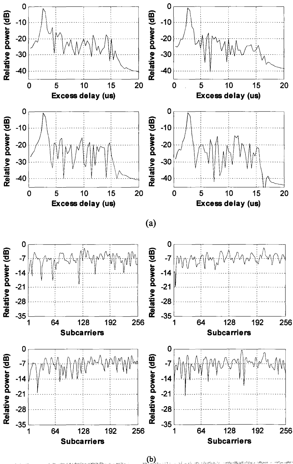
Figure 6.11 (a) Examples of channel impulse responses , (b) their corresponding channel transfer functions.
