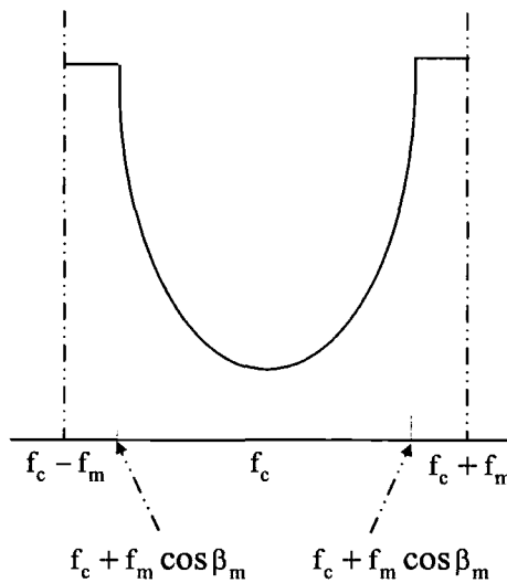
Figure 2.6 Doppler spectrum for Aulin's model
