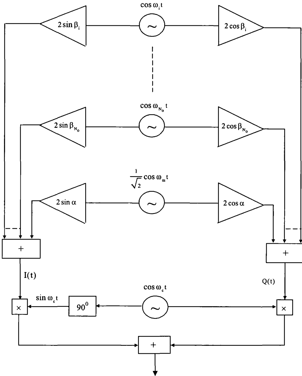
Figure 3.4 Jakes method of simulation
