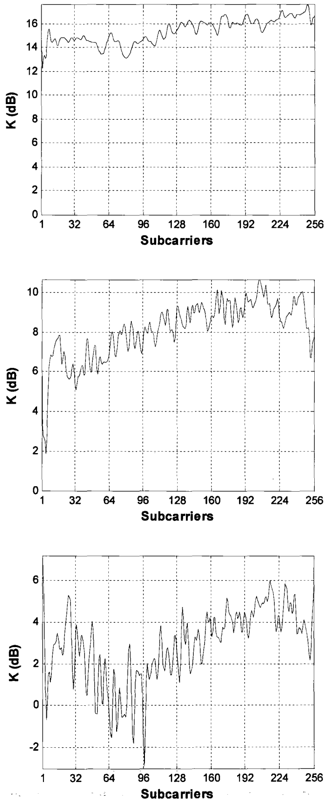
Figure 6.22 K-factor versus subcarriers for channel profiles 1,2 and 3 (from top to bottom) of 3.5 GHz
