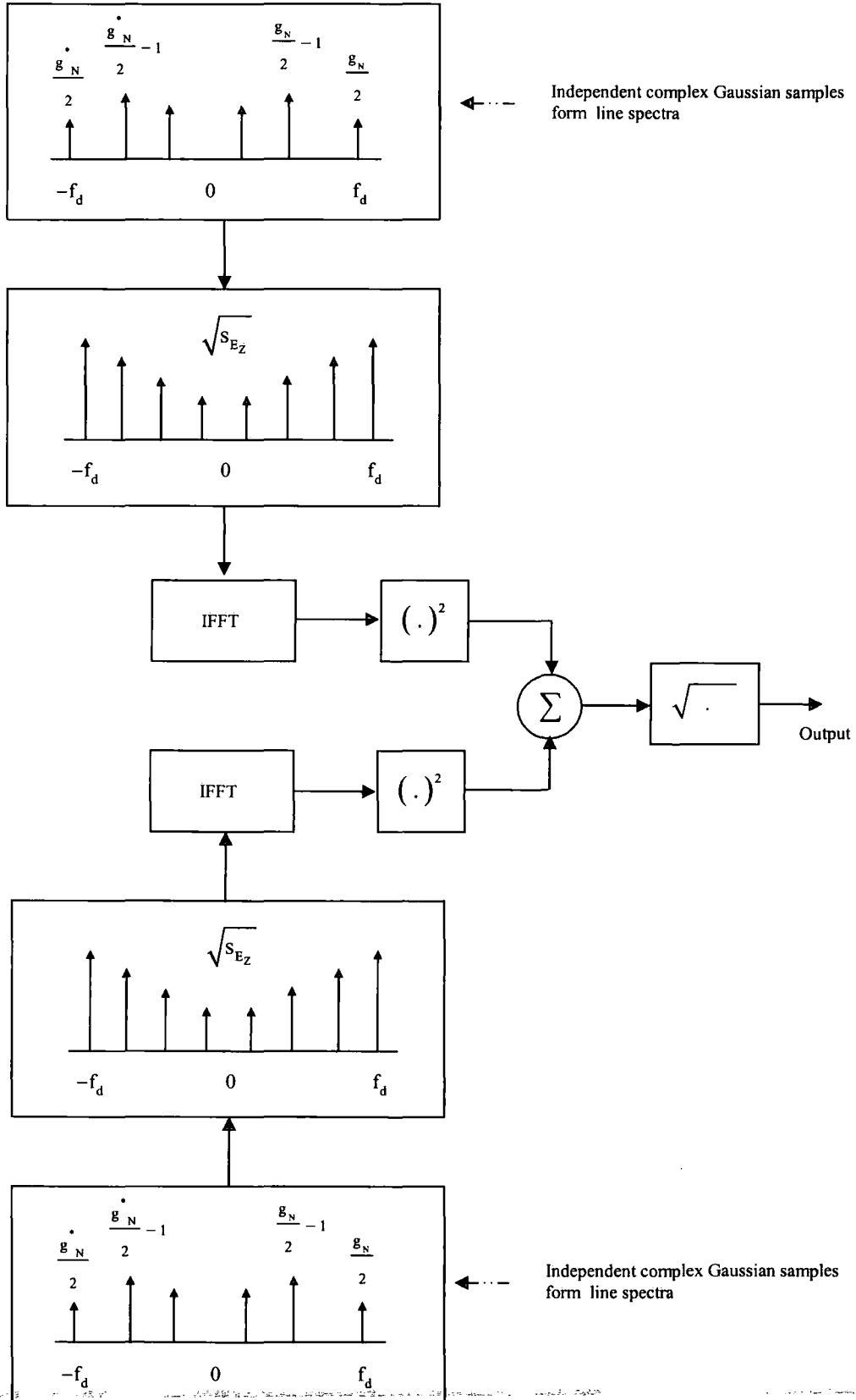
Figure 3.7 Frequency domain method of channel simulation.
