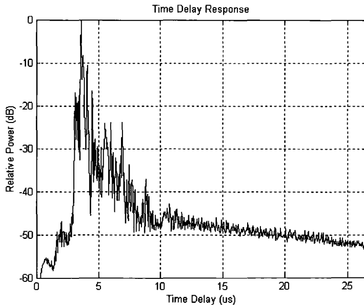
Figure 2.11 An example of a typical measured impulse response
