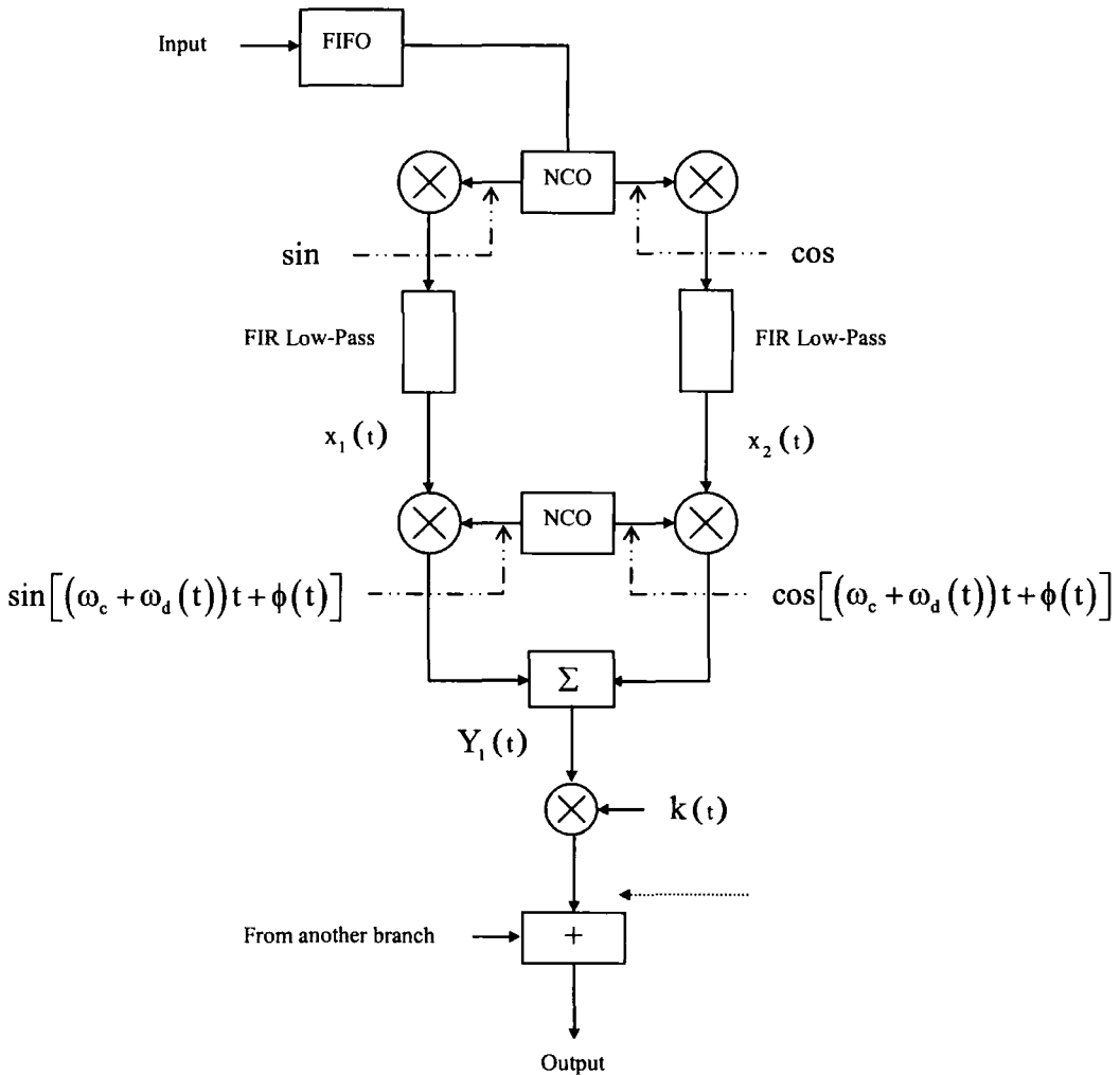
Figure 3.24 Channel simulator employing FIFO and NCO.
