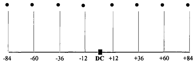
Figure 5.13 Positions of 8 pilots in the spectrum of OFDM symbol
