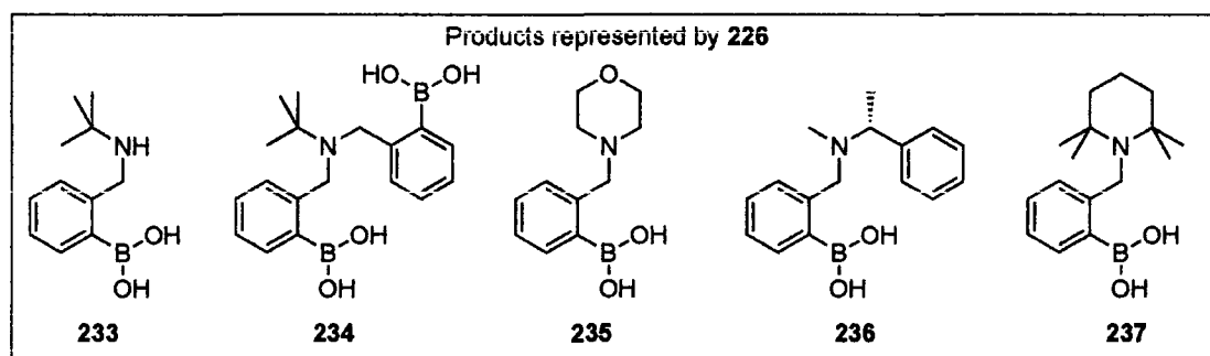
Scheme 21: Reductive amination route to series of N,N -benzylamine-2-boronic acids.
