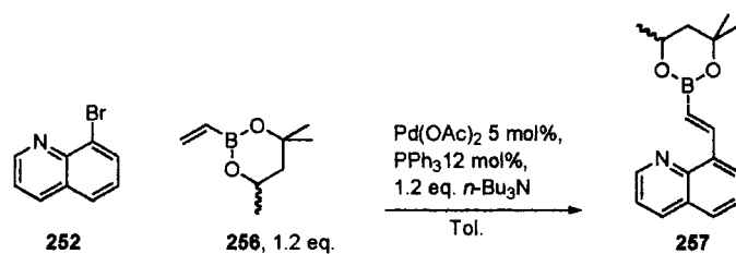
Equation 45: Attempted Heck coupling.
