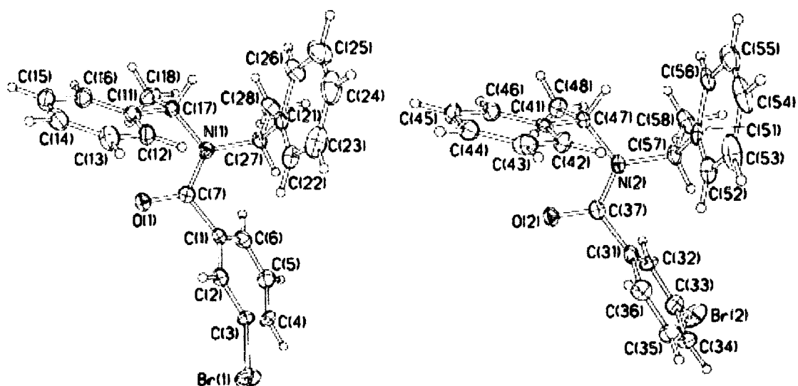
Figure 11: ORTEP X-ray crystal structure of bromide 250 , showing 50% probability ellipsoids.
