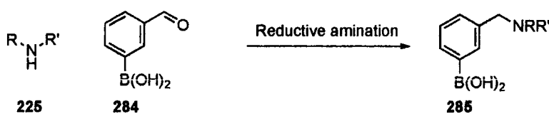
Equation 52: Route to N,N -dialkylbenzylamine-3-boronic acid series.
