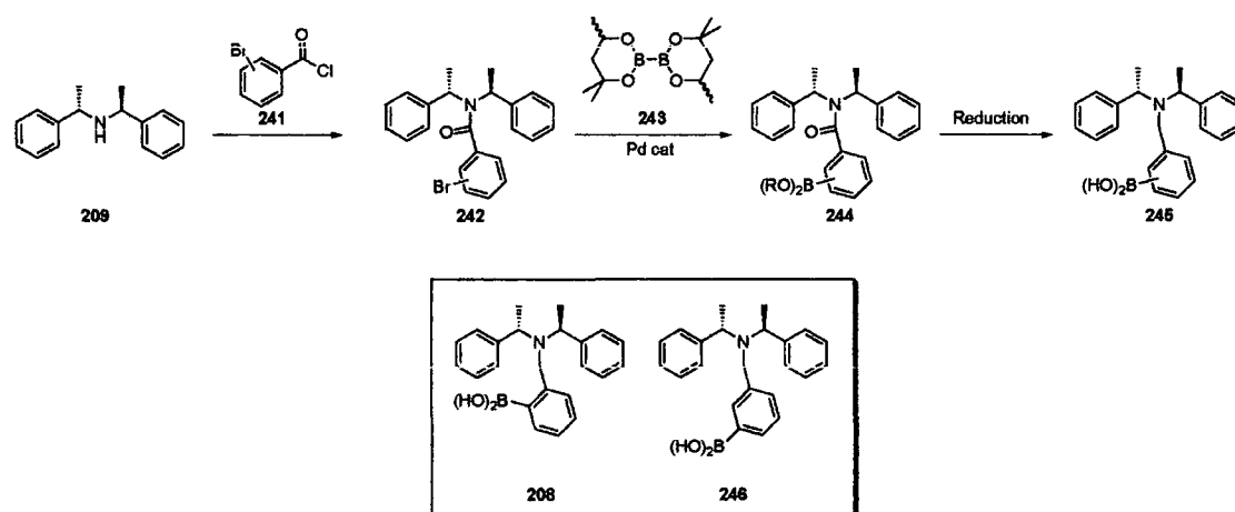
Scheme 23: Acylation-transmetalation-reduction route to benzylamine-2-boronic acids.
