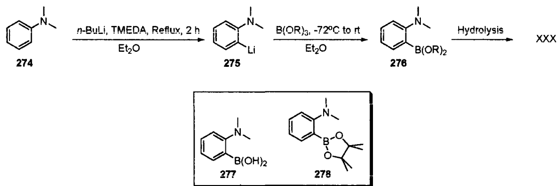
Scheme 28: Boronation of N,N -dimethylaniline.
