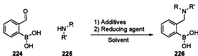
Equation 37: Reductive amination route to benzylamine-2-boronic acids.
