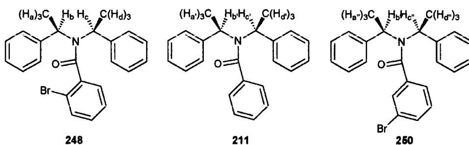
Figure 7: Proton labelling in (S,S)-(-)-bis( \alpha -methylbenzyl)amine]-N-benzylamine series.
