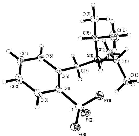
Figure 6: ORTEP X-ray crystal structure of trifluoroborate 207 , showing 50% probability ellipsoids. [139]
