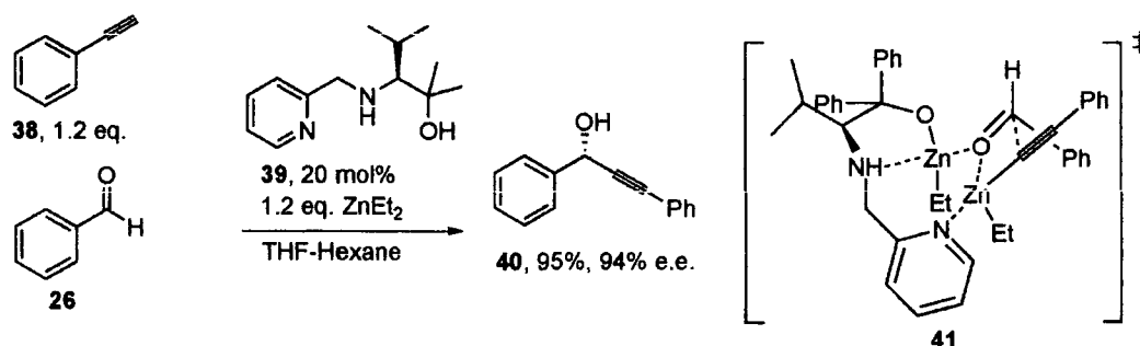
Equation 5: Asymmetric alkylation of aldehydes.
