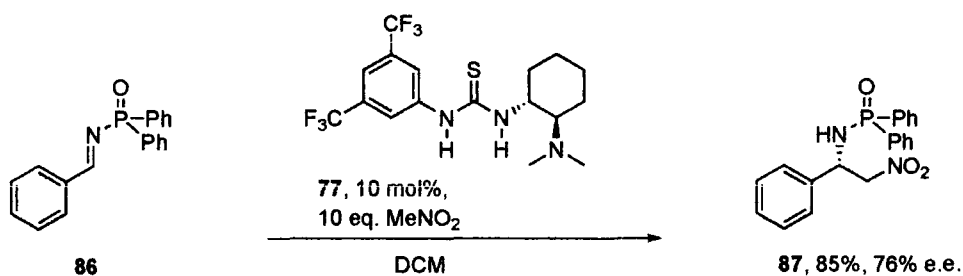
Equation 15: Bifunctional thiourea-catalysed aza-Henry reaction.
