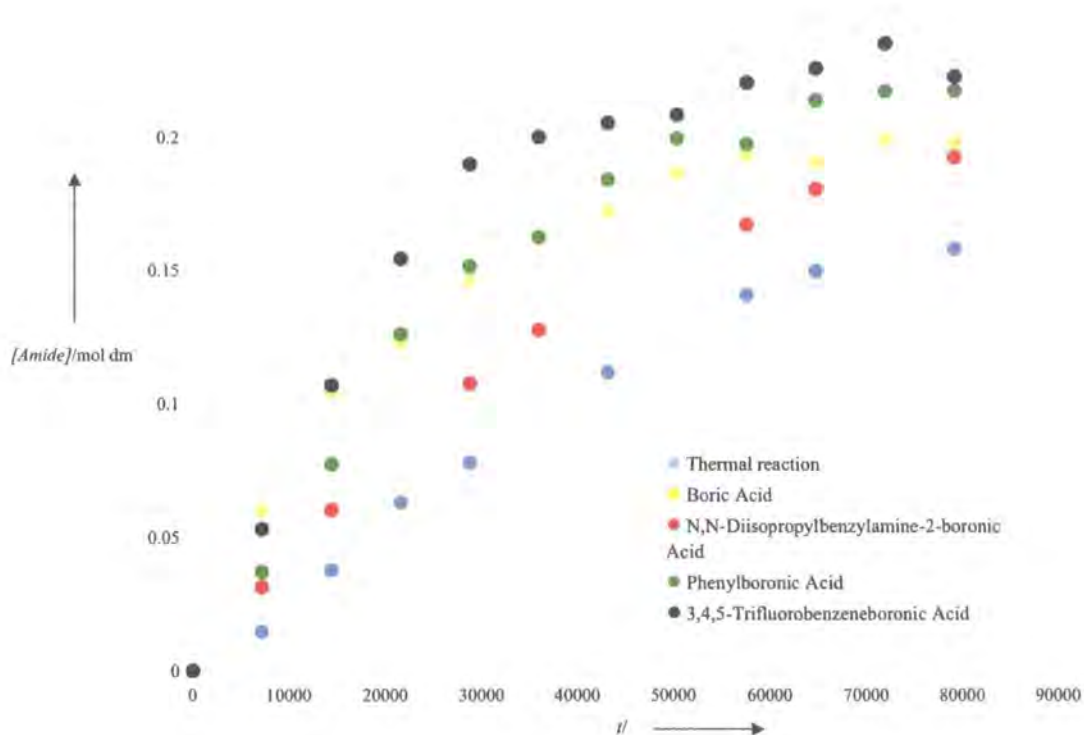
Chart 4: Formation of N -4-phenylbutyl-4-phenylbutyramide.
