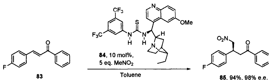
Equation 14: Bifunctional thiourea-catalysed Michael addition.
