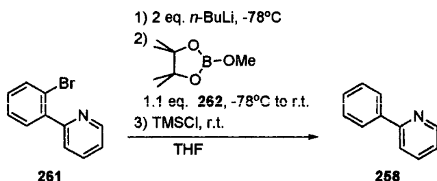
Equation 46: Attempted lithium-halogen exchange route to 2-phenylpyridine-2'-boronic acid series.
