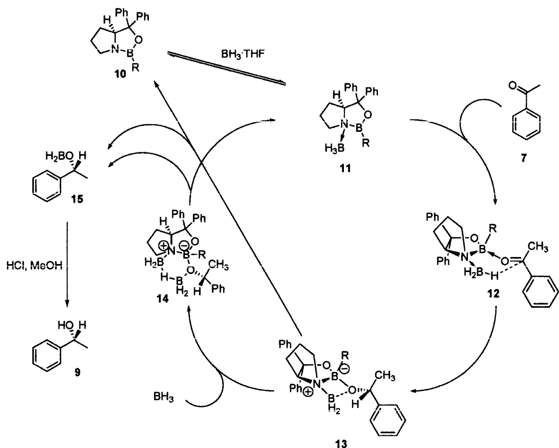
Scheme 1: Proposed reaction mechanism of the CBS reaction.
