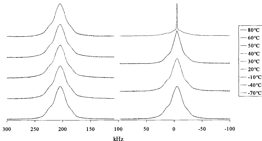
Figure 5.4: Proton bandshapes obtained from the last spectrum of the T_1^{\text{H}} array at different temperatures for amorphous nifedipine. The horizontal scale is for reference only.
