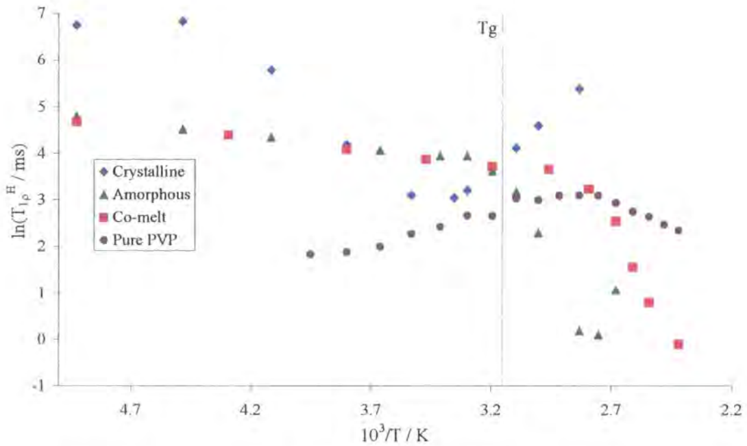
Figure 6.14: Comparison of the T_{1p}^H curves obtained for crystalline and amorphous indomethacin, PVP/indomethacin co-melt and pure PVP.
