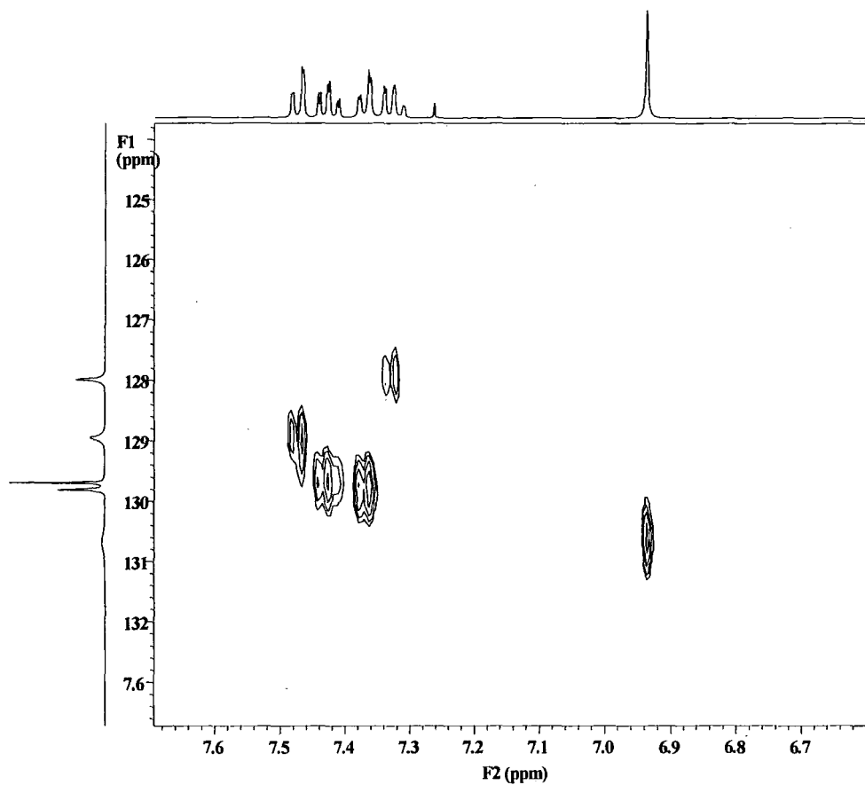
Appendix 10: HSQC spectrum of carbamazepine, in \text{CDCl}_3 , showing the high-frequency part.
