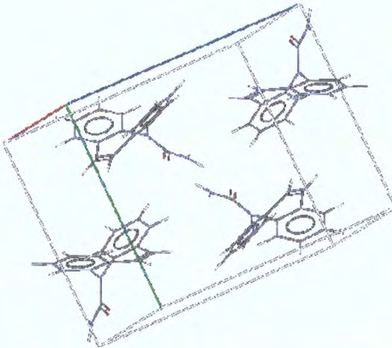
Figure 3.16: Unit cell of modification III of carbamazepine.
