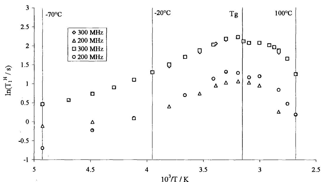
Figure 5.6: T_1^{\text{H}} measurements for amorphous indomethacin. The maximum is observed at T_g ( 45^\circ\text{C} ).
