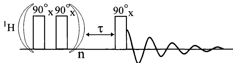
Figure 1.7: The pulse sequence for a saturation-recovery experiment.
