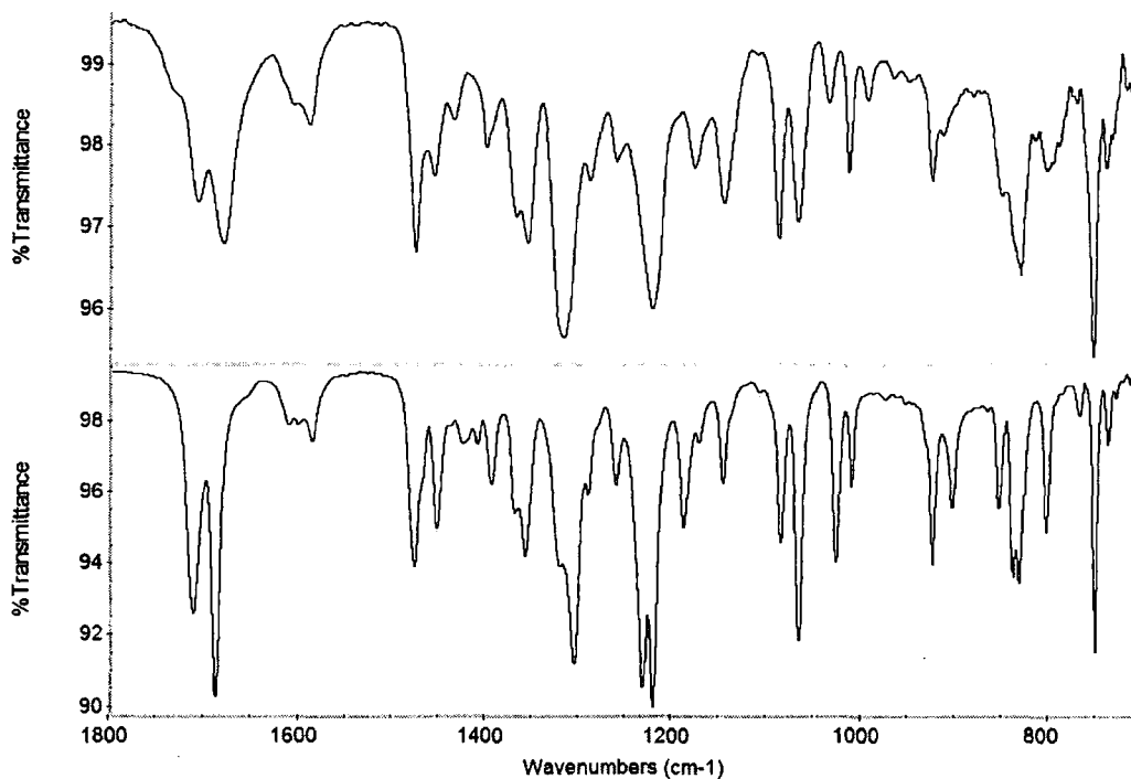
Figure 4.3: FTIR spectra of amorphous (top) and crystalline (bottom) indomethacin, showing only the 700-1800 \text{cm}^{-1} region.
