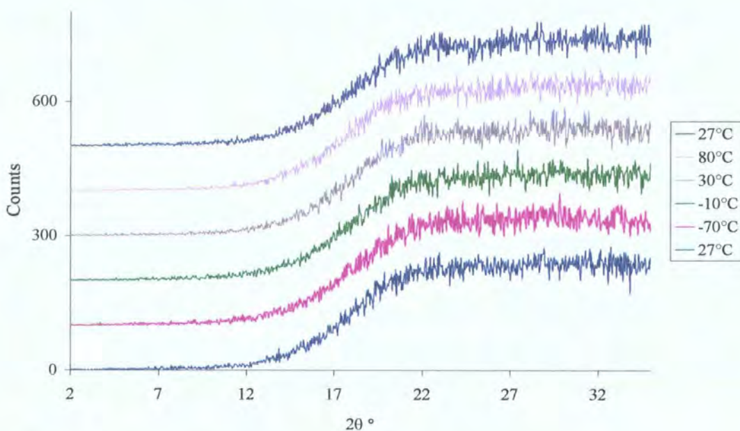
Figure 4.9: VT XRPD experiment of amorphous indomethacin.
