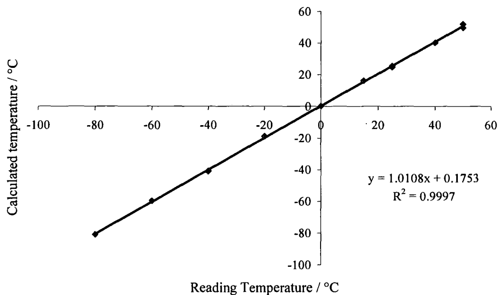
Figure 1: Reading versus calculated temperature plot of the VT calibration of the static probe, mounted with the 10 mm coil, on the CMX 200.
