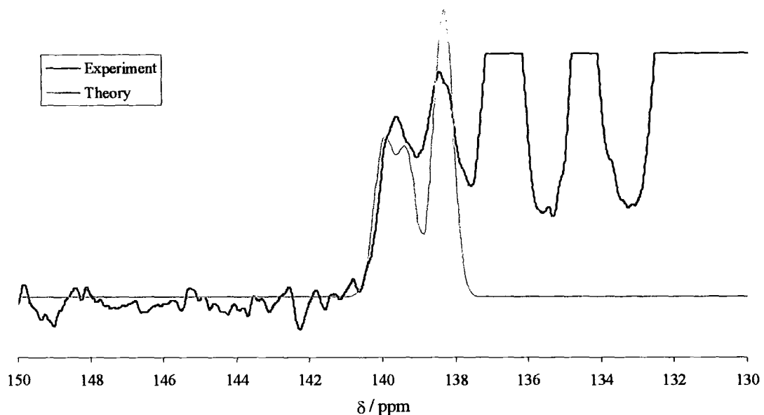
Appendix 16: Theory versus experimental for indomethacin, at 201.12 MHz, ^{13}\text{C} frequency, of C-14, J = -43 Hz and \chi = -63 MHz.
