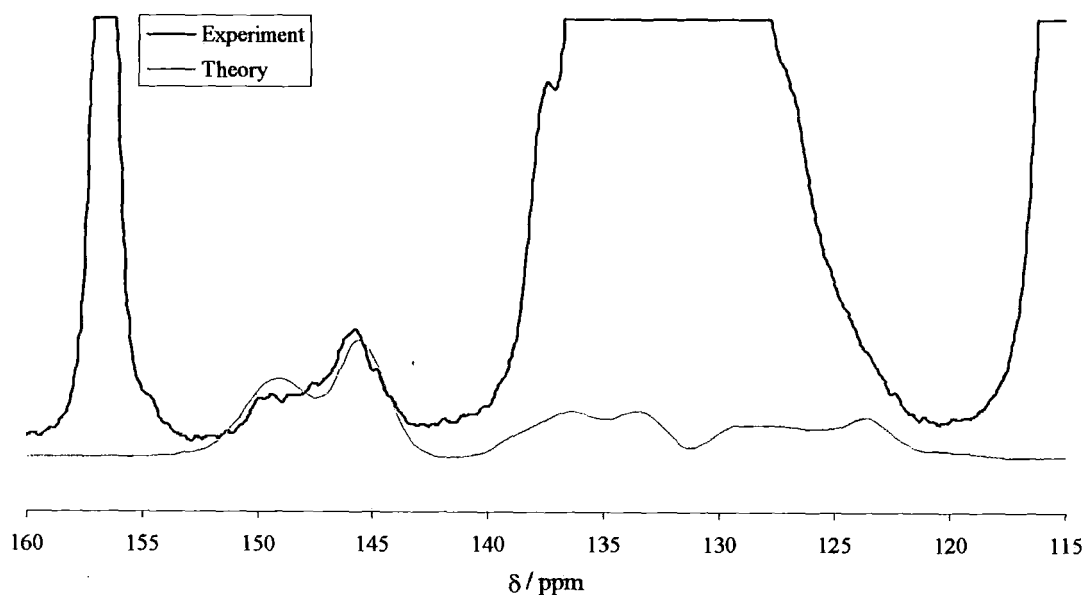
Appendix 13: Theory versus experimental for indomethacin, at 50.32 MHz, 13 C frequency, of C-14, J = -43 Hz and \chi = -63 MHz.
