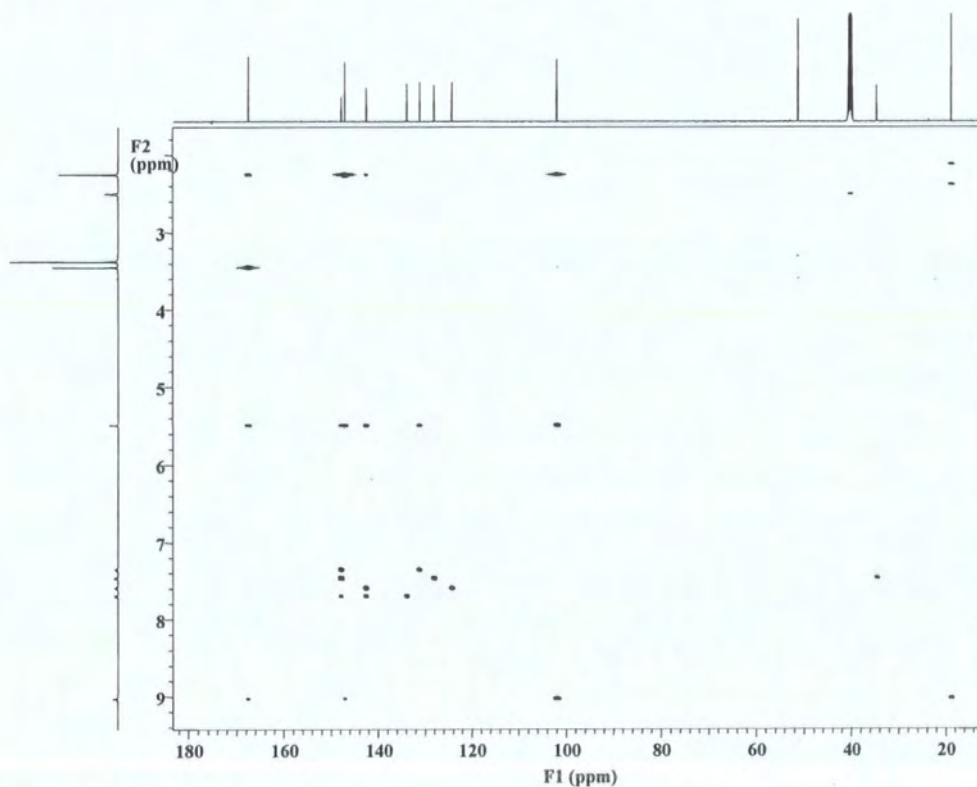
Appendix 7: HMBC spectrum of nifedipine, in d_6 -DMSO.
