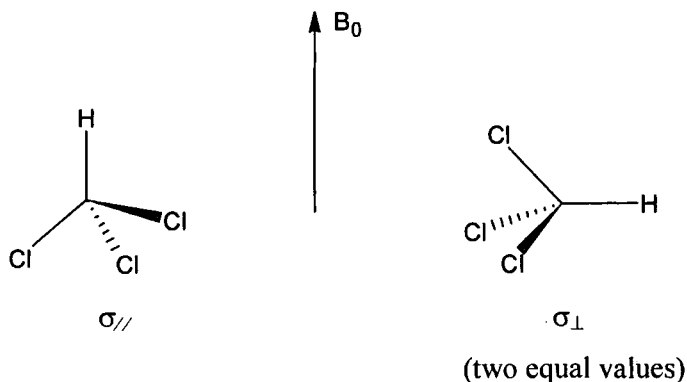
Figure 1.3: Axially symmetric case
