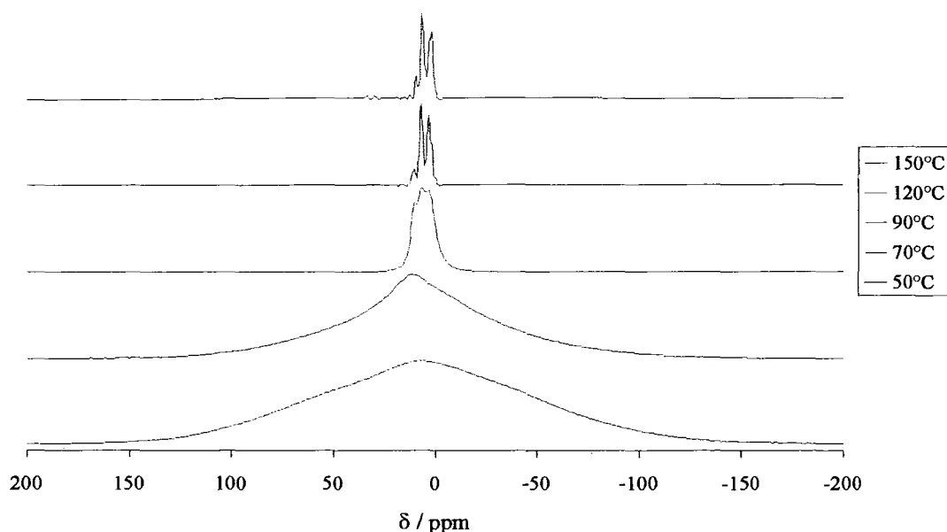
Figure 5.1: Static ^1\text{H} VT SSNMR spectra of amorphous indomethacin obtained by single-pulse-and-acquire at 200.13 MHz, ^1\text{H} frequency.
