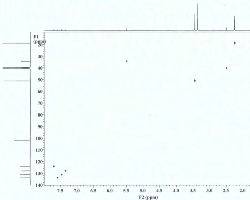
Appendix 6: HSQC spectrum of nifedipine, in d_6 -DMSO.
