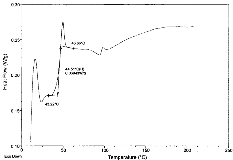
Figure 4.1: DSC of amorphous indomethacin showing Tg at 45°C.
