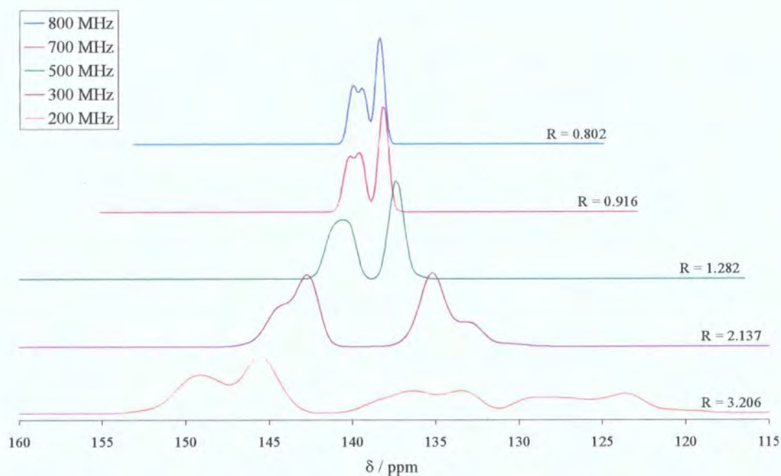
Figure 3.37: Theory at different magnetic fields, written as ^1\text{H} frequency, of C-14, J = -43 Hz and \chi = -63 MHz.
