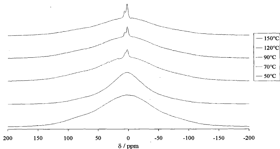
Figure 5.3: Static ^1\text{H} VT SSNMR spectra of amorphous nifedipine obtained by single-pulse-and-acquire at 200.13 MHz, ^1\text{H} frequency.
