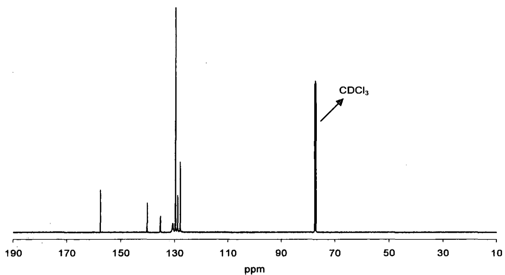
Figure 3.28: Carbamazepine carbon spectrum, in CDCl 3 .
