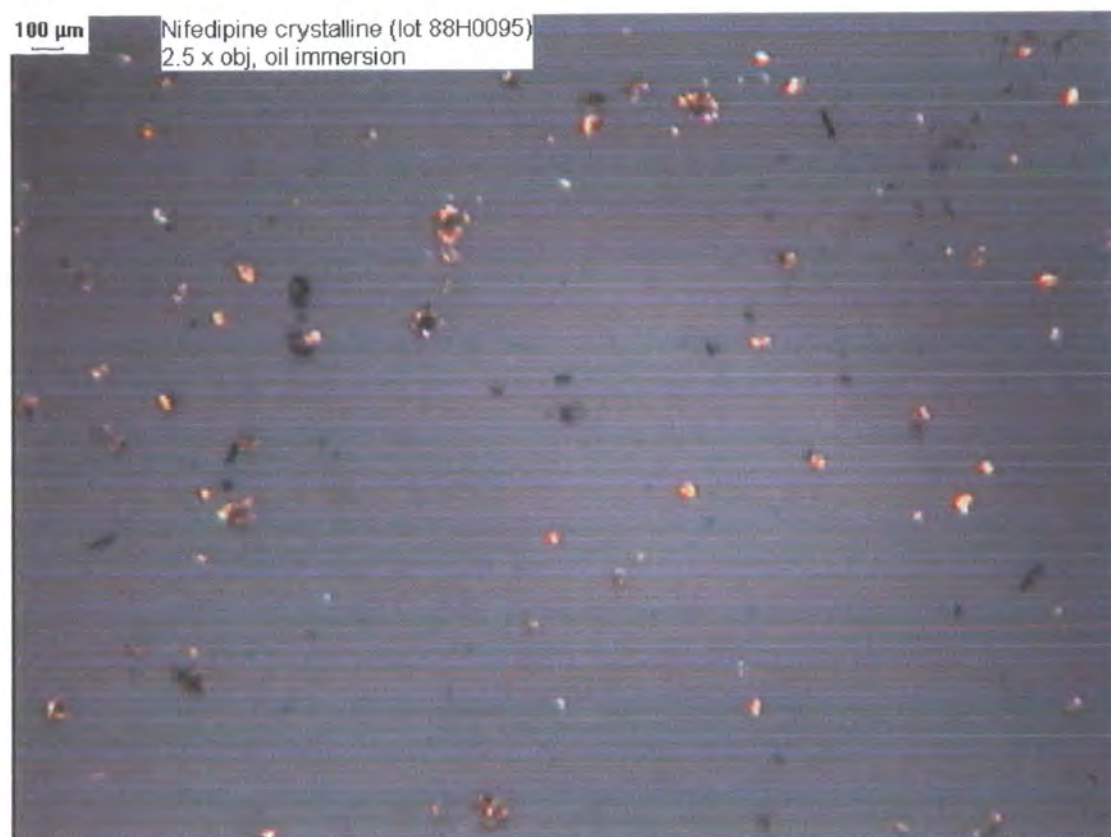
Figure 4.13: Polarised light microscopy snapshot of crystalline nifedipine showing birefringence.
