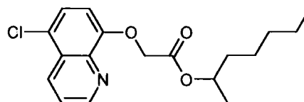
cloquintocet mexyl
