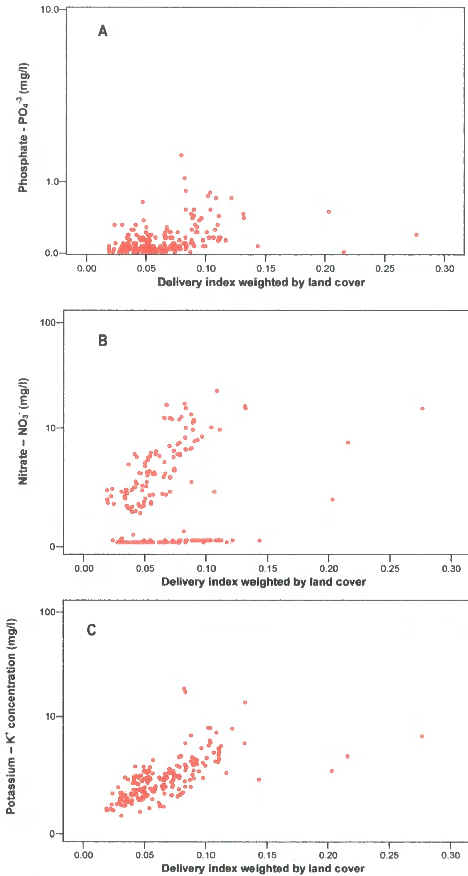
Figure 5.11: Scatterplots of nutrient concentration (mg/l) against delivery index weighted by land cover within the Eden catchment (a) phosphate ( PO_4^{3-} ), (b) nitrate ( NO_3^- ) and (c) potassium ( K^+ ).
