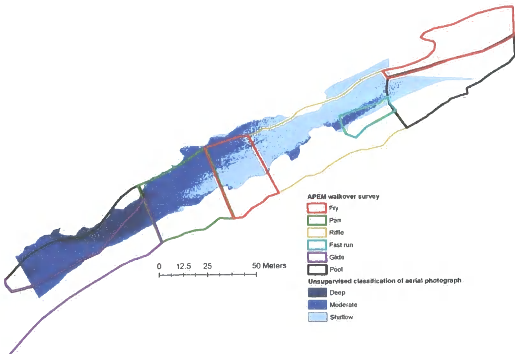
Figure 4.12: The relative depth composition (from aerial photography) of in-stream habitat types mapped during a walkover survey of the River Eamont by APEM Ltd. The data presented is for a 200m reach.
