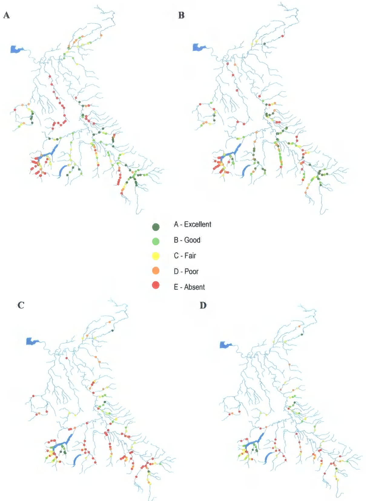
Figure 6.10: Sample sites used in the multivariate analysis. (a) salmon fry 2004; (b) salmon fry 2005; (c) trout fry 2004; and (d) trout fry 2005.
