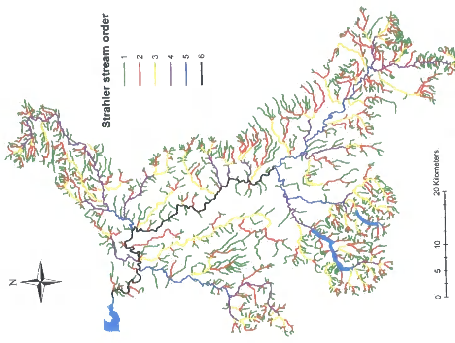
Figure 1.6(c) Strahler Stream Order (Source: Digitised from OS Raster 1:50,000 Environment Agency, 100026380 (2007)).
