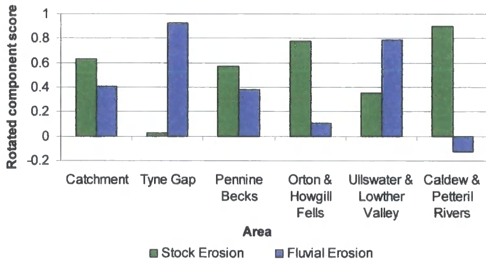
Figure 6.15: Relationship between bank erosion severity and the cause of erosion. Rotated component scores are presented for the PCA factor in each area which represents bank erosion severity.
