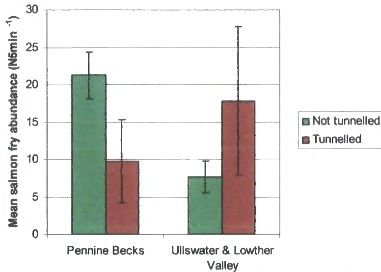
Figure 6.16: Area-scale variations in mean salmon fry abundance stratified by the presence/absence of tunnelled riparian vegetation. Standard error bars are shown.
