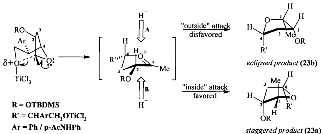
Scheme 64 – Explanation of the product stereochemistry according to the "inside attack" model
