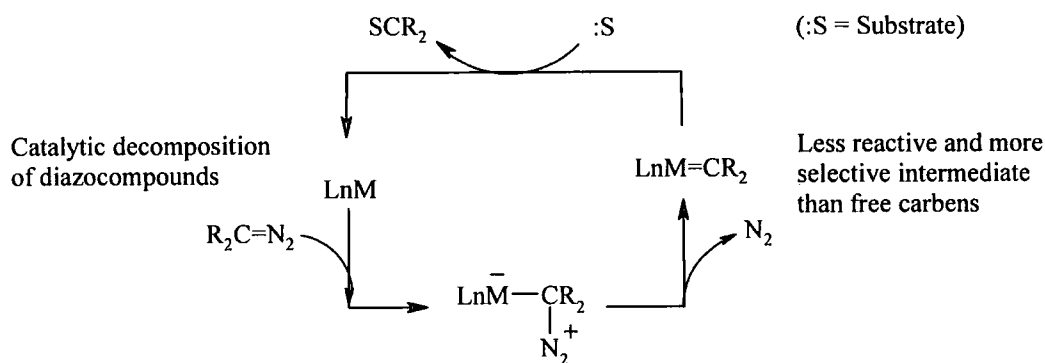
Scheme 13 – Reaction mechanism of metallocarbenes
