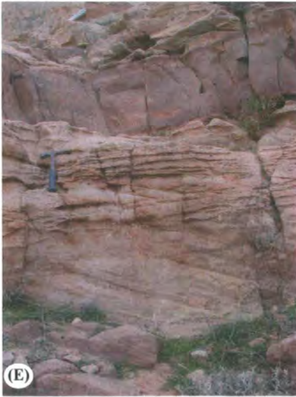
Large and small-scale of planar cross-stratification (Gsp).
