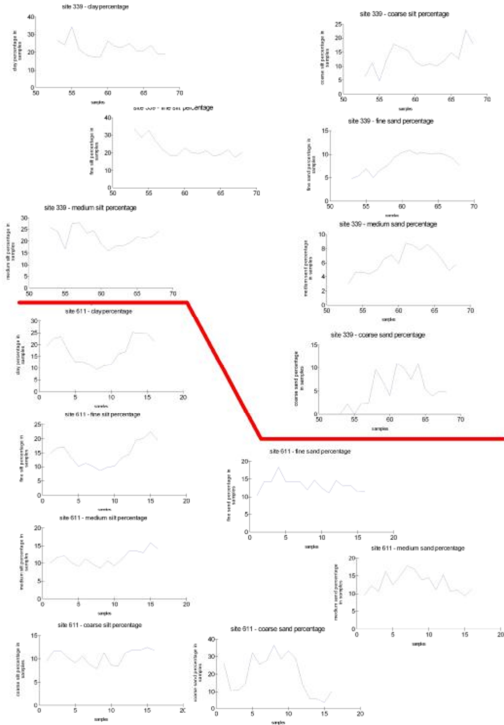
Figure 6-34 – Site 339 (Khirba Al-Tahisah) and transect 611 [Site 279 (Khirbet Al-Qatiyya)] granulometry graphs. Soil samples 53-68 and 1-16 respectively.
