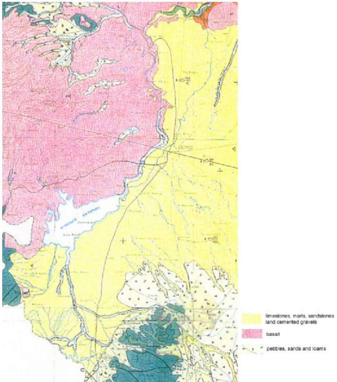
Figure 5-3 – Part of geological map covering the area of interest. The map is dated 1964, and the scale is 1:200,000 (Ponikarov et al. , 1963).
