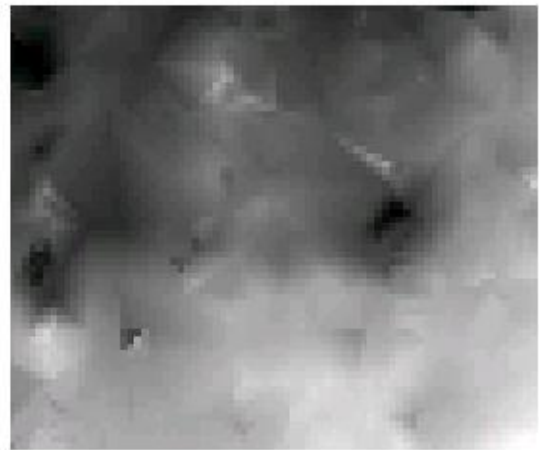
CORONA DEM, scaled values minimum=560, maximum=590
