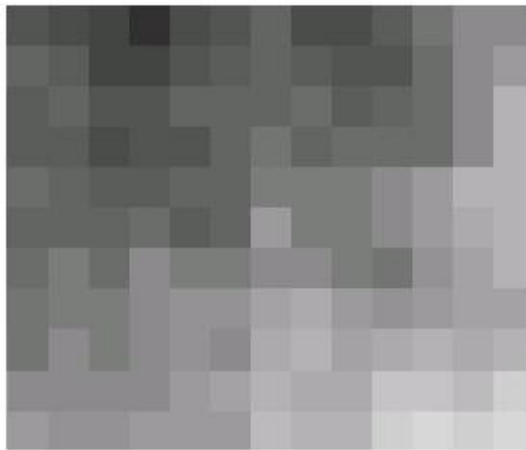
SRTM-3 DEM, scaled values minimum=560, maximum=590
