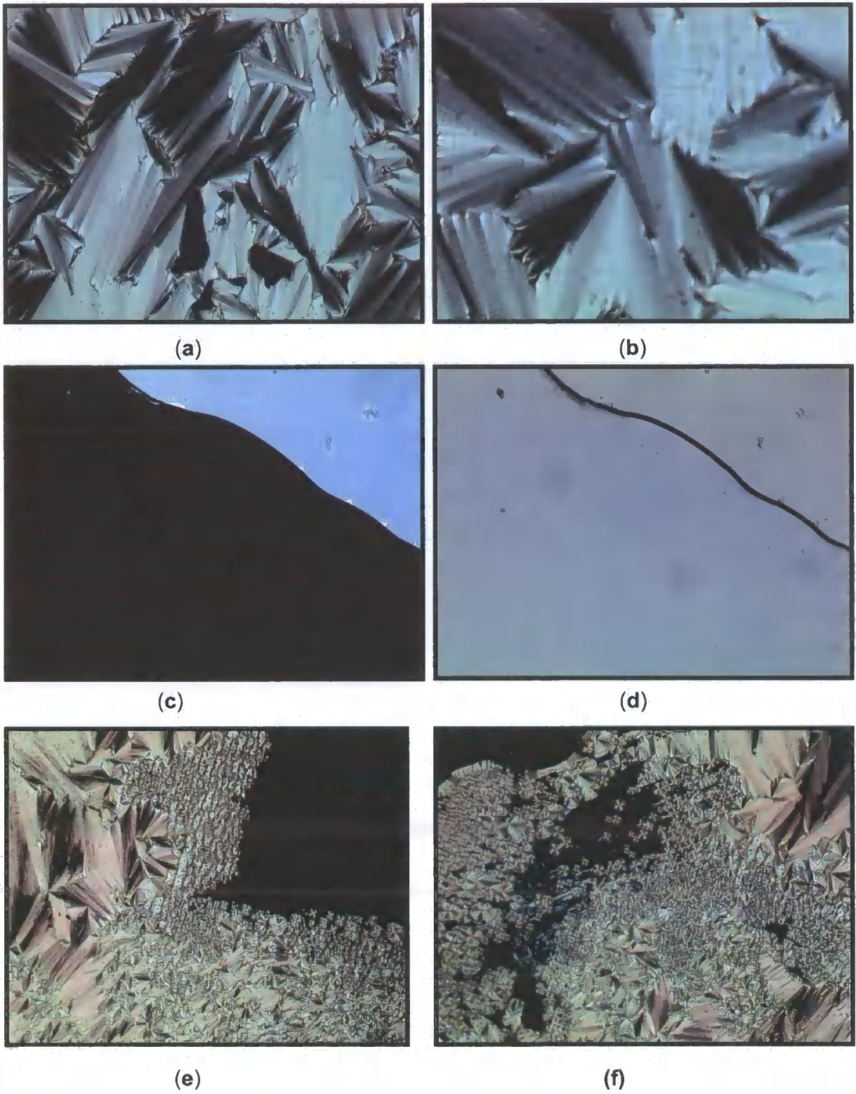
Figure 3.4: The different optical textures associated with the smectic A phase of (a) 7c (b) 7c (c) 7d (d) 7d (e) 11c.(f) 11c
