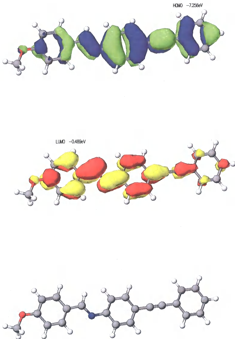
Figure 2.2: Graphical representation of the HOMO and LUMO orbitals, together with the optimised molecular structure of compound 4-OMe (courtesy of Dr A. Beeby, Department of Chemistry, University of Durham).
