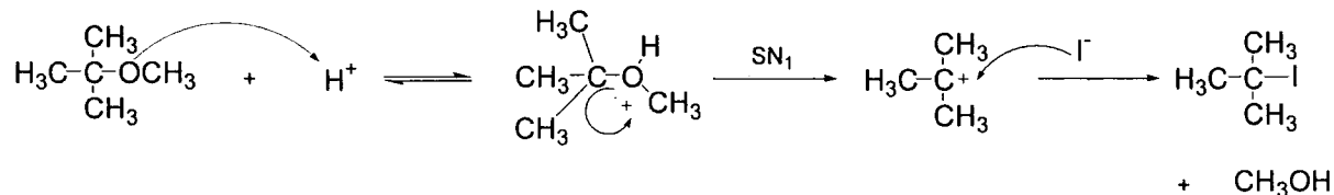
Scheme 1.24: The mechanism of ether cleavage by the protonation of ether oxygen as an initial step.
