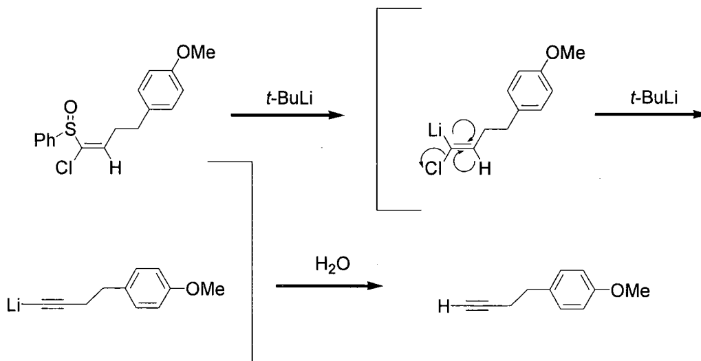
Scheme 1.11: The examples of Fritsch-Buttenberg-Wiechell rearrangement. 41
