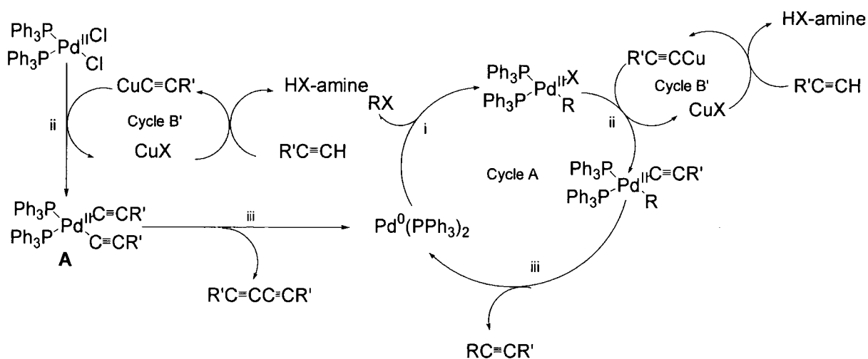
Scheme 1.13: Pd-catalysed cross-coupling reaction of terminal acetylene mechanism involving steps of i) oxidative addition, ii) transmetalation and iii) reductive elimination. 43
