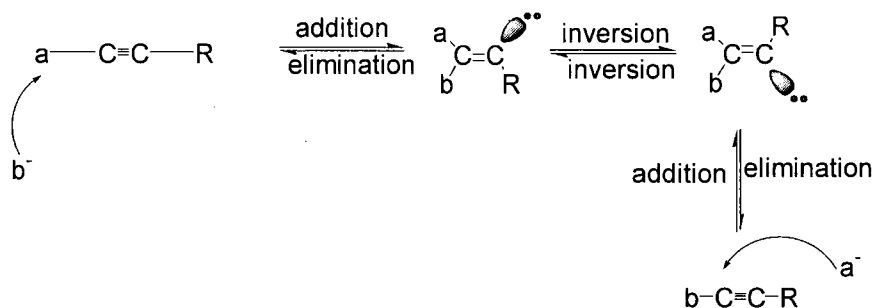
Scheme 1.8: The reversible mechanism of substitution formation of alkyne.
