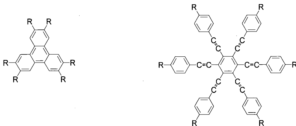
Figure 3.2: The examples of discotic mesogens 32
