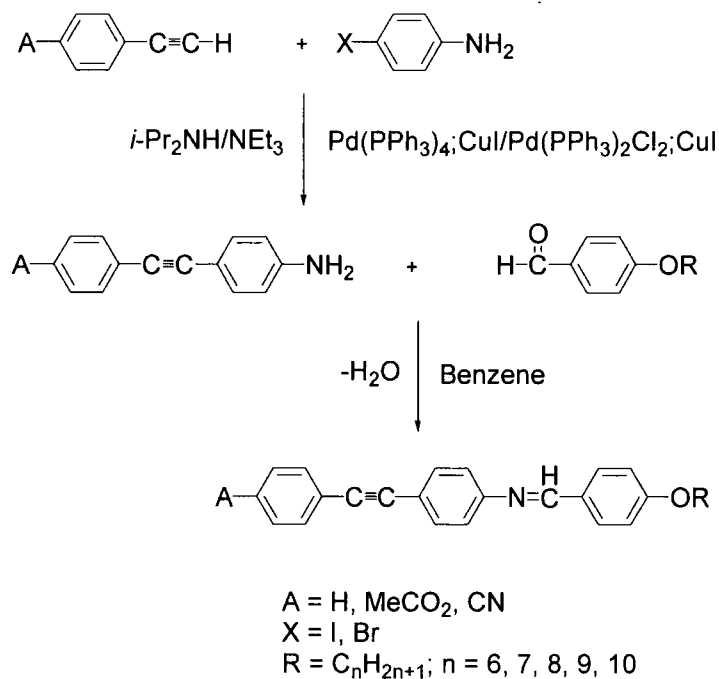
Scheme 2.1: Synthetic approach adopted in this thesis.
