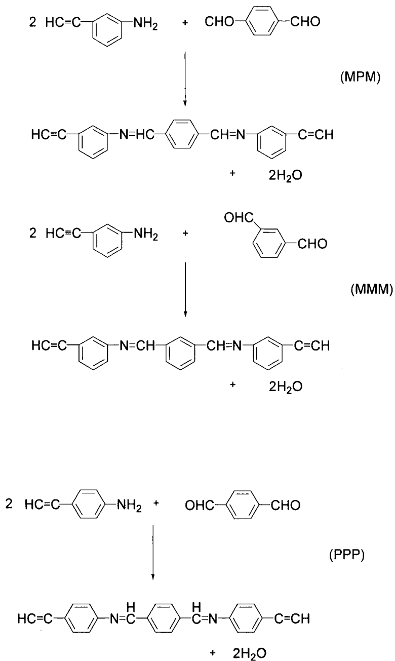
Scheme 1.1: The condensation of 1,3- or 1,4-phthalaldehyde with 3- or 4-aminophenylacetylene gave the meta-meta-meta (MMM), meta-para-meta (MPM) or para-para-para (PPP) monomers. 29
