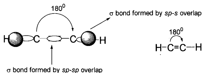
Figure 1.4: Alkyne is a linear molecule with bond angles of close to 180^\circ .
