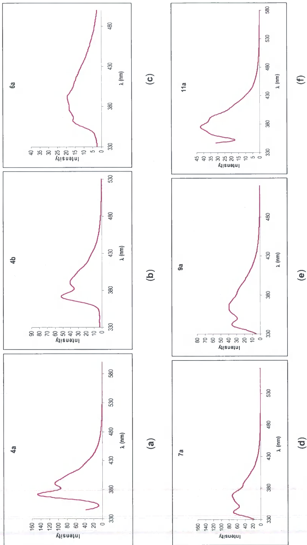
Figure 2.4: The emission spectra for selected compounds in each series recorded in cyclohexane at 298 K.
