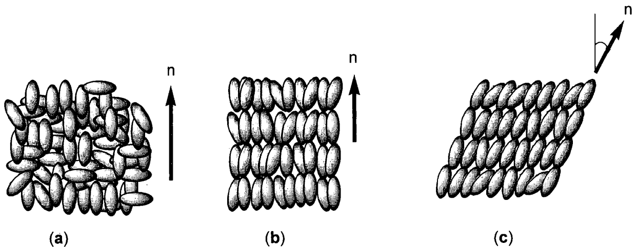
Figure 3.3: Generalized structure (a) nematic, (b) smectic A (c) smectic C.
