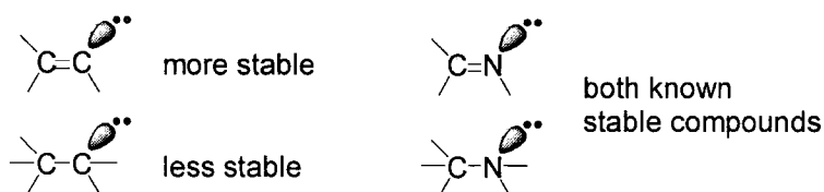
Figure 1.5: The analogous isoelectronic nitrogen derivatives of unsaturated carbon compounds.
