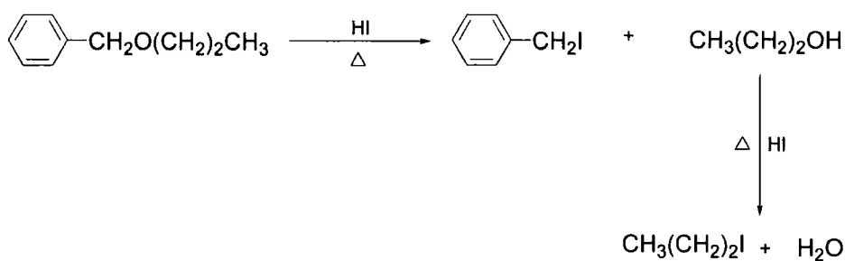
Scheme 1.26: The \text{S}_{\text{N}}2 cleavage reactions would react with HBr or HI to form the substitution product.
