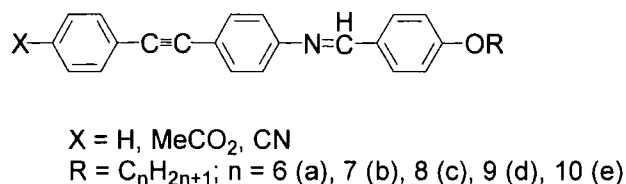
Figure 1.3: Proposed ethynylated Schiff-Base aromatic systems.
