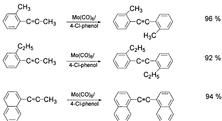
Scheme 1.20: The reaction conditions of alkyne metathesis utilizing \text{Mo(CO)}_6 and 4-chlorophenol by increasing the reaction temperature producing more than 90 % yields. 19
