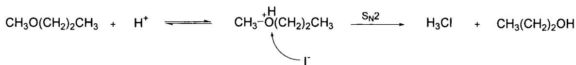
Scheme 1.25: The displacement of \text{S}_{\text{N}}1 by \text{S}_{\text{N}}2 in the ether cleavage.
