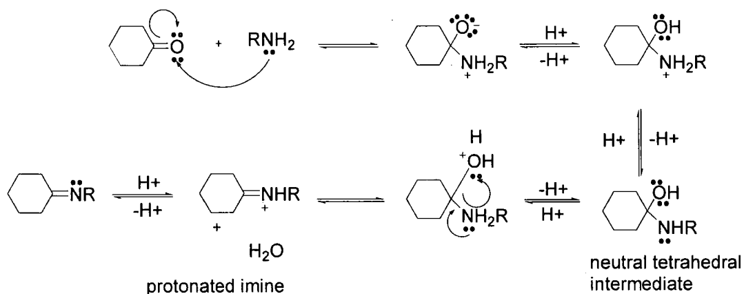
Scheme 1.4 : The mechanism of imine formation.
