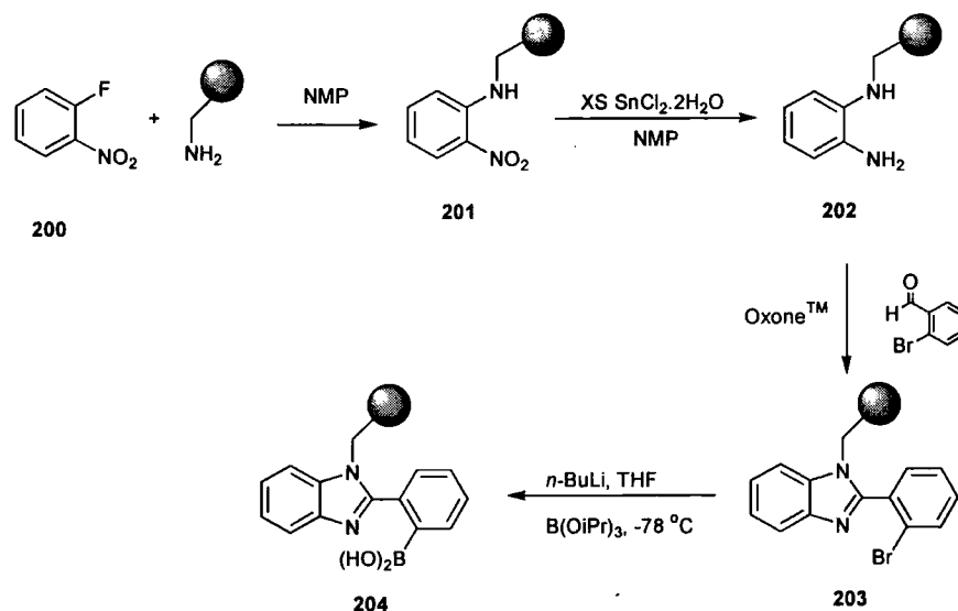
Scheme 34
