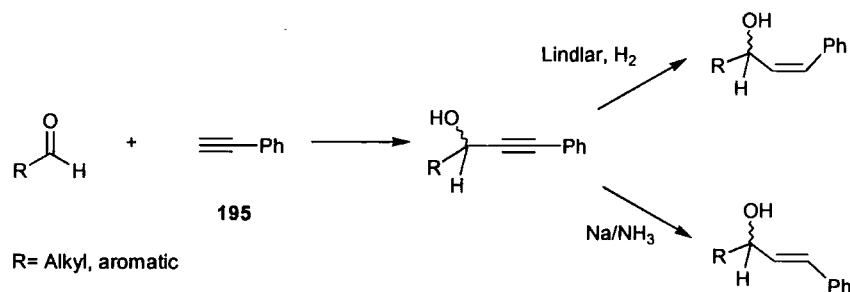
Scheme 33
