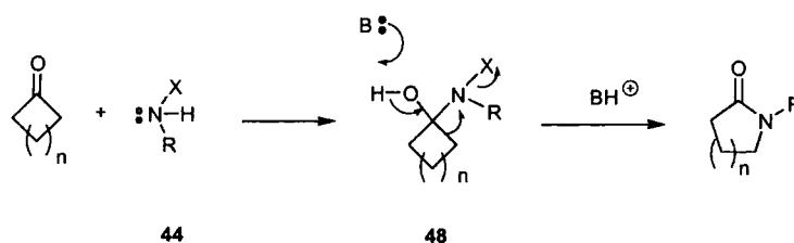
Scheme 9
