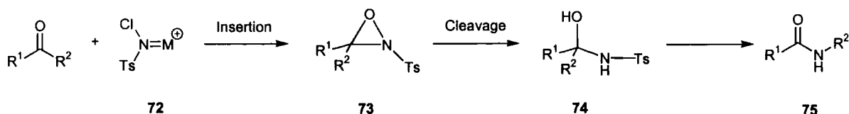
Scheme 14
