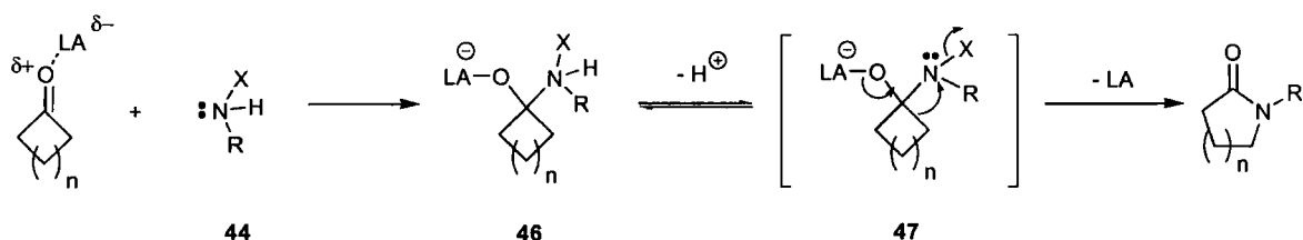
Scheme 8
