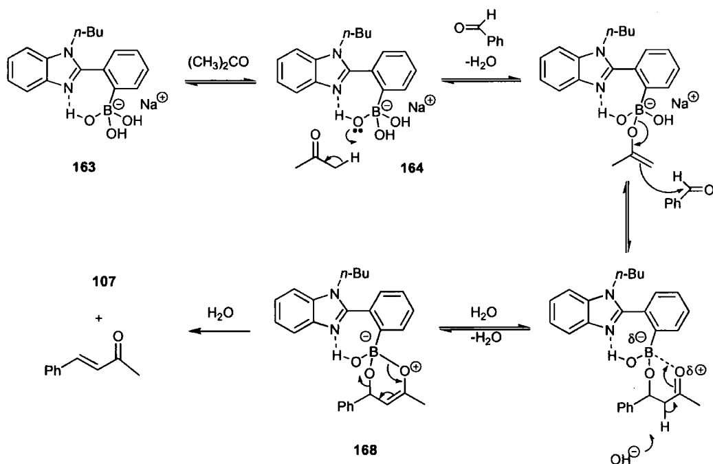
Scheme 31
