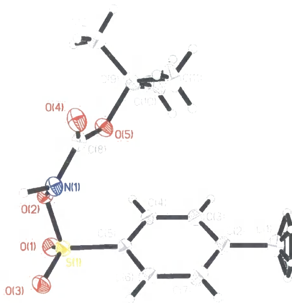
Figure 3: 50% probability thermal ellipsoid plot of 61
