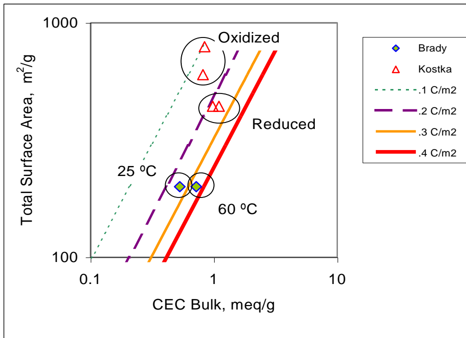
Figure 5.3 – Effect of iron reduction and temperature effects on surface charge. Brady (1992) measured CEC and SSA on one \text{SiO}_2 sample at two temperatures (diamonds). Surface charge at 60 °C increased to about 0.35 \text{ C/m}^2 . Kostka et al. (1999) measured CEC and SSA on two smectite samples (triangles) before and after reduction of iron. Surface charge increased sharply.
