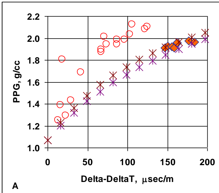
Figure 5.9: \Delta\Delta T ( 10^6/V - 10^6/V_n ) versus pore pressure gradient (PPG) from Hottman and Johnson (1965). Diamonds are data from Well A. Crosses represent the expected relationship for Well A, assuming constant effective stress along line A-B in Figure 5.7 in accordance with an equivalent depth model. The top set of crosses assumes a mean-stress model and bottom set assumes a (standard) vertical-stress model. More details will be given later on the method for determining the predicted values.
