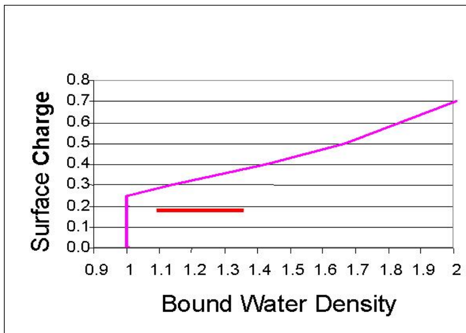
Figure 5.4: The dielectric saturation effect (from Danielewicz-Ferchmin and Ferchmin, 1996). The red horizontal is the average surface charge for soils. Surface charge is expressed in \text{C/m}^2 and bound water density is expressed in \text{g/cc} .
