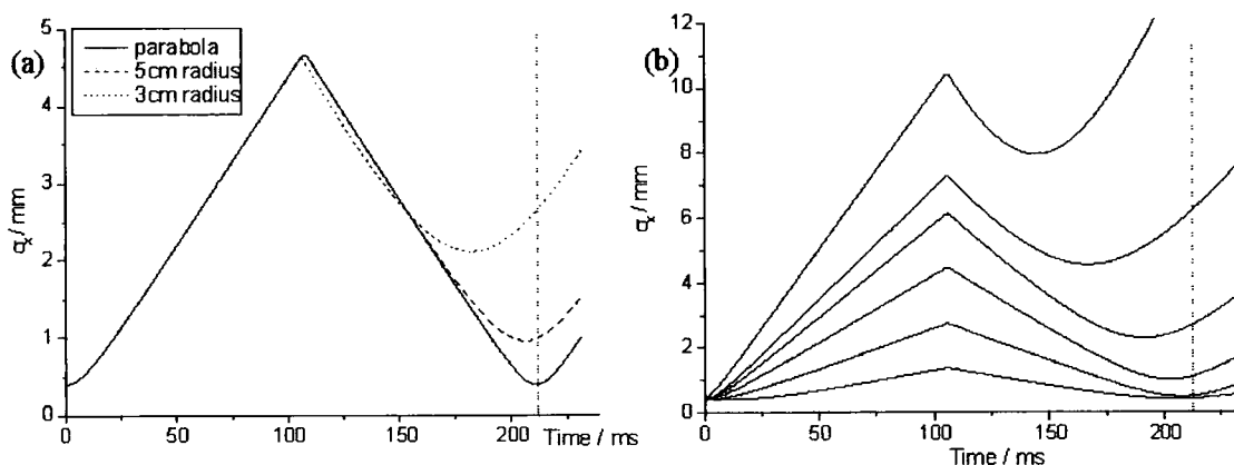
Figure 4.2. (a) Simulation of 500 atoms going through a 10 000 Amp-turn strategy I lens. The solid, dashed and dotted lines correspond to a parabolic approximation lens, a 5 cm radius lens, and a 3 cm radius lens, respectively. The duration and timing of the impulse is chosen using the \mathcal{ABCD} matrix formalism, bringing the atoms to a focus 22 cm above their launch height. (b) A shell plot of 1000 simulated atoms passing through a 3 cm radius strategy I lens. The distances from the coil centre are 0–10% of the coil radius, 10–20%, through to 50–60%. Atoms further from the centre are not focussed as well, and the focusing occurs at earlier times. Both of these factors degrade the image quality and size.
