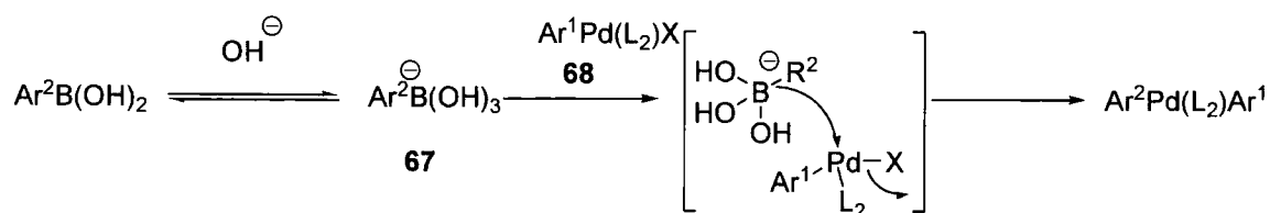
Scheme 1.2d: Transmetallation step.
