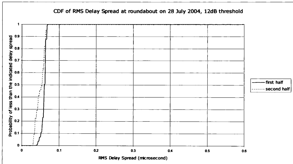
Figure 8.65 CDF of RMS Delay Spread at the roundabout on 28 July 2004 with a 12 dB threshold.
