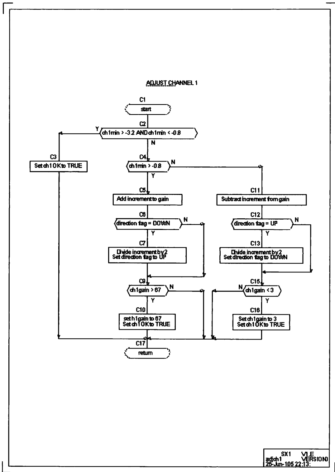
Figure 7.6. Logic of the channel gain adjustment routine.
