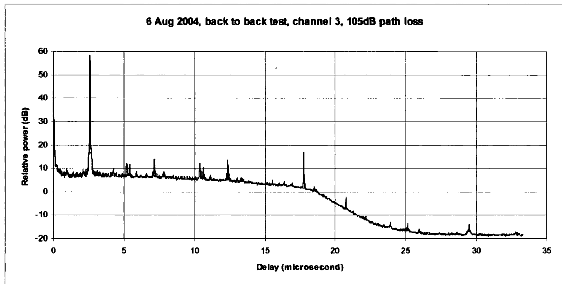
Figure 5.6 Result from back to back test on 6 August 2004 for channel 3.
