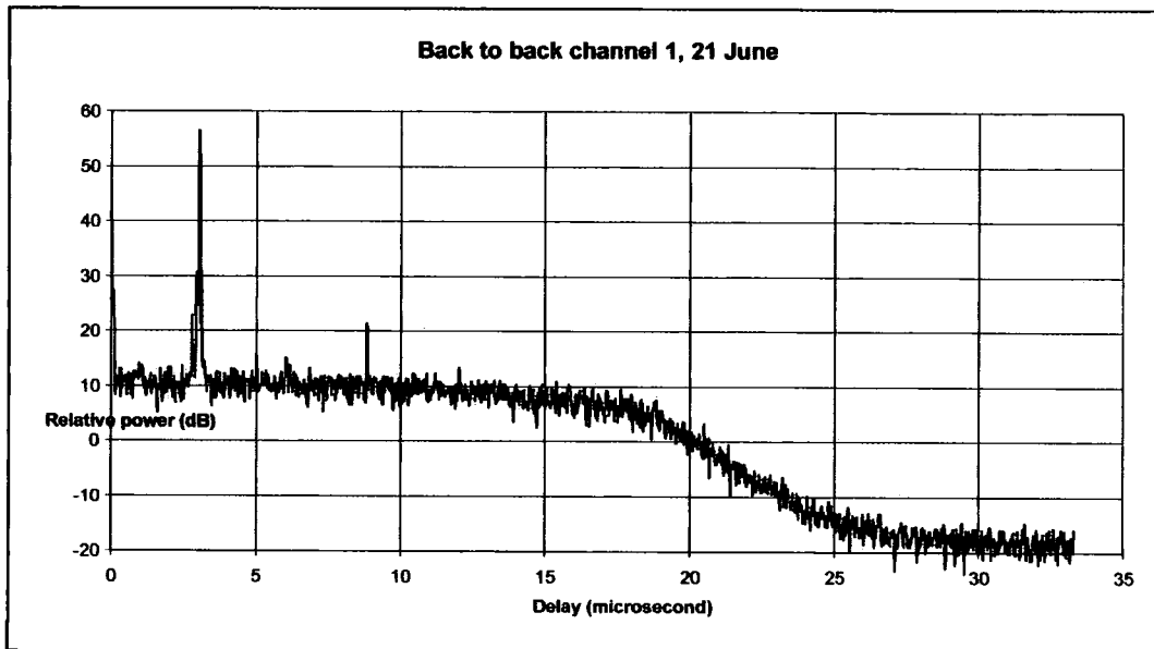
Figure 5. Back to back delay profile with roofing filter.
