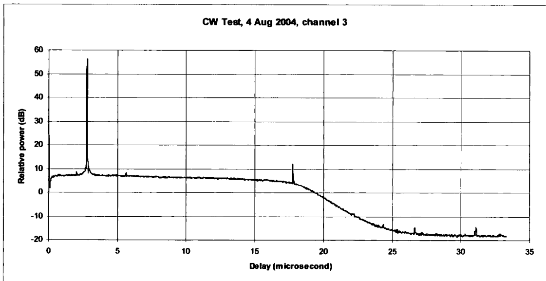
Figure 5.2 Result of typical CW Test, complete spectrum
