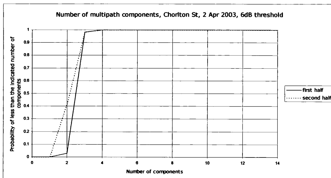
Figure 8.25 CDF of the number of multipath components at Chorlton Street car park, Manchester on 2 April 2003 with a 6 dB threshold.
