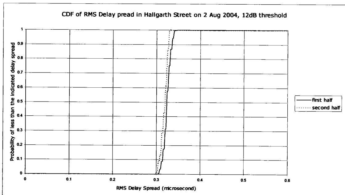
Figure 8.67 CDF of RMS Delay Spread in Hallgarth Street on 2 August 2004 with a 12 dB threshold.
