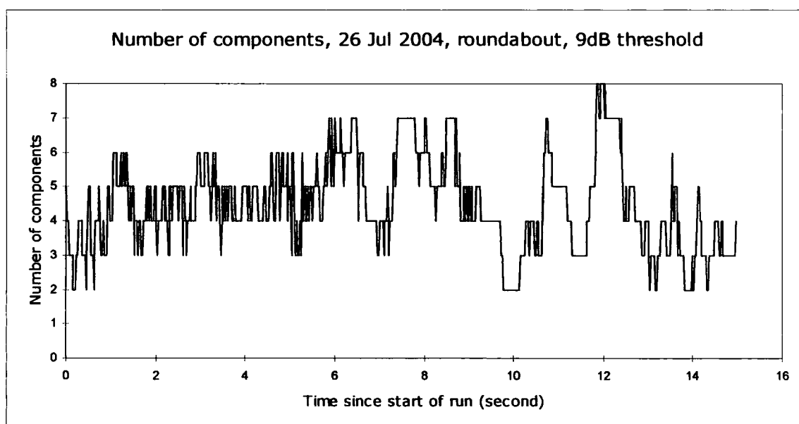
Figure 8.5 Variation in the number of components with a 9 dB threshold by the roundabout in Durham on 26 July 2004
