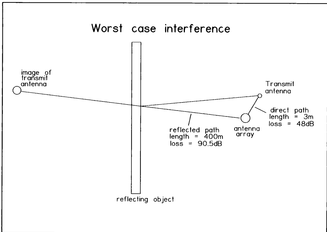
Figure 6.5. Worst case interference
