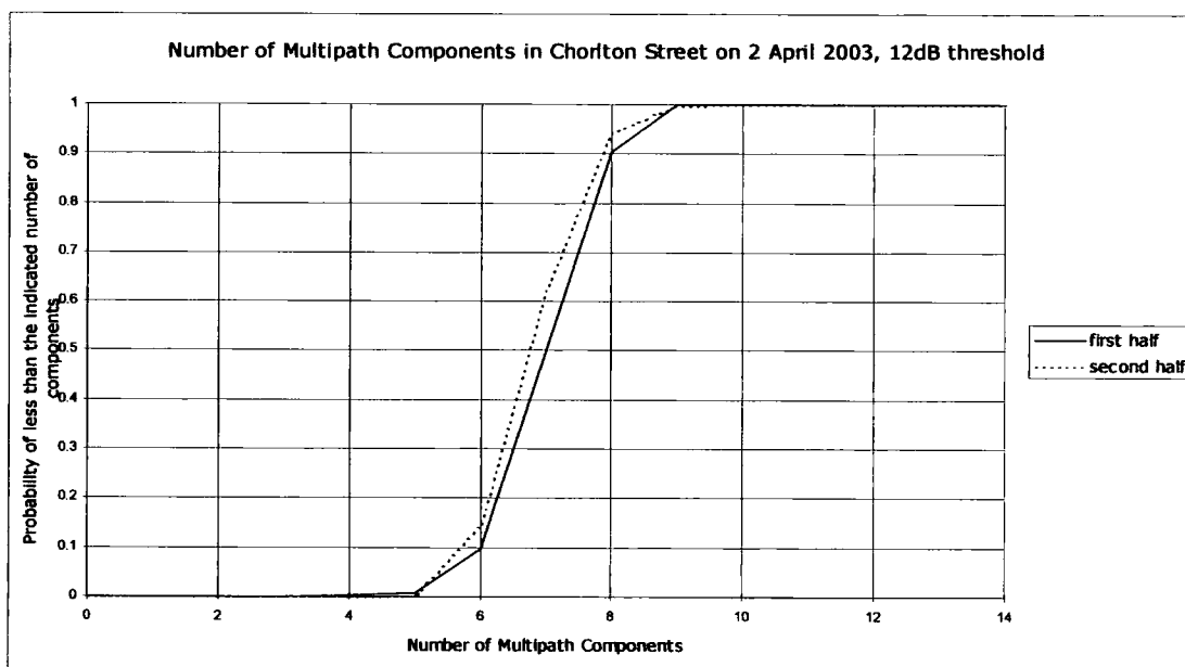
Figure 8.26 CDF of the Number of Multipath Components at Chorlton Street car park, Manchester on 2 April 2003 with a 12 dB threshold.
