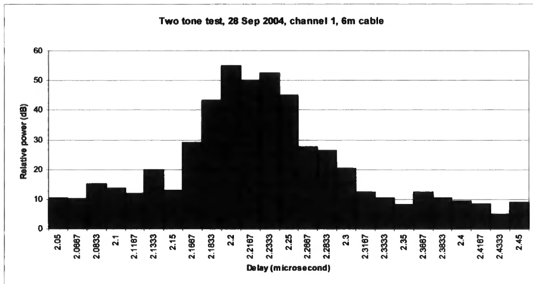
Figure 5.16. Results from two tone back to back test with 6 m cable.
