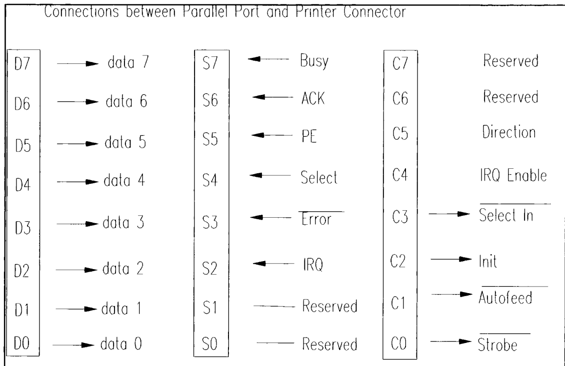
Figure 2. Connections between Parallel Port Registers and Printer Connector.
