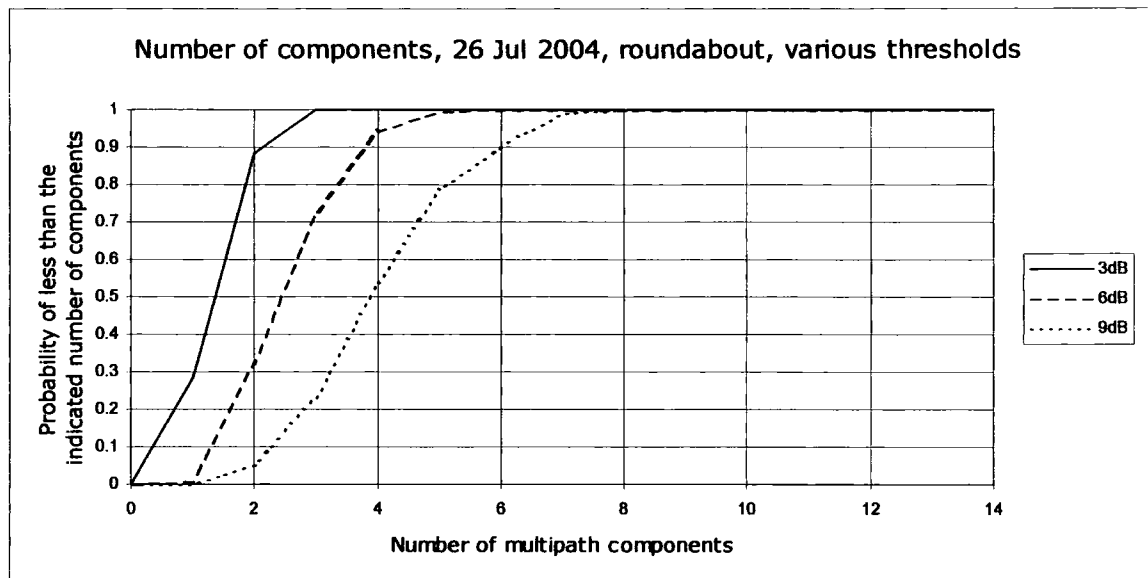
Figure 8.6. CDF of the number of components by the roundabout in Durham with various thresholds.
