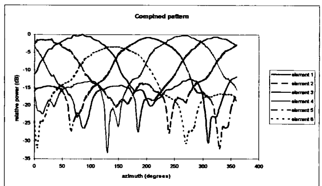
Figure 2. Combined radiation pattern of 6 element array.
