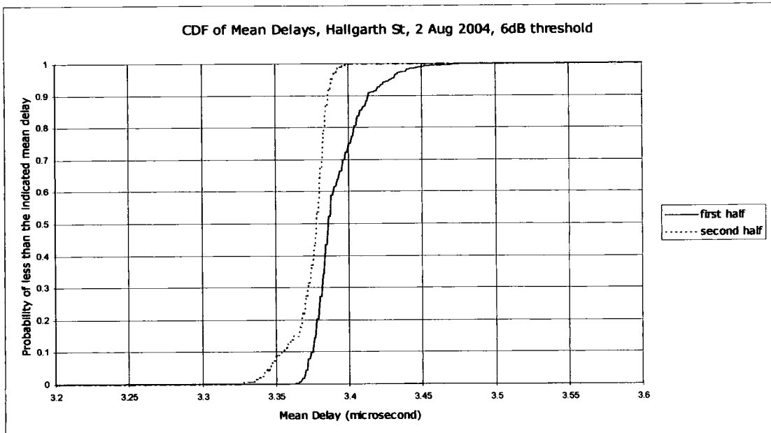
Figure 8.46 CDF of mean delays in Hallgarth Street on 2 August 2004 with a 6 dB threshold.
