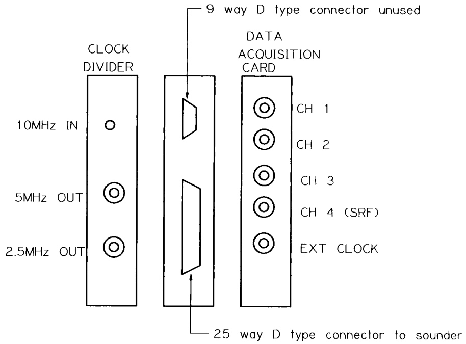
Figure 7.7. Data Acquisition card and Associated Connectors
