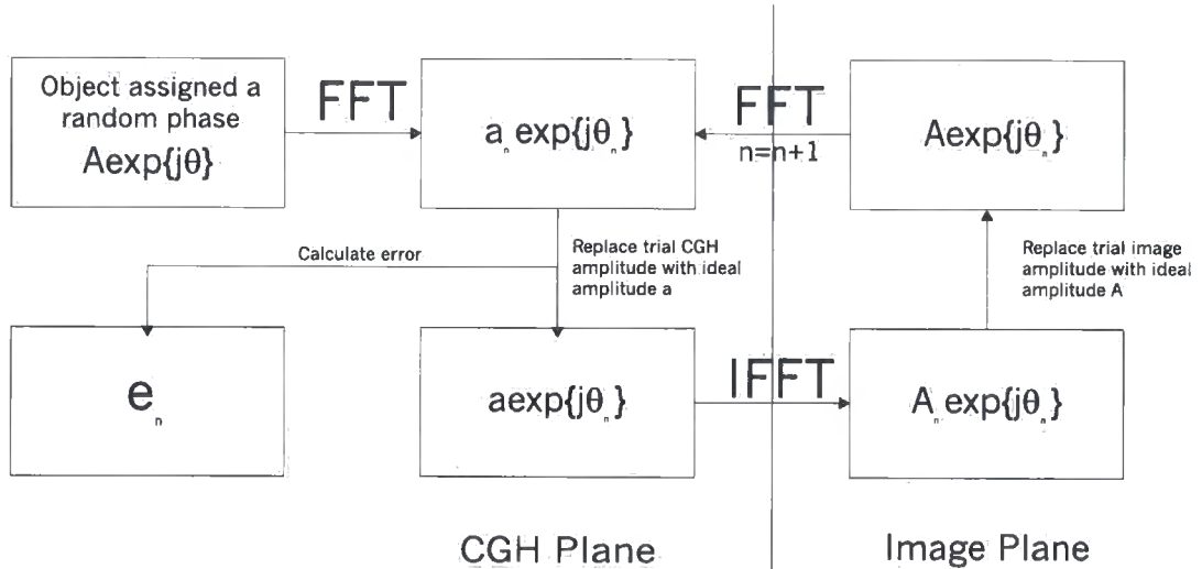
Figure 3.5: Operation of the Gerchberg-Saxton Algorithm
