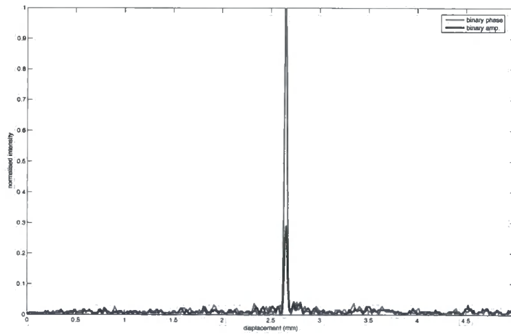
Figure 6.8: The line segment cross-sections that result from the binary masks
