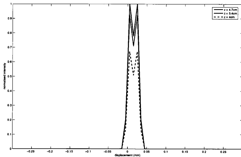
Figure 8.13: Plots across the line image of figure 8.11
