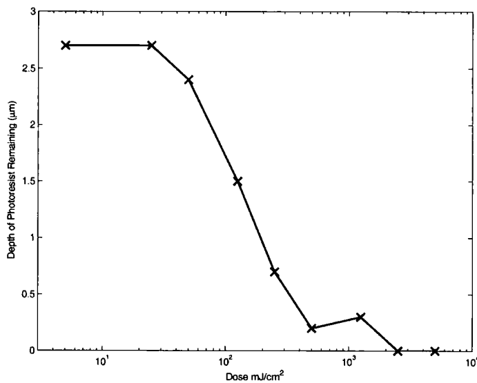
Figure 10.4: The Dill curve for PEPR
