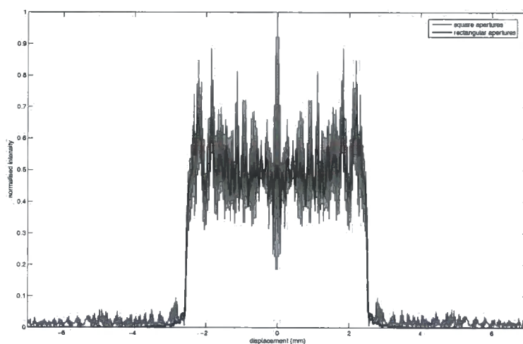
Figure 6.18: Comparison between the profiles along the rectangle image formed using square and rectangular apertures in the CGH
