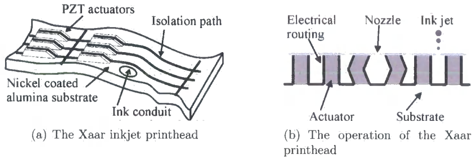
Figure 10.1: Structure and operation of the Xaar printhead
