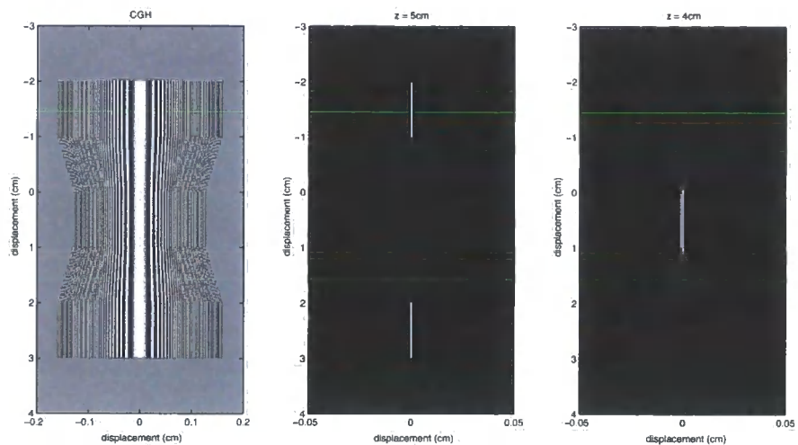
Figure 8.6: A CGH consisting of several sloped line segments and the image it produces
