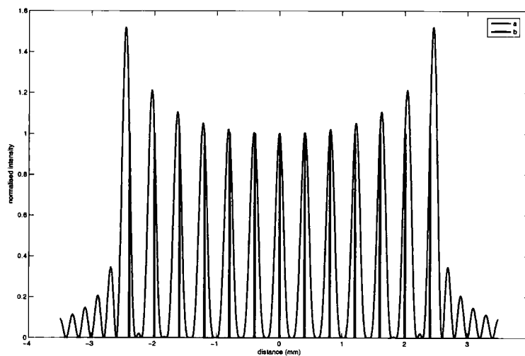
Figure 7.5: (a); the intensity across 13 parallel line segment images separated by 2x the Rayleigh criterion. (b); the locations of the centres of each line segment CGH pattern
