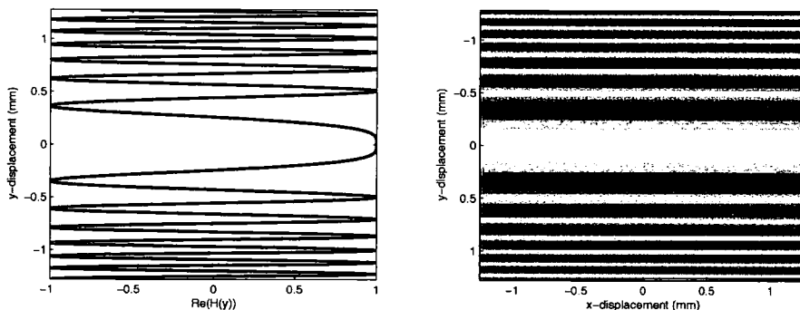
Figure 5.2: A typical phase angle profile for equation 5.3
