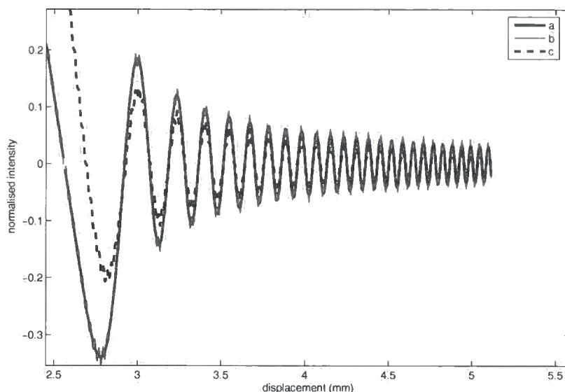
Figure 5.12: Approximations to the FDF for large +x . a; C(a_2) , b; C(a_2) - C(a_1) , c; Real(FDF_R(x))
